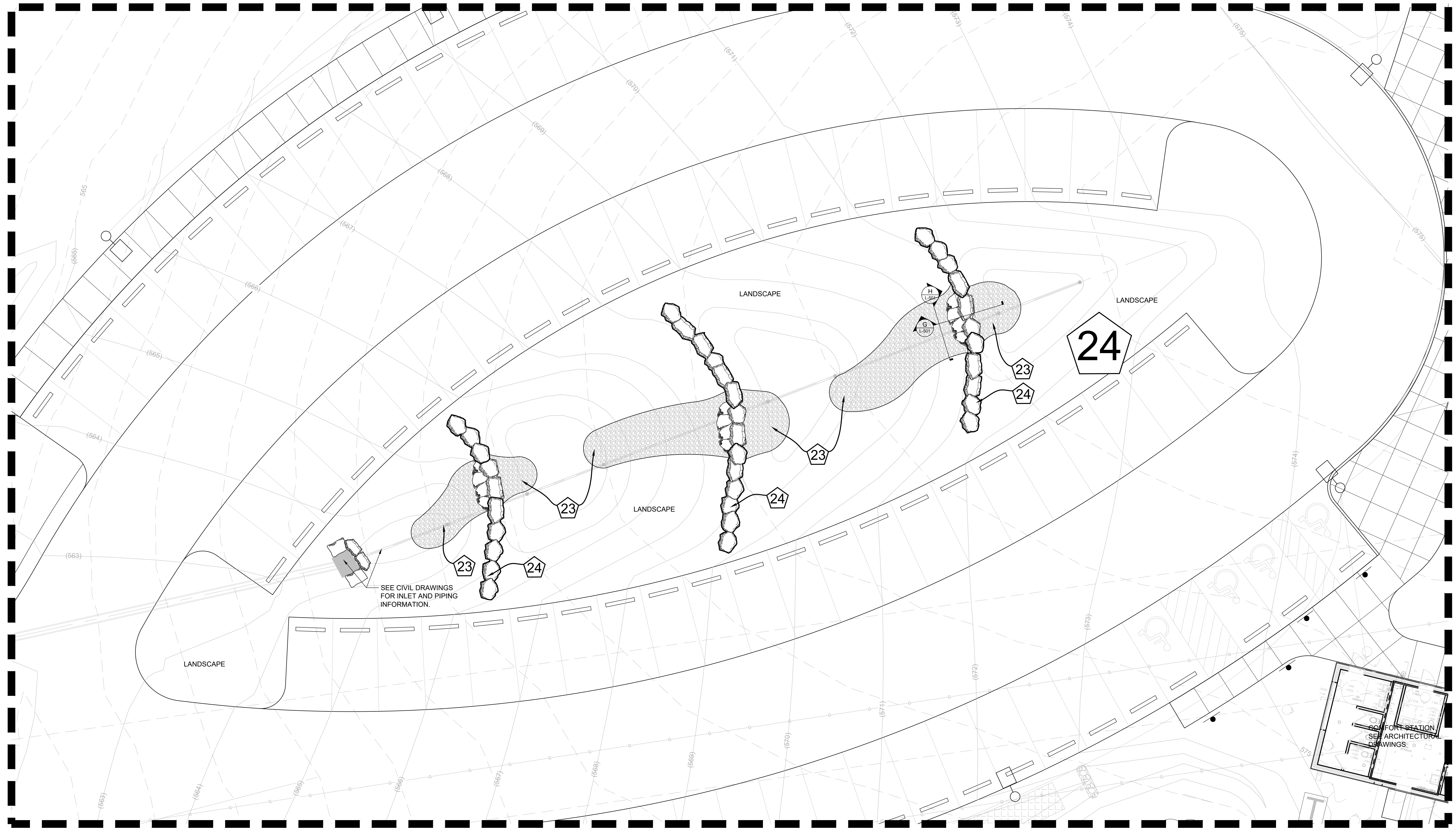
A RAIN GARDEN ENLARGEMENT PLAN SCALE: 1"=10'
