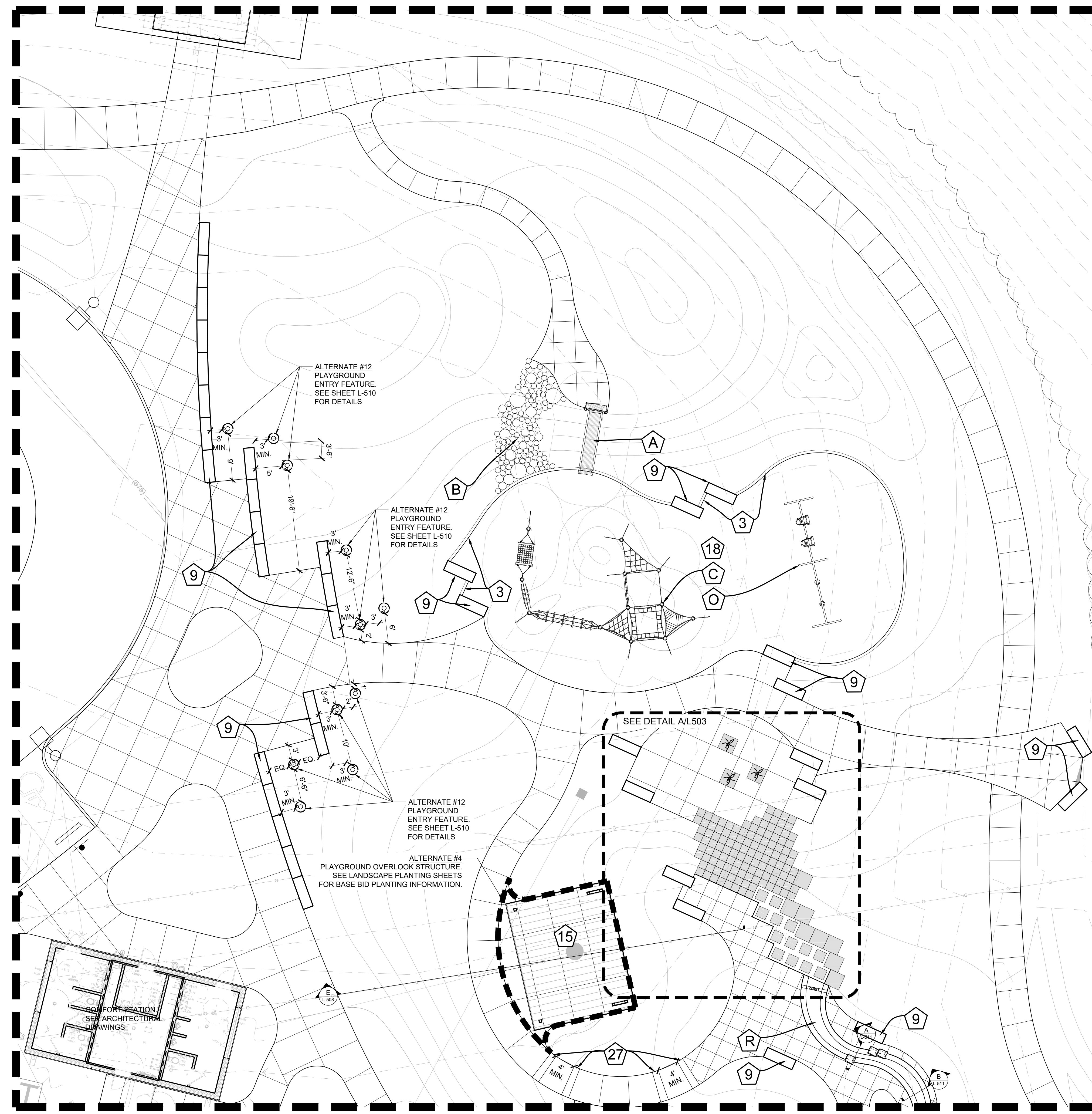
A PLAYGROUND ENLARGEMENT PLAN SCALE: 1"=10'
