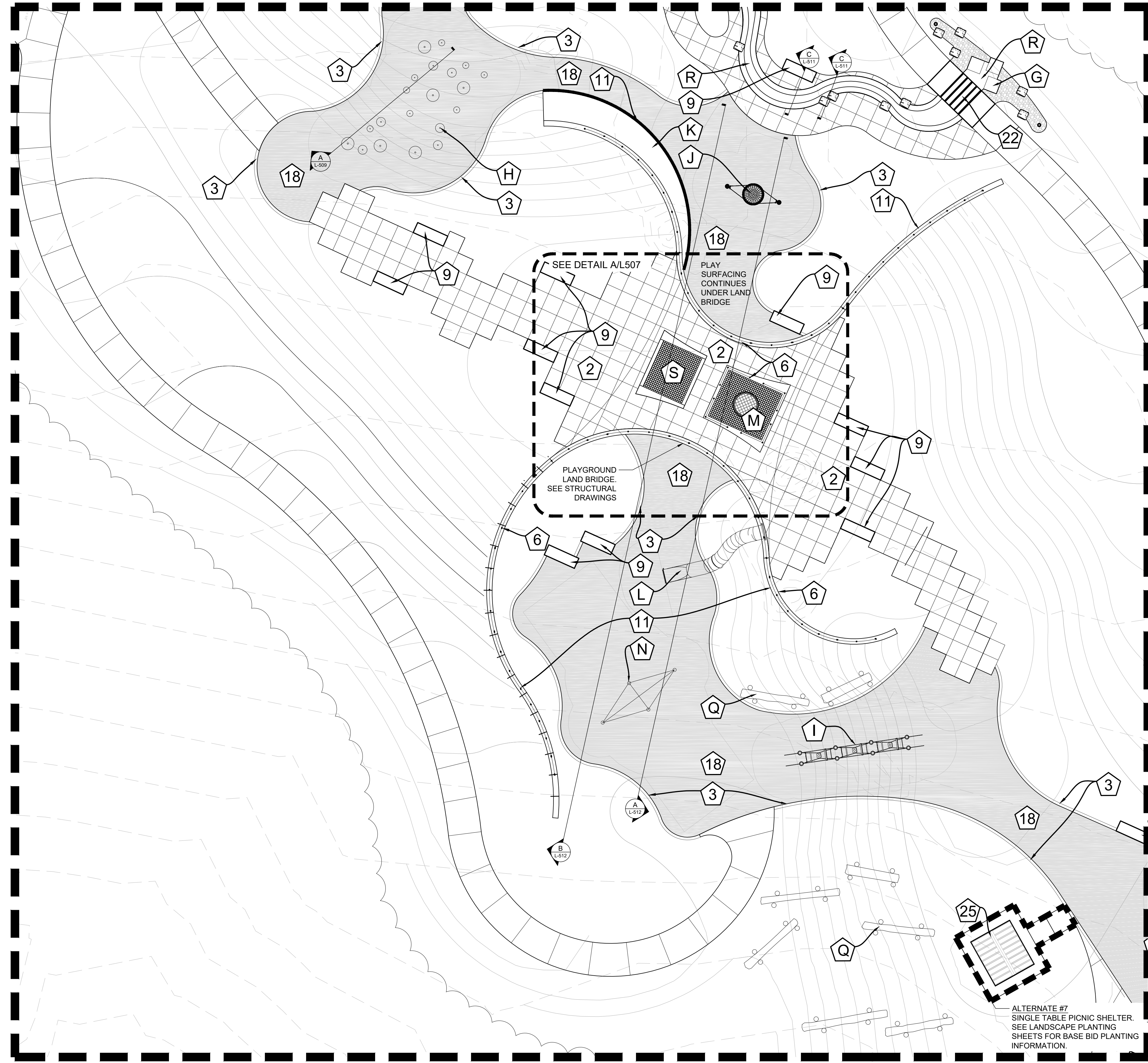
A PLAYGROUND ENLARGEMENT PLAN SCALE: 1"=10'
