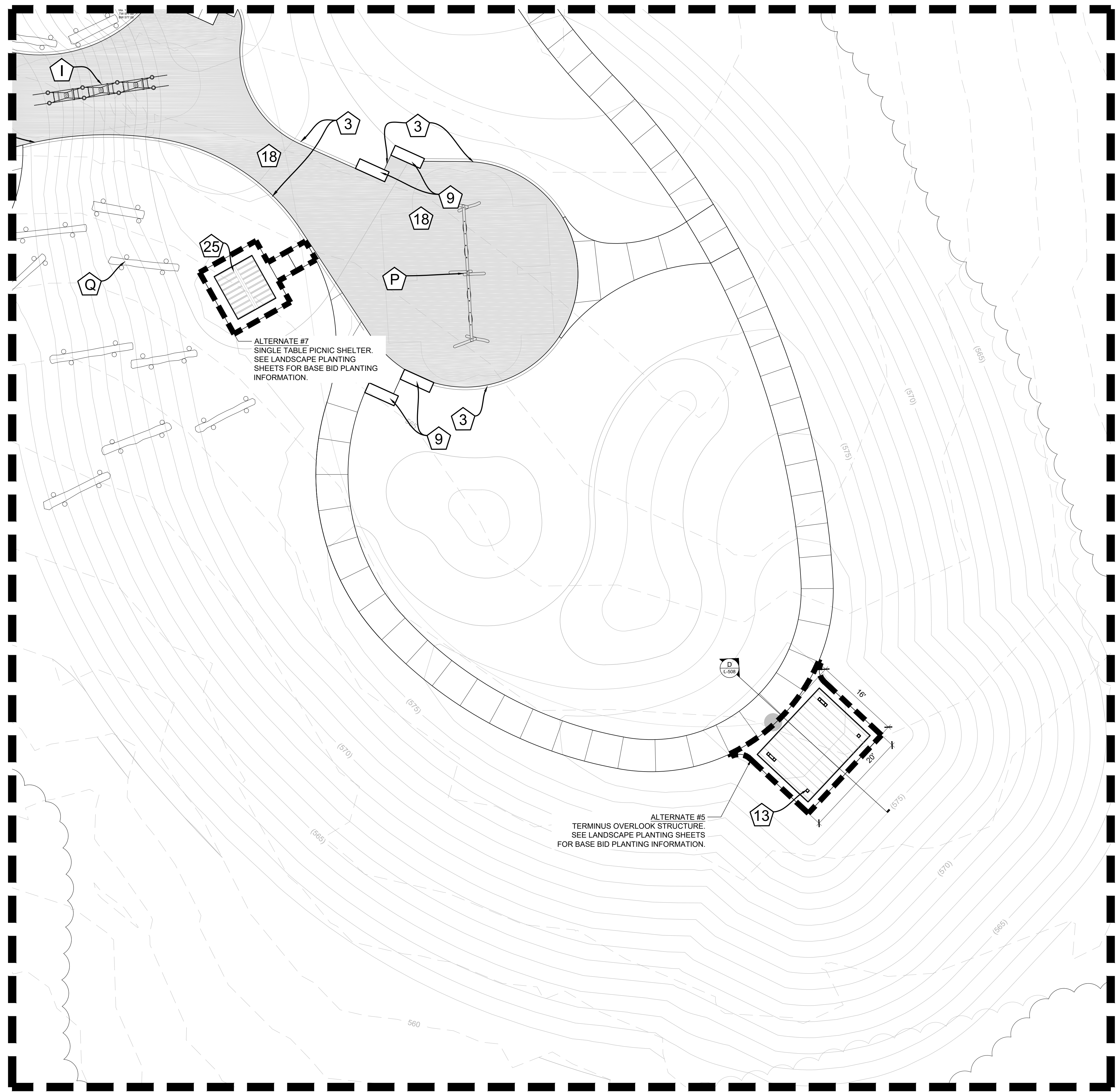
A PLAYGROUND ENLARGEMENT PLAN SCALE: 1"=10'
