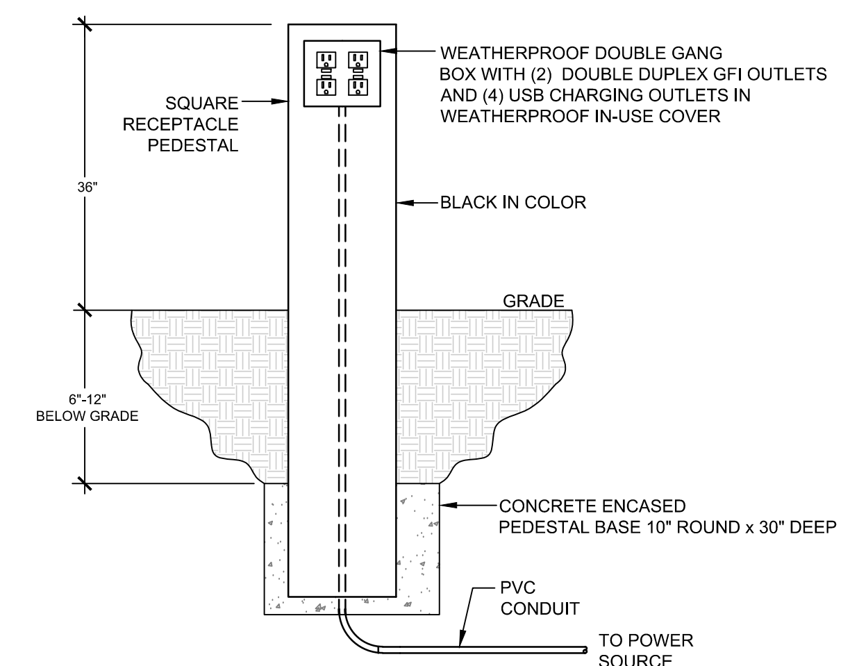
GROUND MOUNTED RECEPTACLE DETAIL SCALE: N.T.S.
