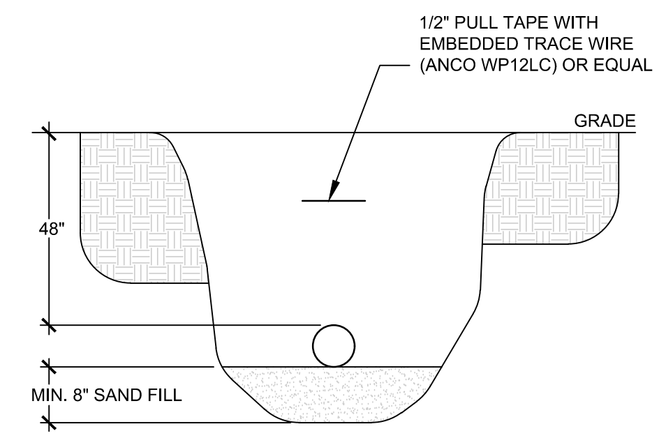
PRIMARY (UTILITY) CONDUIT BURIAL DETAIL SCALE: N.T.S.
