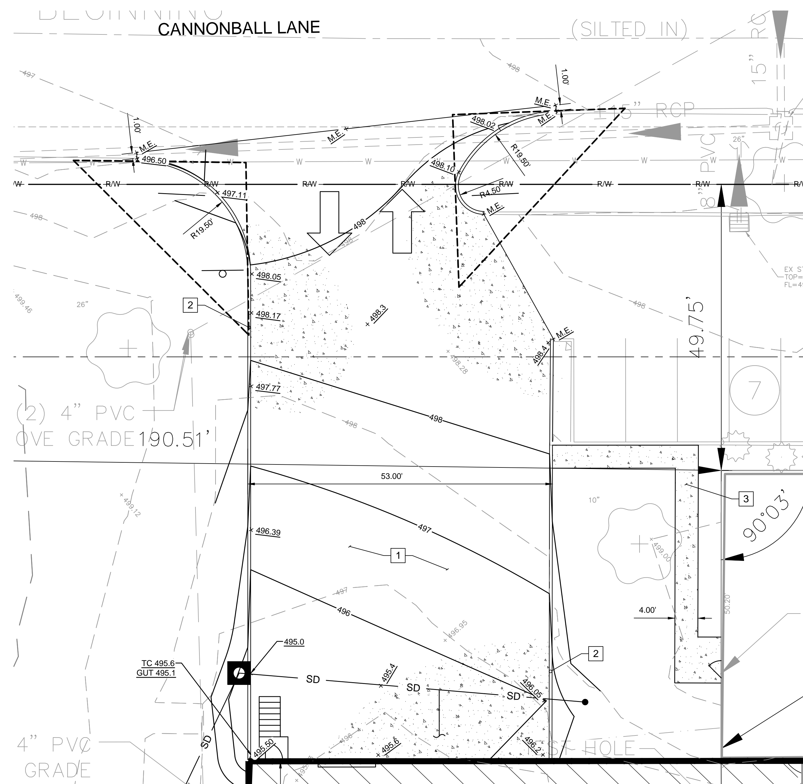
1 ENLARGEMENT B Scale: 1" = 10'
