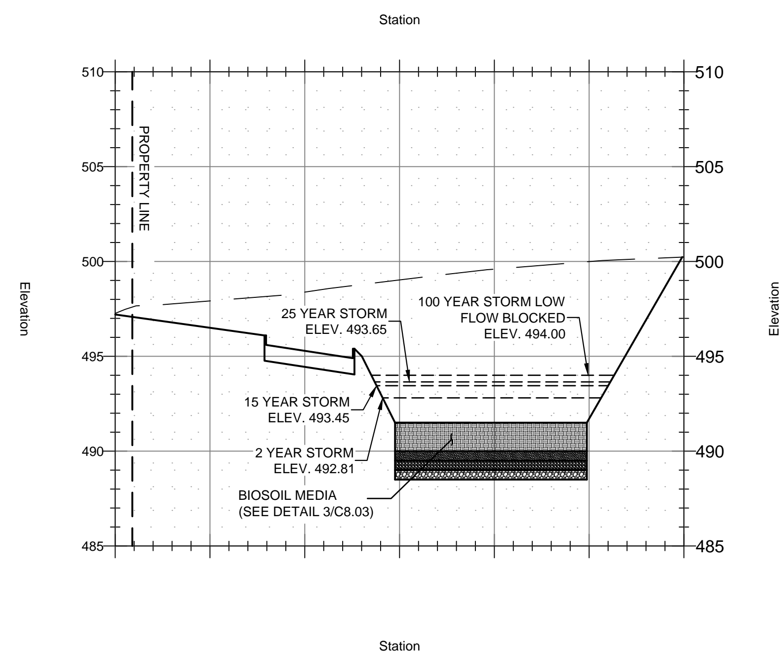
BASIN 1 PROFILE
