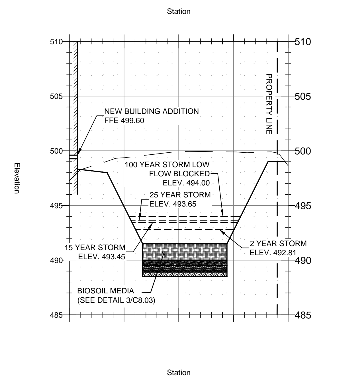
BASIN 3 PROFILE
