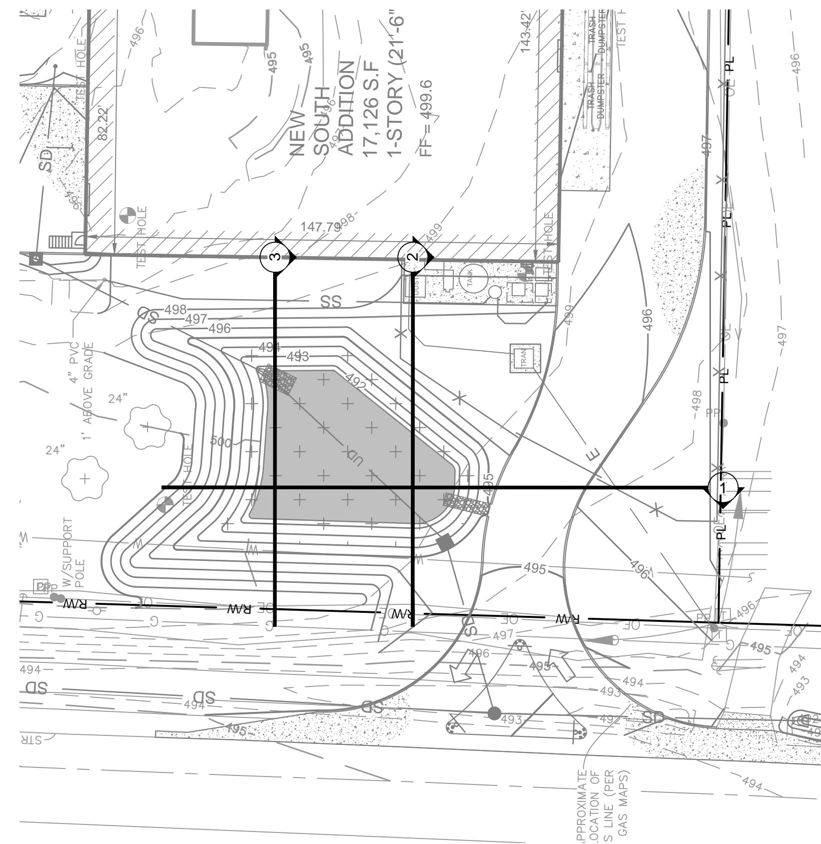
PLAN VIEW SCALE: 1" = 30' HORIZONTAL
