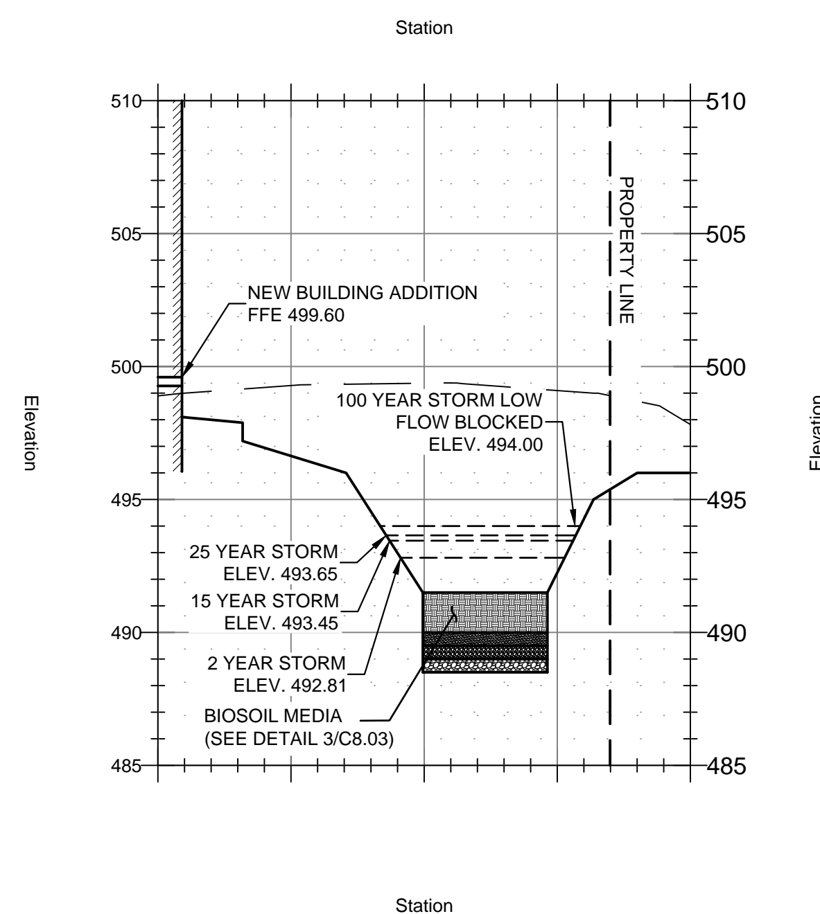
BASIN 2 PROFILE
