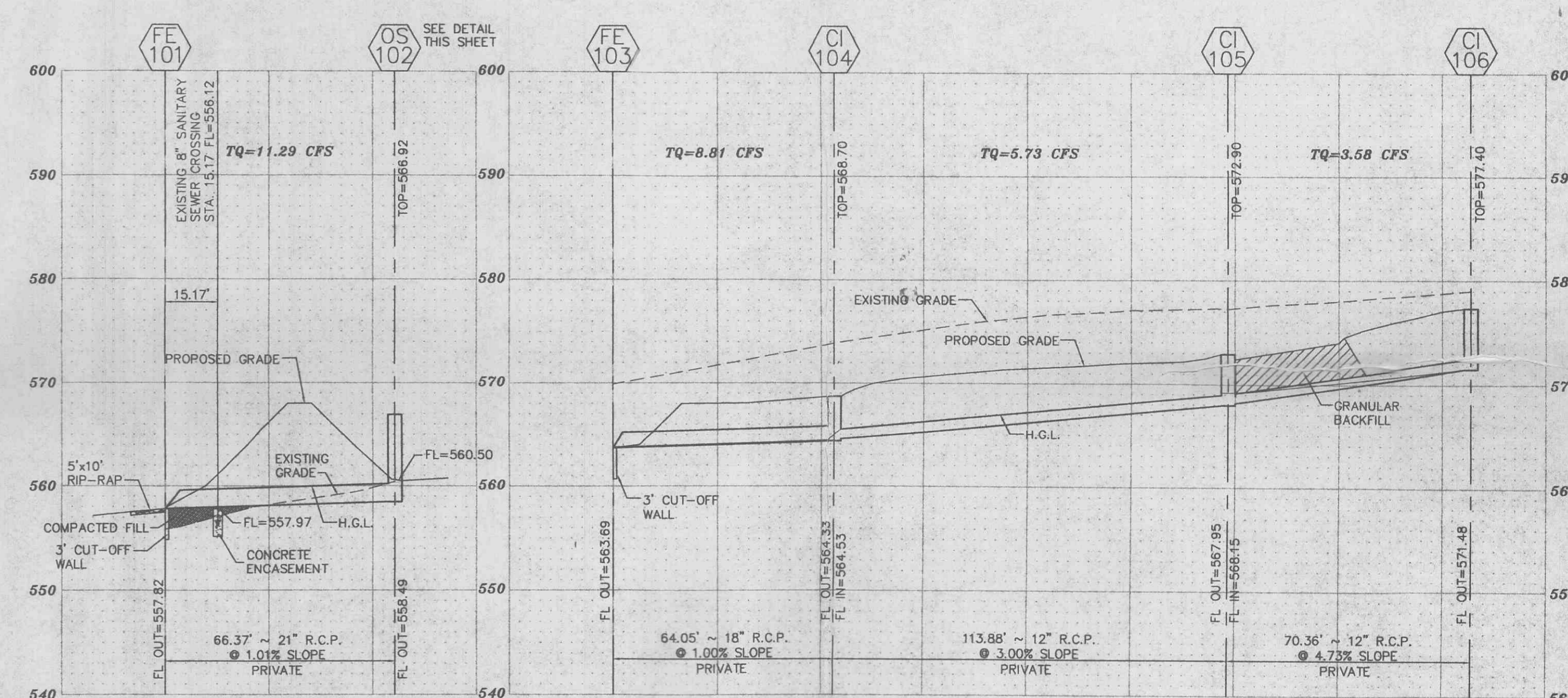
EAST ENTRANCE DETAIL SCALE: 1"=10'
