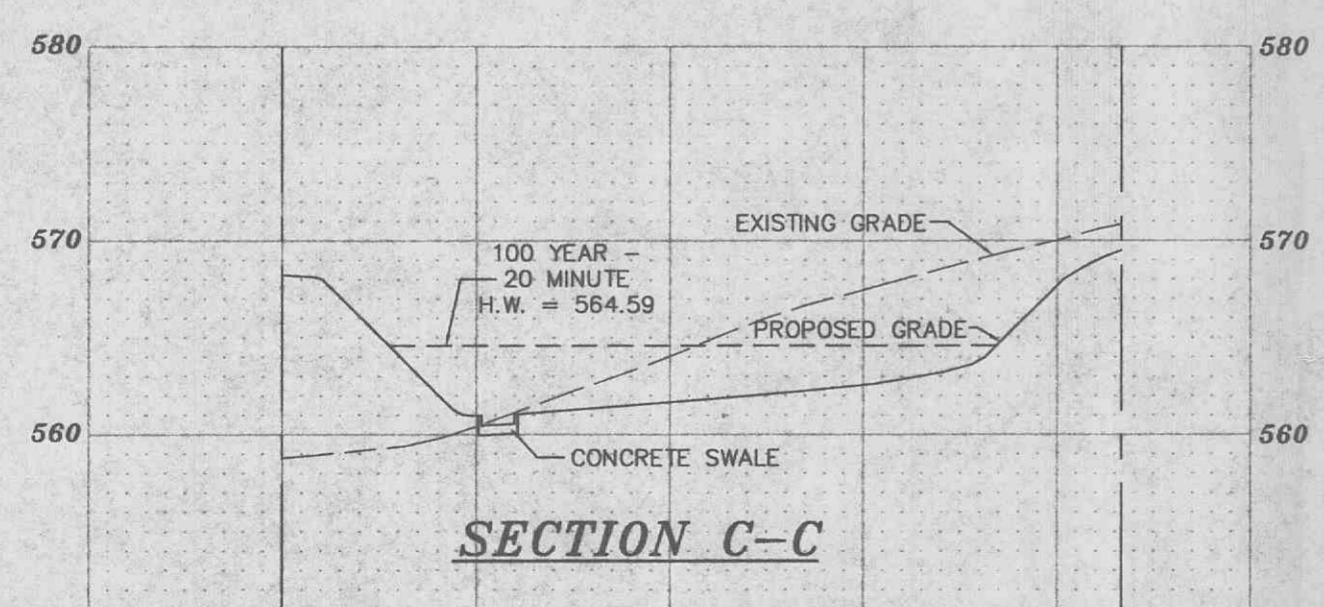
DETENTION BASIN CROSS SECTIONS SCALE: 1"=30' HORIZONTAL 1"=10' VERTICAL
