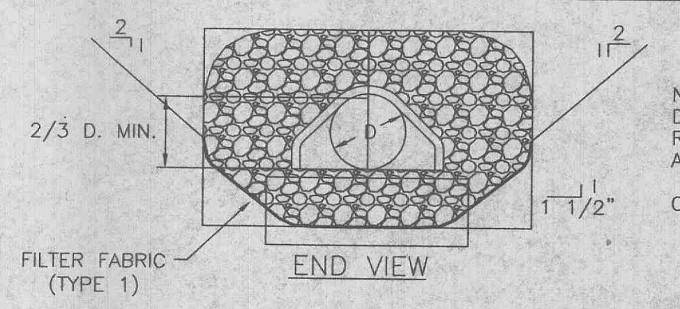
FLARED END SECTION
