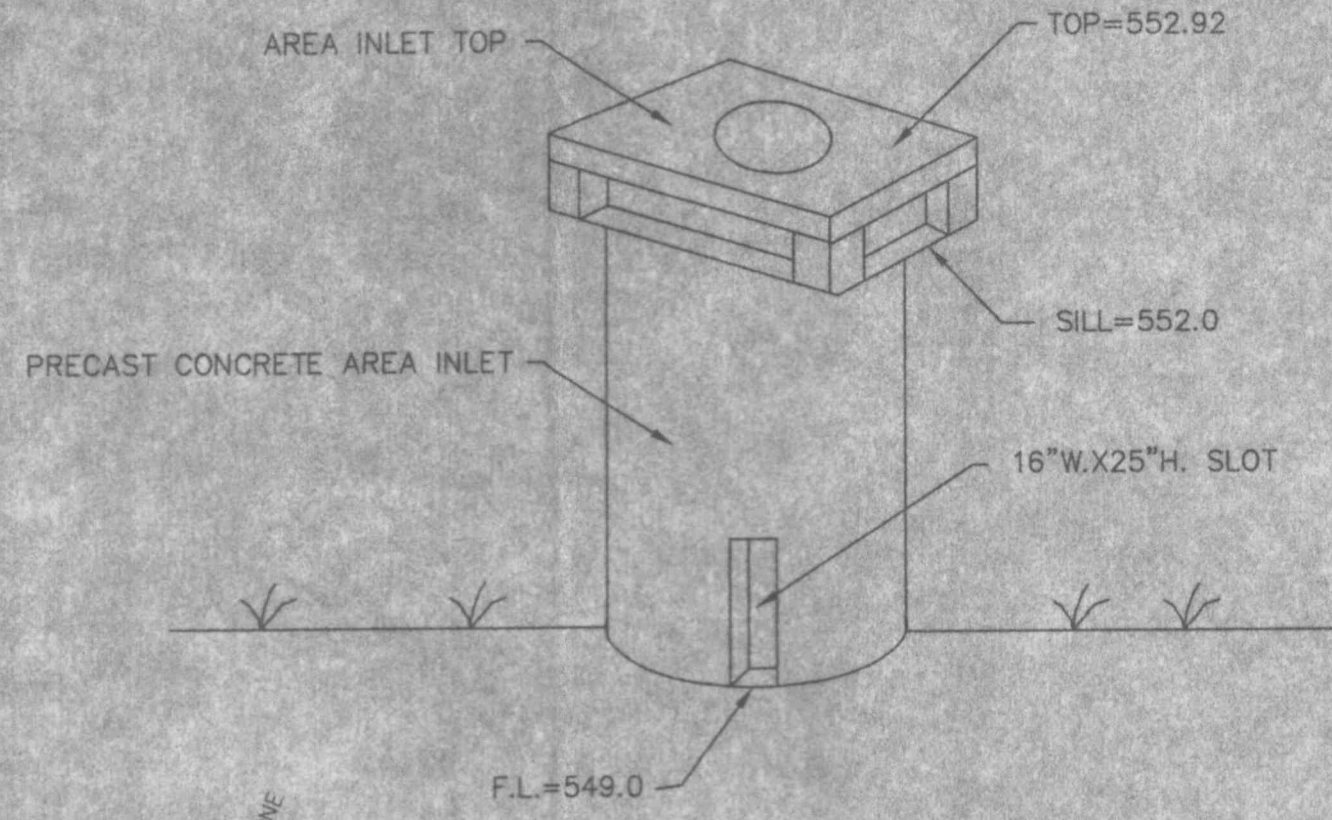
OVERFLOW STRUCTURE DETAIL NOT TO SCALE
