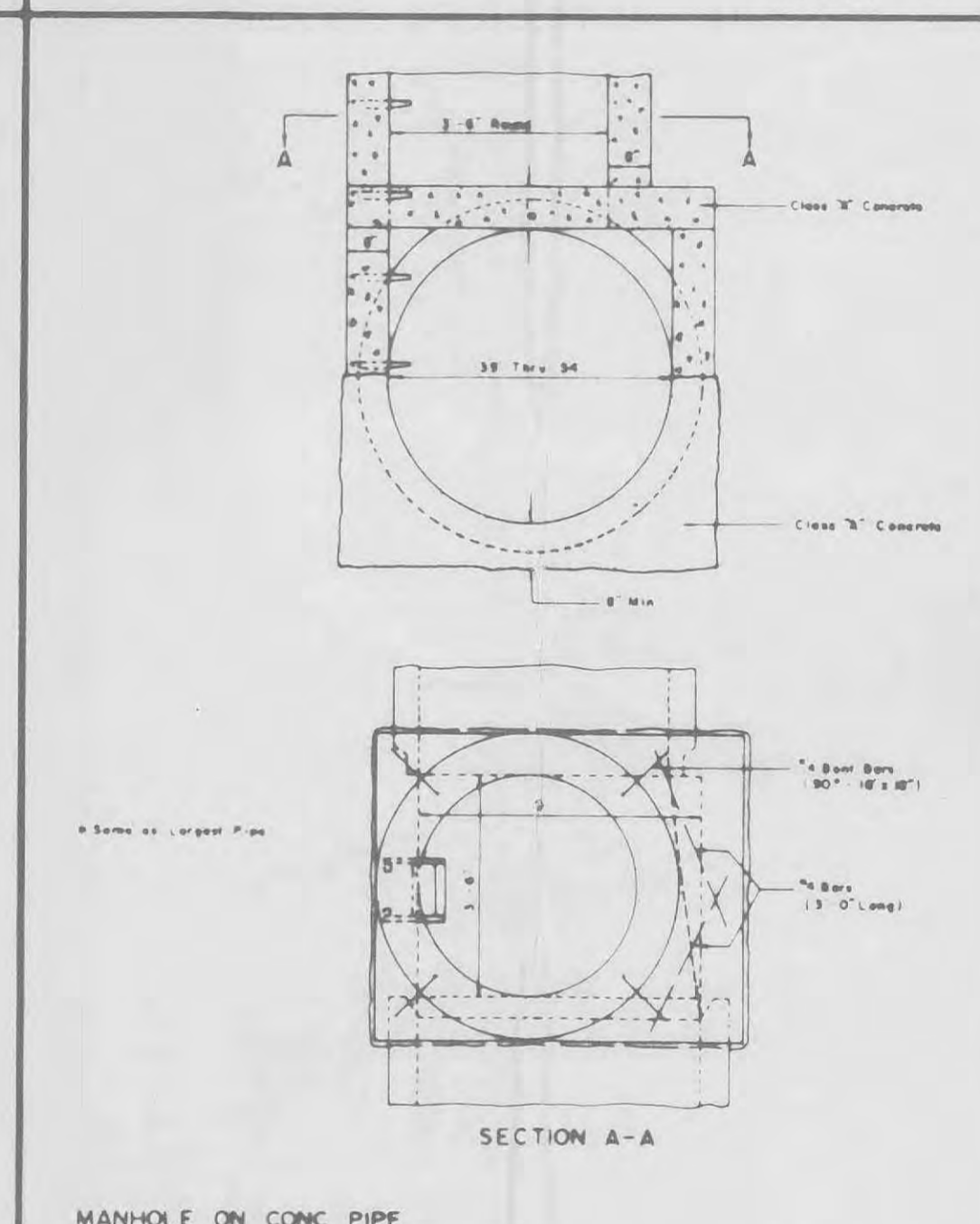
MANHOLE ON CONCRETE PIPE SEWERS 59" THRU 72" (ALTERNATE)
