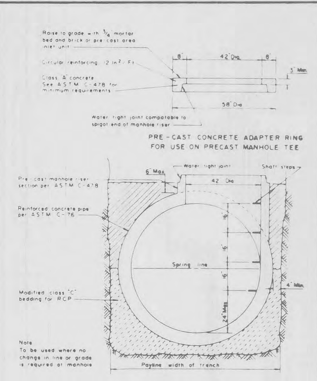
TYPICAL PRE-CAST M.M. TEE FOR REINFORCED CONCRETE PIPE SEWERS 48" AND LARGER IN DIAMETER
