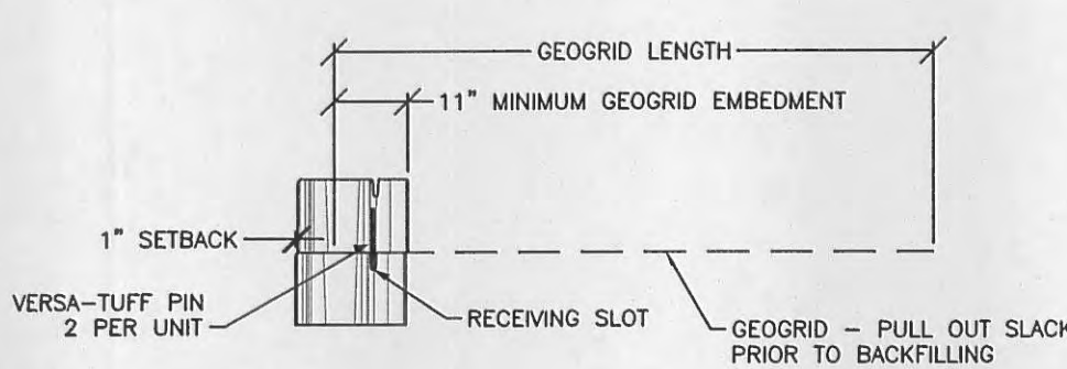
CONNECTION DETAIL NOT TO SCALE
