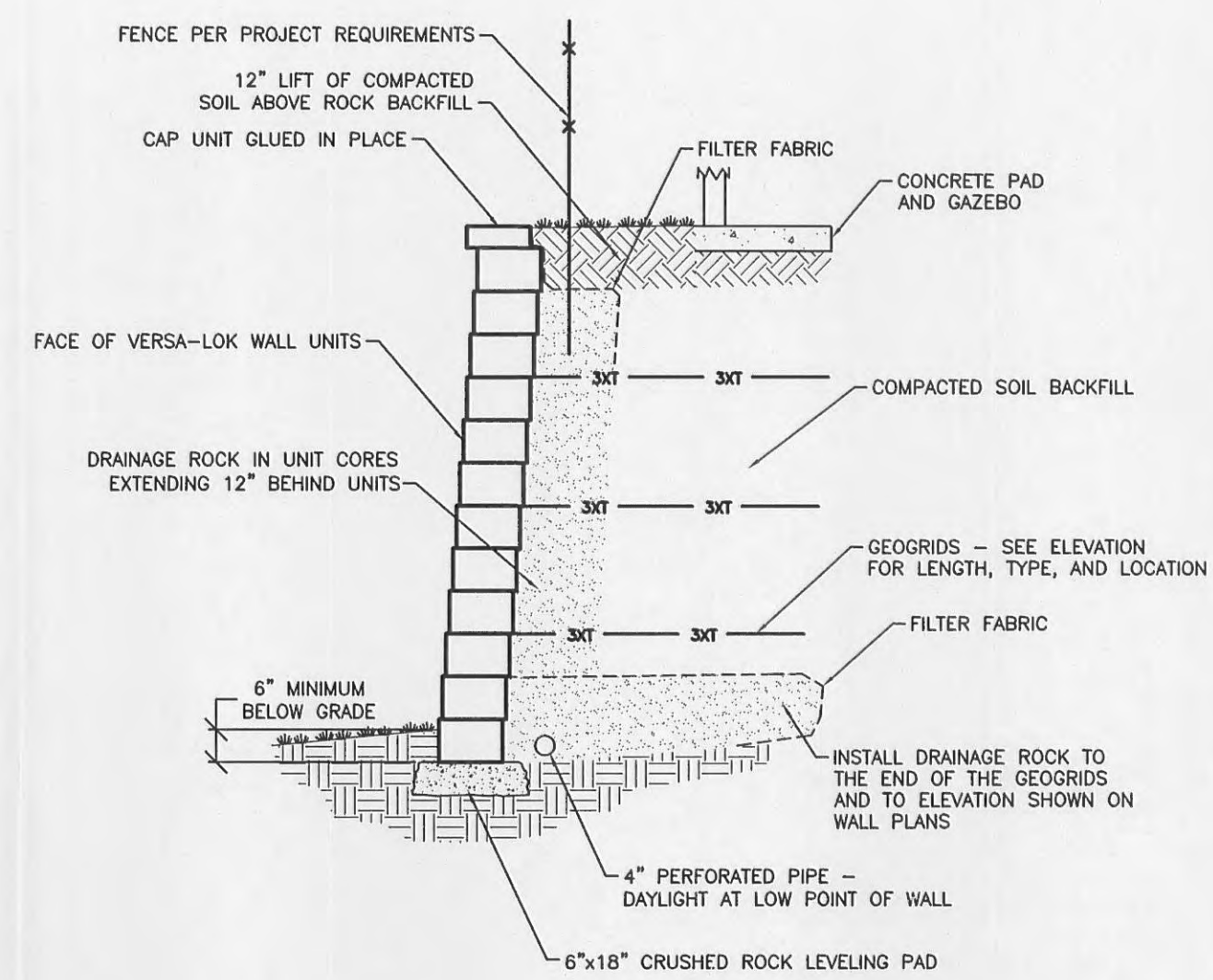
WALL F- TYPICAL SECTION NOT TO SCALE
