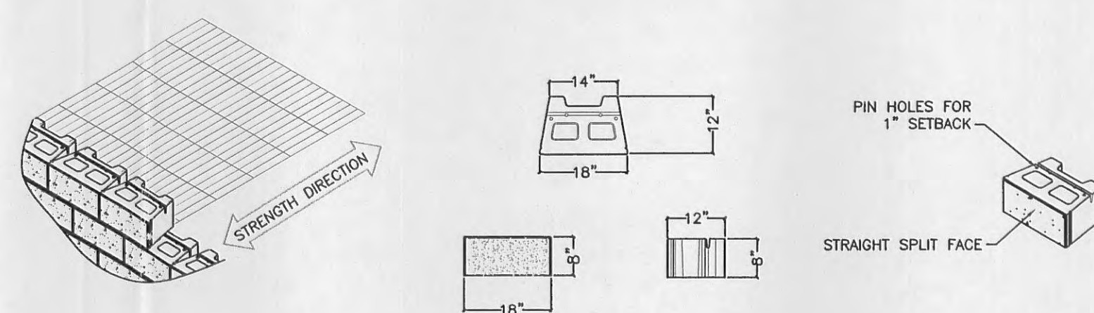
VERSALOK SQUARE FOOT UNIT NOT TO SCALE
