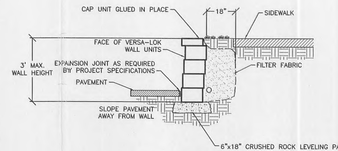
WALL E - TYPICAL SECTION NOT TO SCALE
