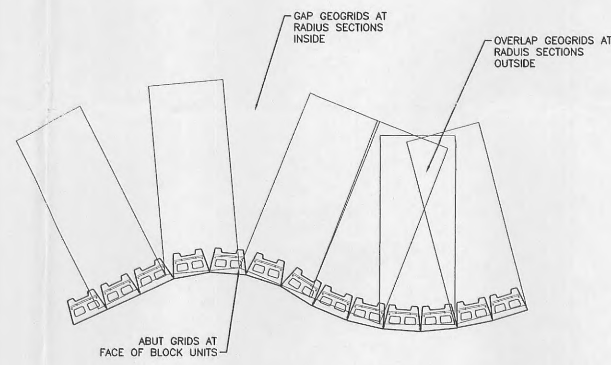
RADIUS DETAIL NOT TO SCALE
