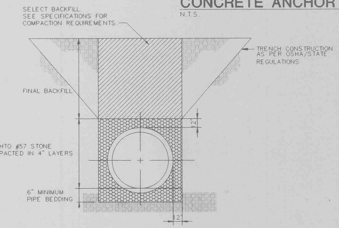
SANITARY SEWER BEDDING NO SCALE CG12
