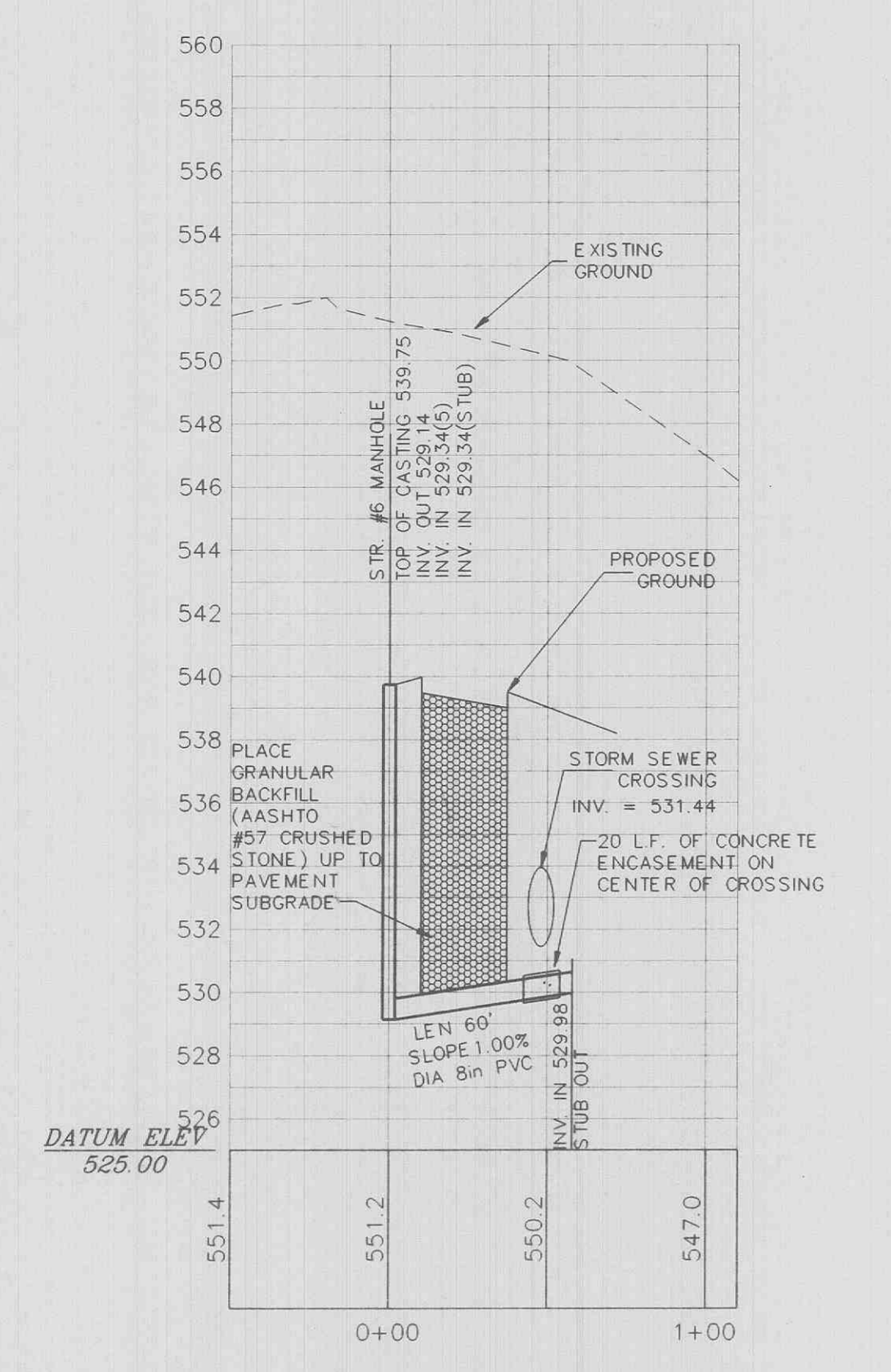
MANHOLE #6 TO STUB OUT
