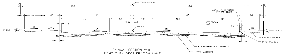
TYPICAL SECTION WITH RIGHT TURN DECELERATION LANE
