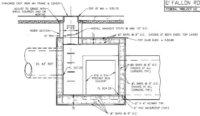
4 SECTION A-A JUNCTION CHAMBER SCALE: 1" = 2"
