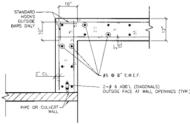
3 TYPICAL WALL CORNER DETAIL SCALE: NOT TO SCALE
