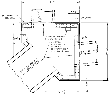
1 PLAN VIEW JUNCTION CHAMBER SCALE: 1" = 2"
