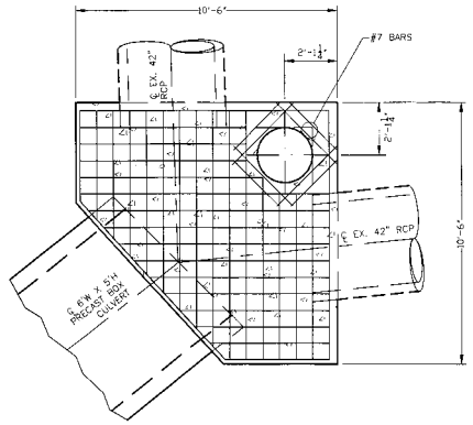
2 TOP SLAB JUNCTION CHAMBER SCALE: 1" = 2"
