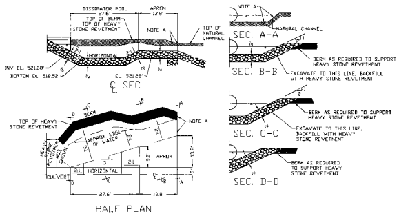
HALF PLAN
