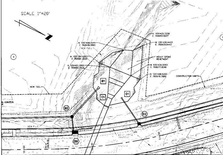
TURN AROUND DETAIL
