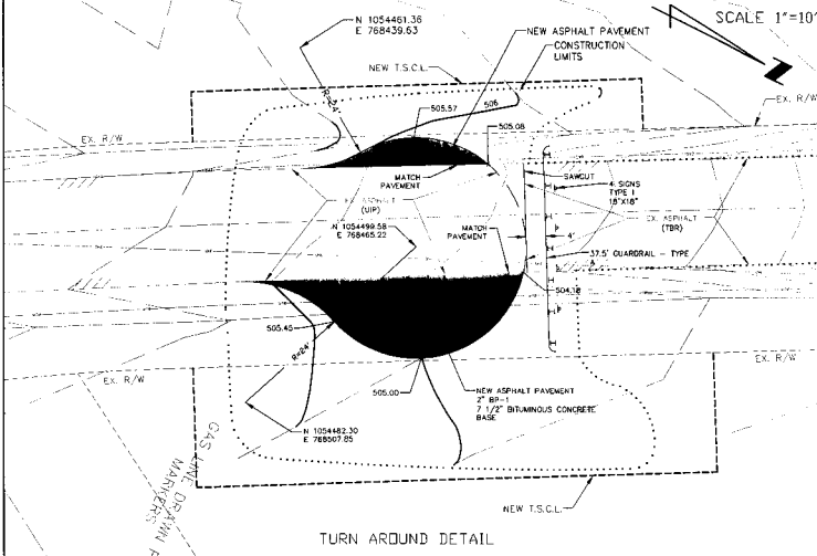
TURN AROUND DETAIL
