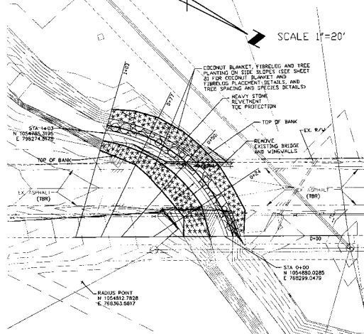
CHANNEL RESTORATION AT BRIDGE REMOVAL
