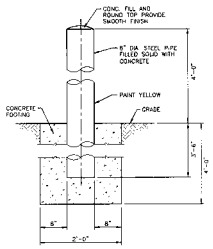
GUARD POST DETAIL NOT TO SCALE
