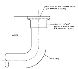
YARD DRAIN DETAIL NOT TO SCALE
