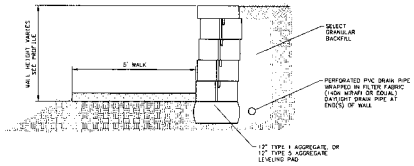
MODULAR BLOCK WALL TYPICAL SECTION NOT TO SCALE
