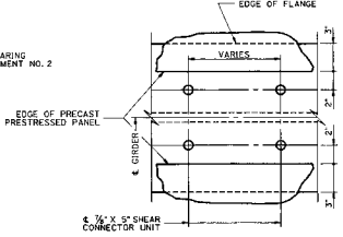
SHEAR CONNECTOR LAYOUT
