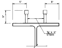
SHEAR CONNECTOR DETAIL
