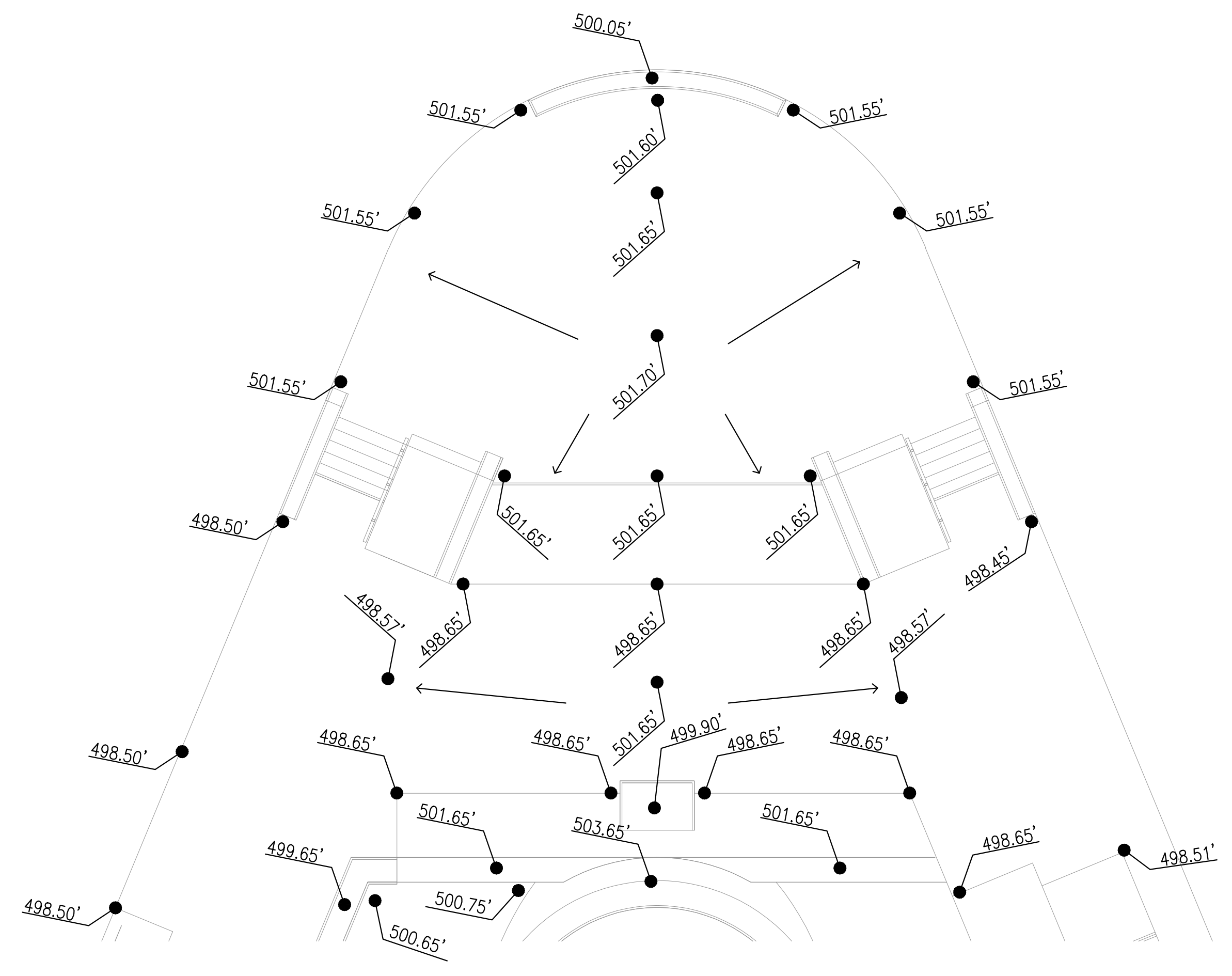
SKATEPARK CONCRETE ELEVATION (ADD ALTERNATE)
