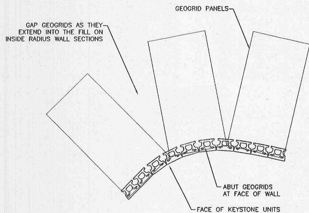
INSIDE RADIUS DETAIL NOT TO SCALE
