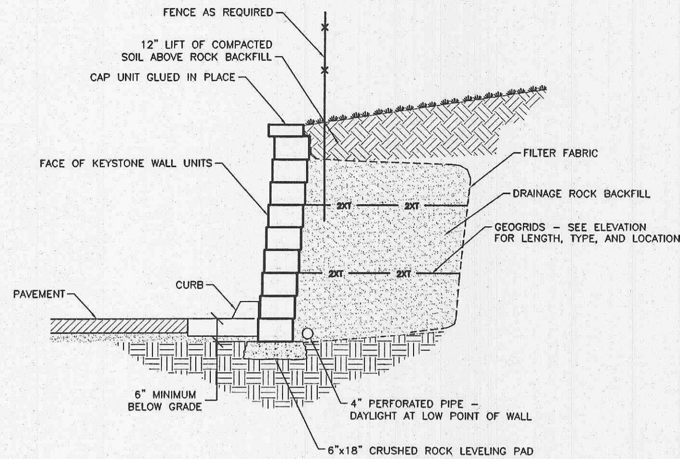
TYPICAL SECTION NOT TO SCALE
