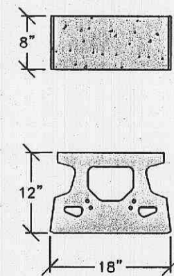
COMPAC II UNIT NOT TO SCALE
