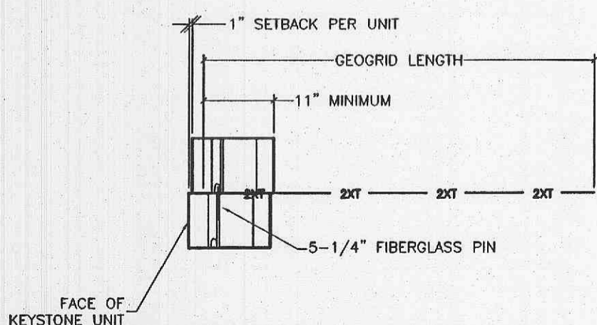
CONNECTION DETAIL NOT TO SCALE
