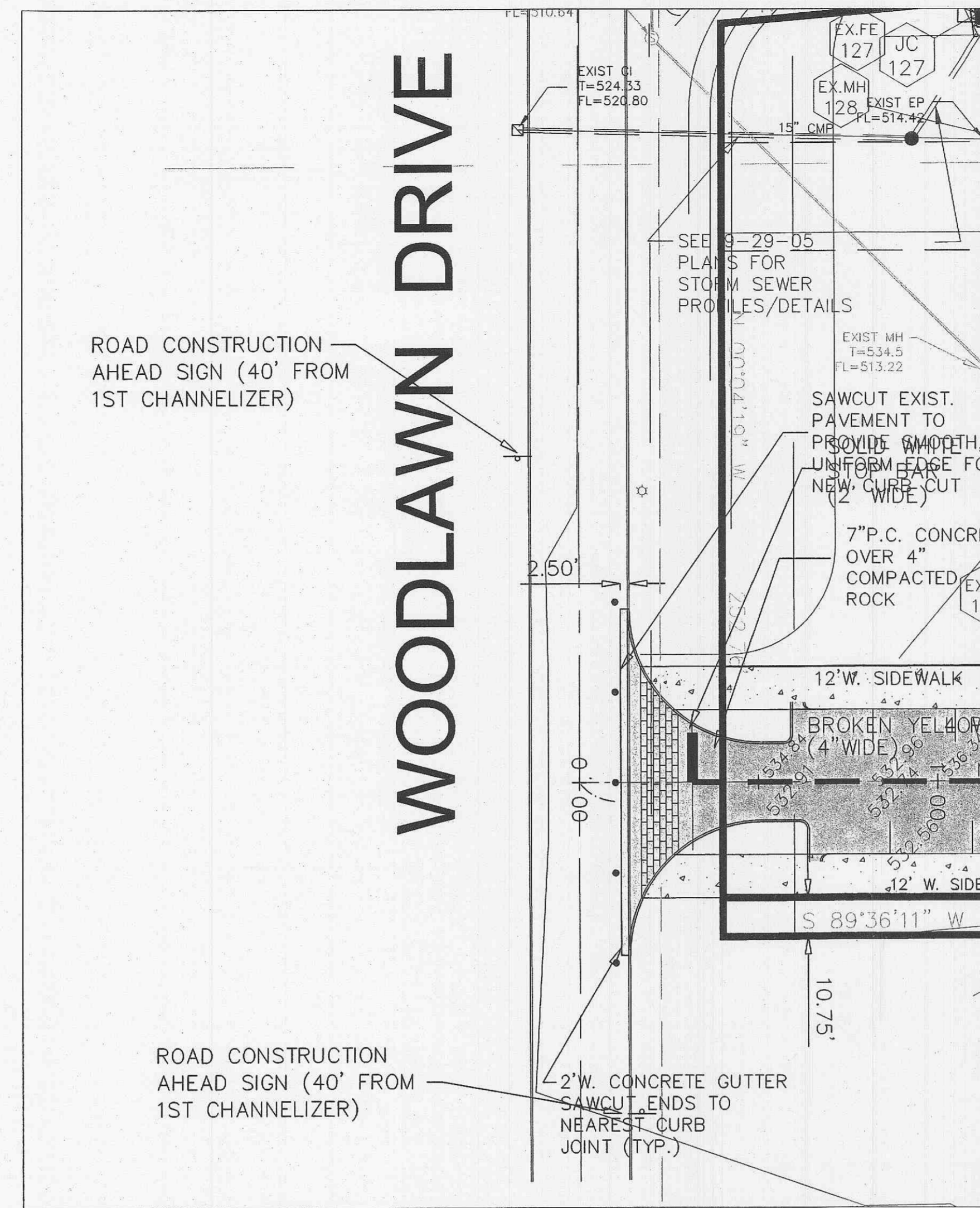
TRAFFIC CONTROL DETAIL FOR INTERSECTION OF WOODLAWN DR. AND WEST ELM ST. SCALE: 1:30
