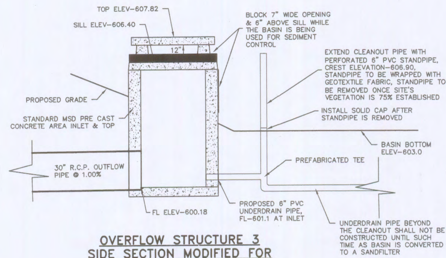
TEMPORARY SEDIMENT BASIN A
