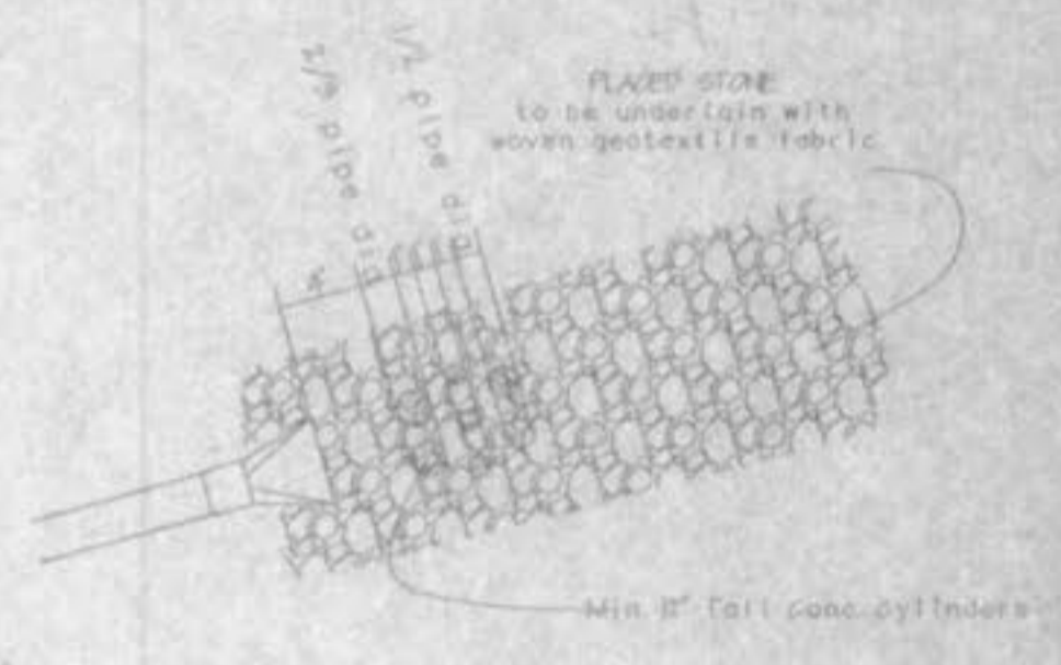
Energy Dissipator
