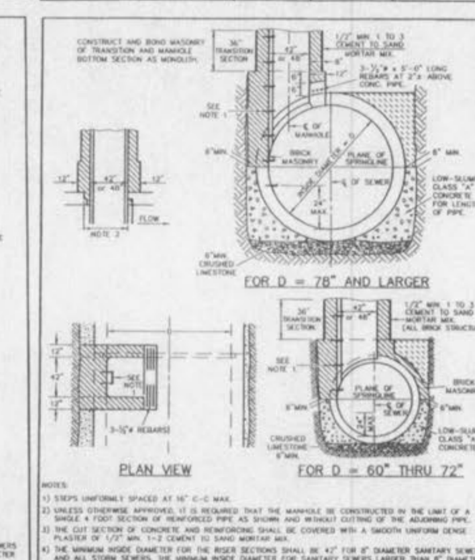
TYPICAL MANHOLE BASE REINFORCED CONCRETE PIPE 60" AND LARGER IN DIAMETER METROPOLITAN ST. LOUIS SEWER DISTRICT Standard Details of Sewer Construction Dr. W.S.H./SAM Ch. J.C.K. 2000 SHEET 15
