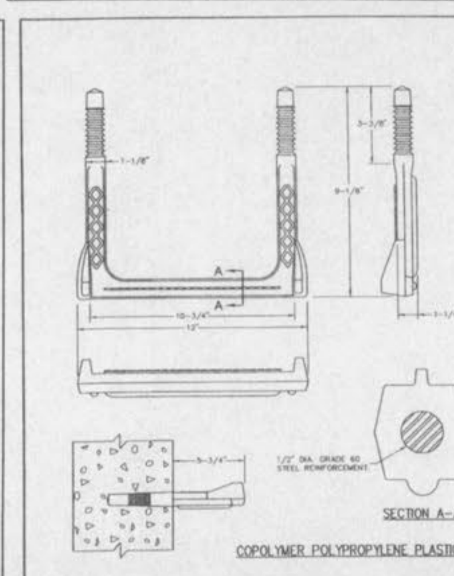
MANHOLE STEP FOR PRECAST & CAST-IN-PLACE MANHOLE METROPOLITAN ST. LOUIS SEWER DISTRICT Standard Details of Sewer Construction Dr. D.A.B./SAM Ch. J.C.K. 2000 SHEET 58
