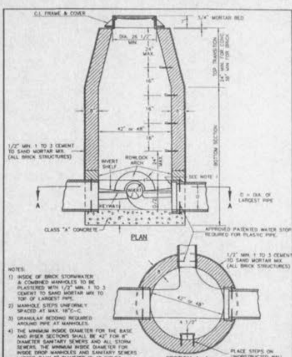
LINE MANHOLE PIPE SEWERS 8"-24" DIA. METROPOLITAN ST. LOUIS SEWER DISTRICT Standard Details of Sewer Construction Dr. W.S.H./SAM Ch. J.C.K. 2000 SHEET 10
