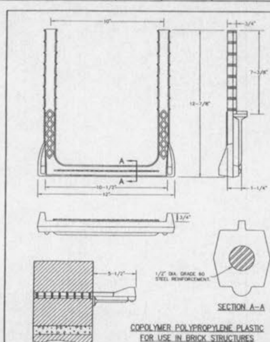
PSI-B MANHOLE STEP INTO JOINT METROPOLITAN ST. LOUIS SEWER DISTRICT Standard Details of Sewer Construction Dr. W.S.H./SAM Ch. J.C.K. 2000 SHEET 57
