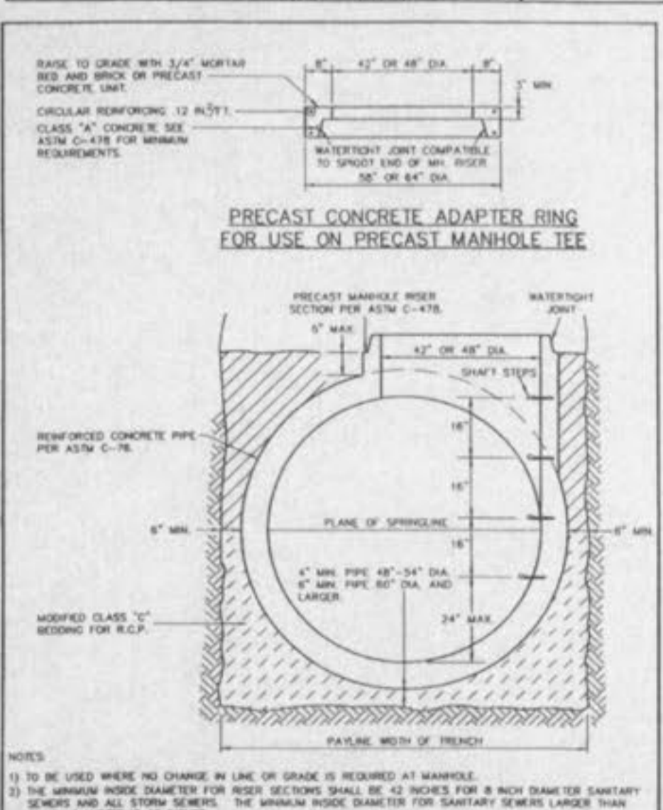
TYPICAL PRECAST MANHOLE TEE FOR REINFORCED CONCRETE PIPE SEWERS 48 INCH AND LARGER IN DIAMETER METROPOLITAN ST. LOUIS SEWER DISTRICT Standard Details of Sewer Construction Dr. W.S.H./SAM Ch. J.C.K. 2000 SHEET 24
