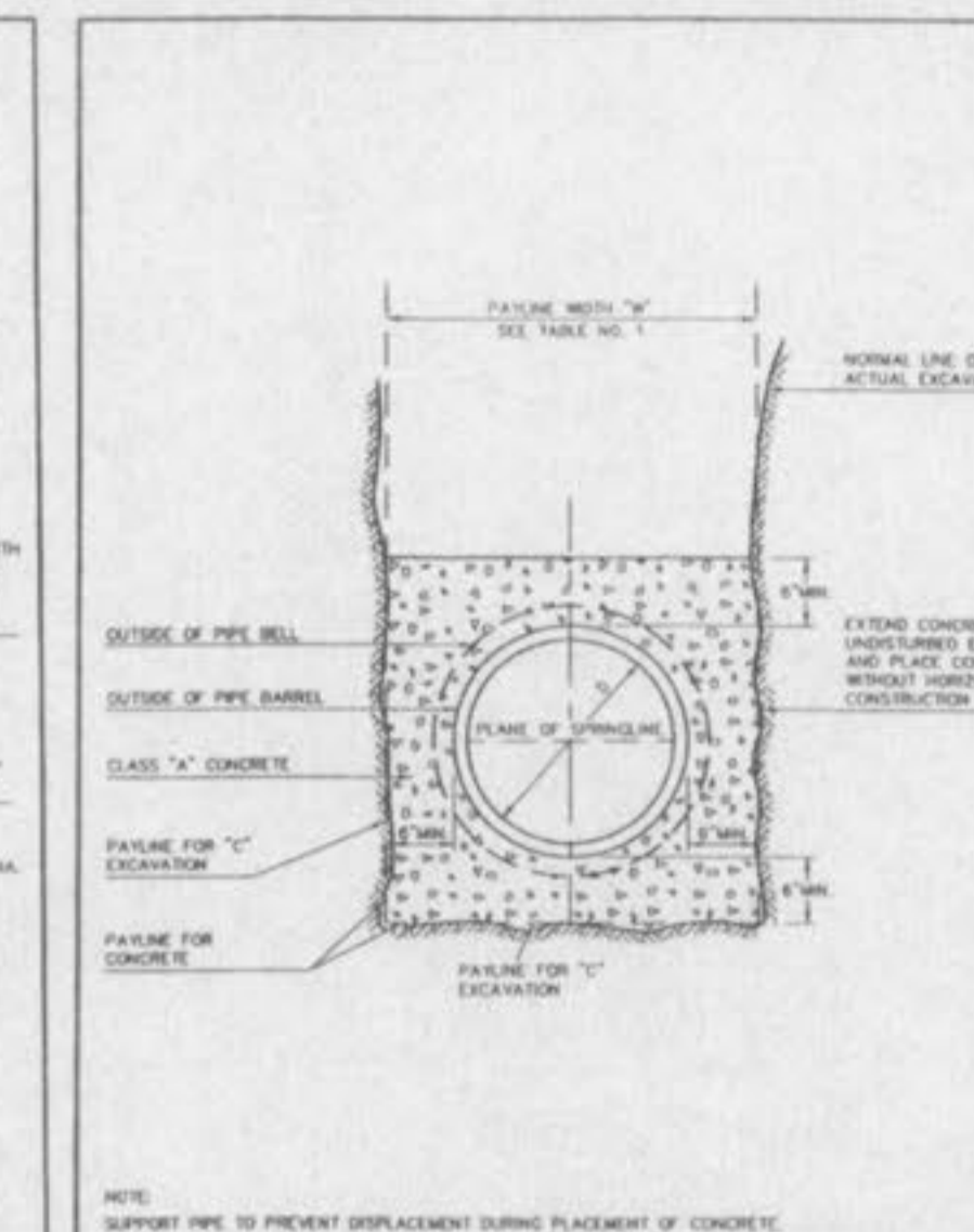
CONCRETE ENCASEMENT METROPOLITAN ST. LOUIS SEWER DISTRICT Standard Details of Sewer Construction Dr. W.S.H./SAM Ch. J.C.K. 2000 SHEET 8
