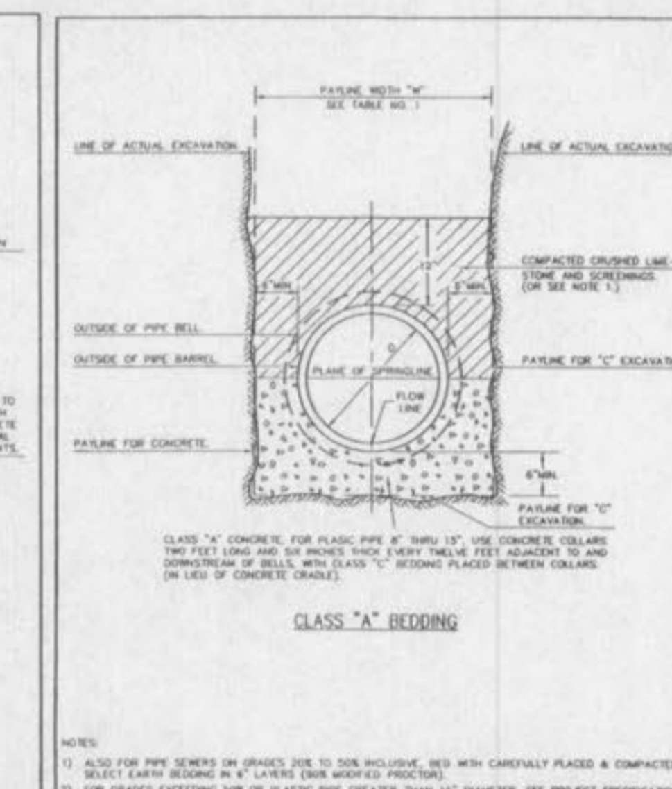
CLASS "A" BEDDING METROPOLITAN ST. LOUIS SEWER DISTRICT Standard Details of Sewer Construction Dr. W.S.H./SAM Ch. J.C.K. 2000 SHEET 9
