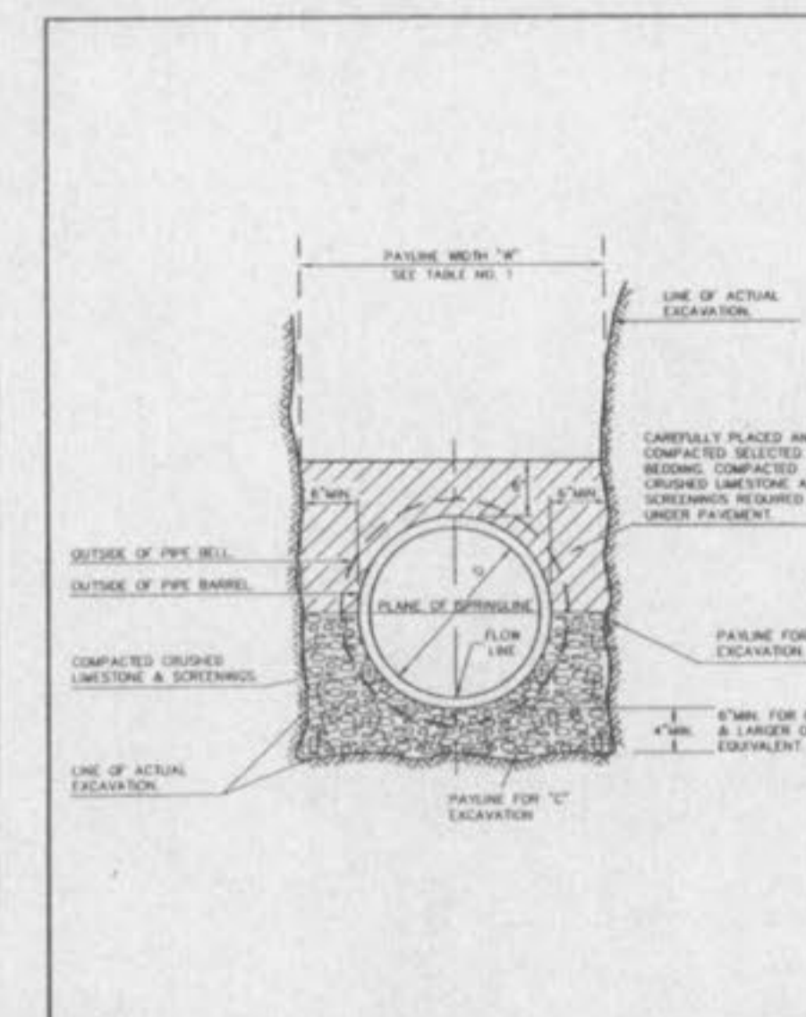
PIPE BEDDING CLASS "C" (MODIFIED FOR REINFORCED CONCRETE PIPE) METROPOLITAN ST. LOUIS SEWER DISTRICT Standard Details of Sewer Construction Dr. W.S.H./SAM Ch. J.C.K. 2000 SHEET 5
