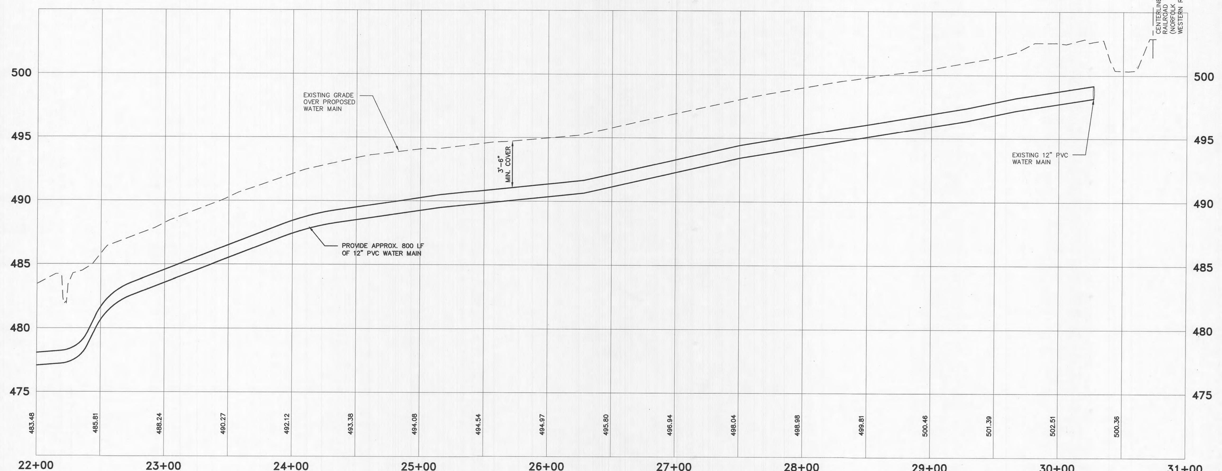
MEMC DRIVE PROFILE SCALE: 1"=40' HORIZONTAL 1"=4' VERTICAL
