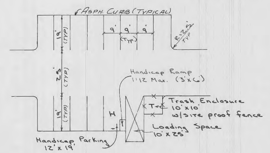
Parking Layout
