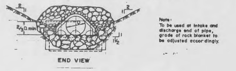
RIP RAP / DISSIPATOR DETAIL
