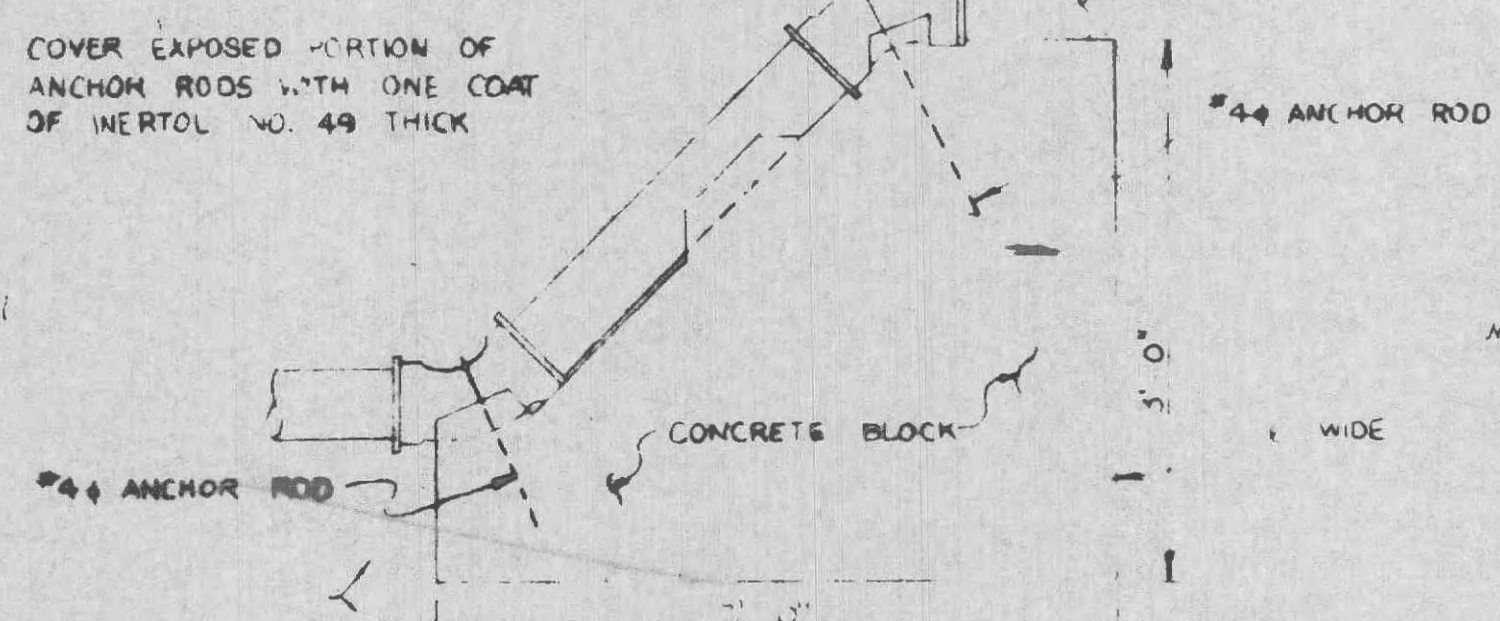
DETAIL THRUST BLOCK FOR VERTICAL OFFSETS
