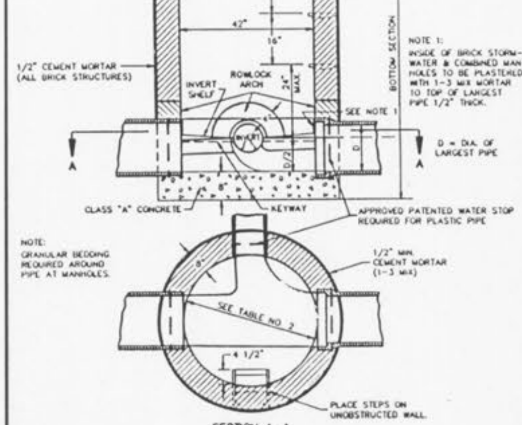
LINE MANHOLE METROPOLITAN ST. LOUIS SEWER DISTRICT Standard Details of Sewer Construction Dr. W.S.H. Ch. J.C.K. 1992 SHEET 8
