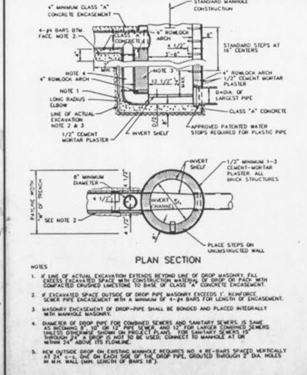
OUTSIDE FOULWATER DROP MANHOLE METROPOLITAN ST. LOUIS SEWER DISTRICT Standard Details of Sewer Construction Dr. W.S.H. Ch. J.C.K. 1992 SHEET 14
