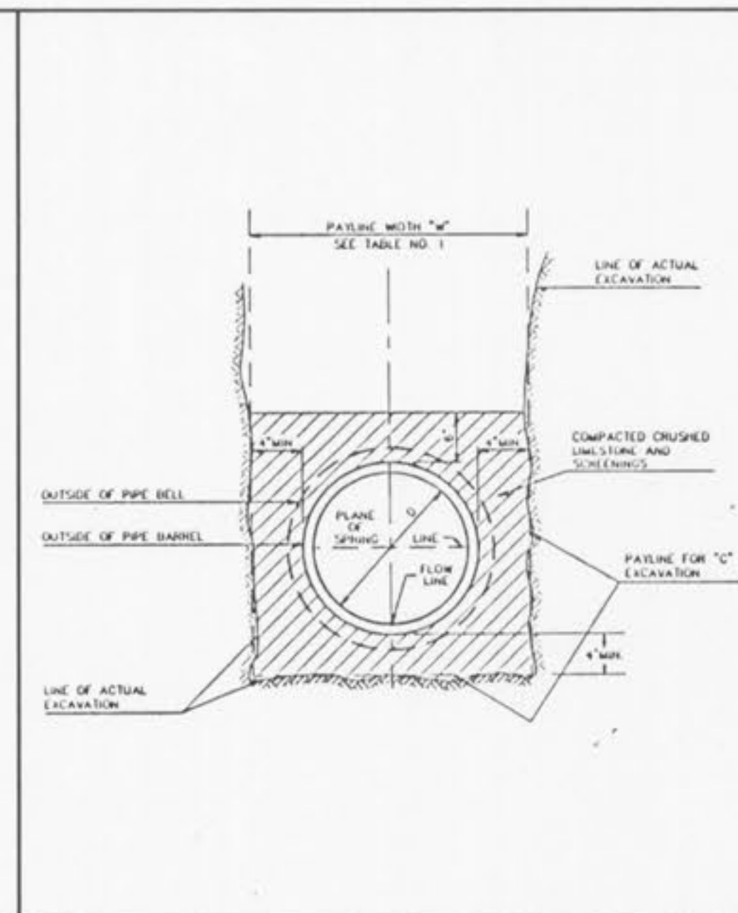
PIPE BEDDING CLASS "C" (MODIFIED FOR REINFORCED CONCRETE PIPE) METROPOLITAN ST. LOUIS SEWER DISTRICT Standard Details of Sewer Construction Dr. W.S.H. Ch. J.C.K. 1992 SHEET 3
