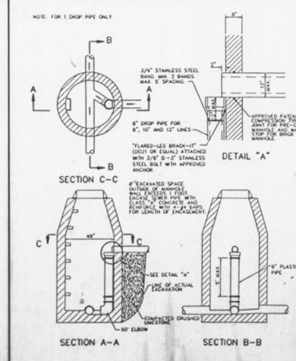
INSIDE FOULWATER DROP MANHOLE METROPOLITAN ST. LOUIS SEWER DISTRICT Standard Details of Sewer Construction Dr. W.S.H. Ch. J.C.K. 1992 SHEET 15
