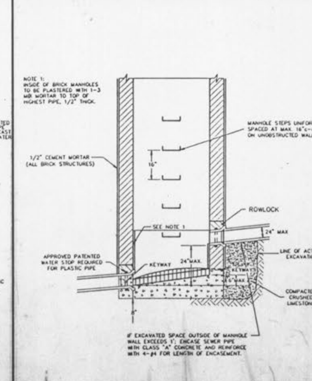
INSIDE FOULWATER DROP MANHOLE (FOR FREE-FALL) METROPOLITAN ST. LOUIS SEWER DISTRICT Standard Details of Sewer Construction Dr. R.C.W. Ch. J.C.K. 1992 SHEET 16
