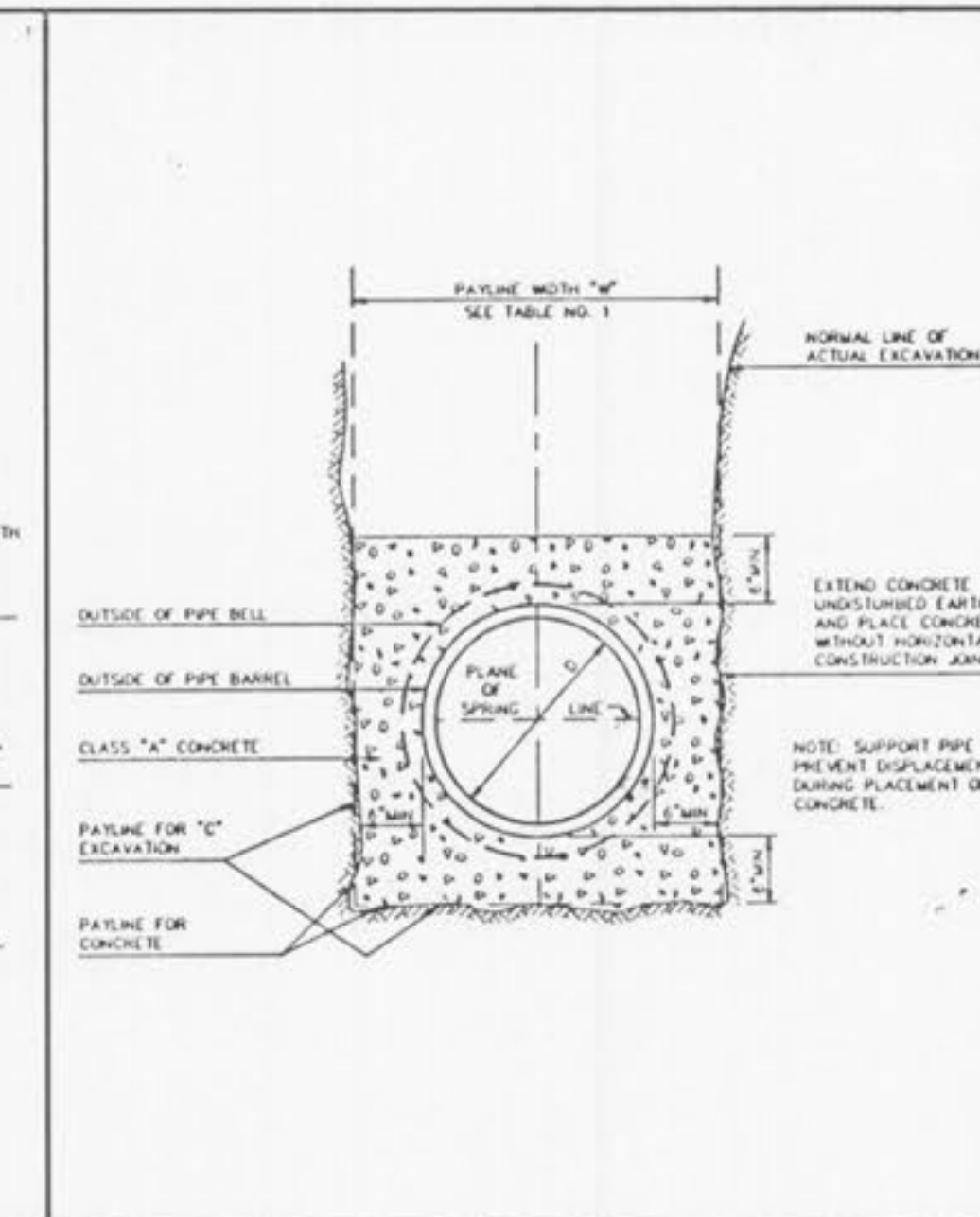
CONCRETE CRADLE METROPOLITAN ST. LOUIS SEWER DISTRICT Standard Details of Sewer Construction Dr. W.S.H. Ch. J.C.K. 1992 SHEET 5
