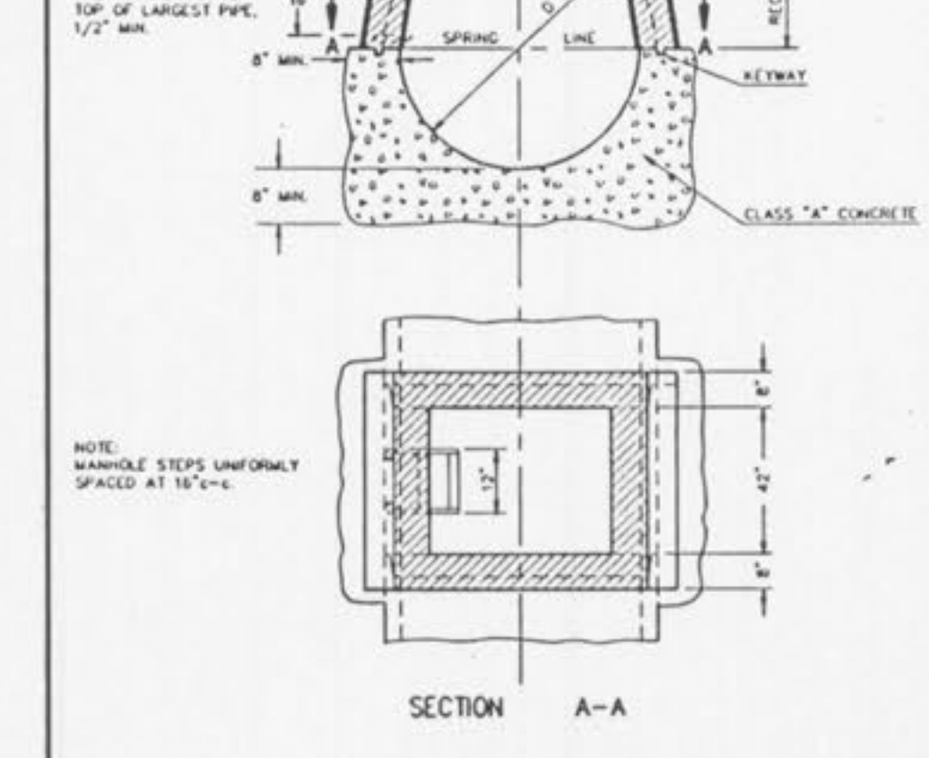
MANHOLE ON CONCRETE PIPE SEWERS 39" THRU 54" DIAMETER METROPOLITAN ST. LOUIS SEWER DISTRICT Standard Details of Sewer Construction Dr. W.S.H. Ch. J.C.K. 1992 SHEET 11
