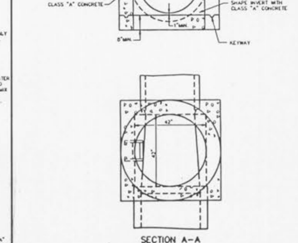
MANHOLE ON PIPE SEWER 27" THRU 36" (ALTERNATE) METROPOLITAN ST. LOUIS SEWER DISTRICT Standard Details of Sewer Construction Dr. D.A.B. Ch. J.C.K. 1992 SHEET 10
