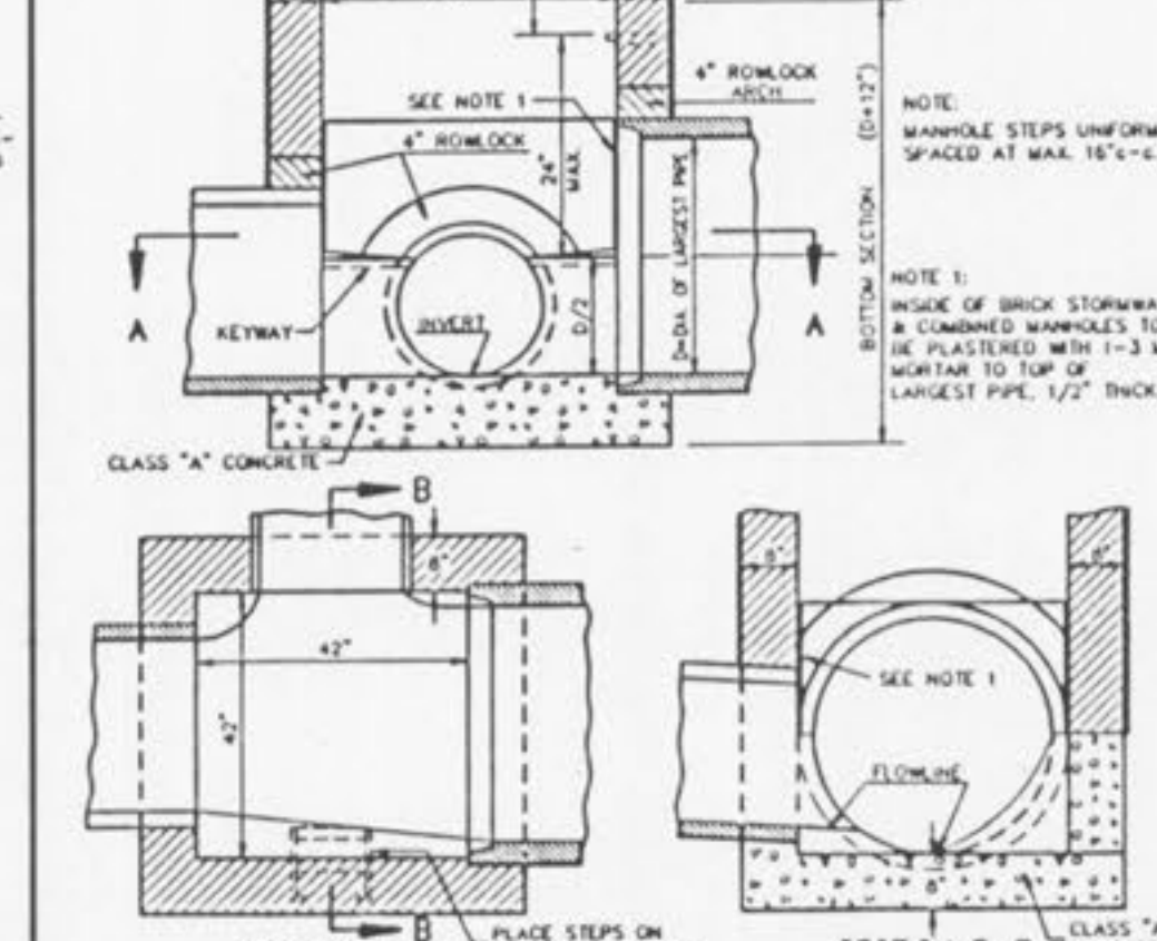
TYPICAL LINE MANHOLE ON PIPE SEWER 27" THRU 36" IN DIAMETER METROPOLITAN ST. LOUIS SEWER DISTRICT Standard Details of Sewer Construction Dr. W.S.H. Ch. J.C.K. 1992 SHEET 9
