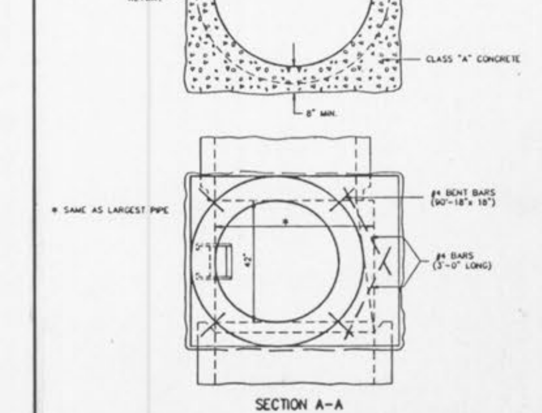
MANHOLE ON CONC. PIPE 39" THRU 54" (ALTERNATE) METROPOLITAN ST. LOUIS SEWER DISTRICT Standard Details of Sewer Construction Dr. W.S.H. Ch. J.C.K. 1992 SHEET 12
