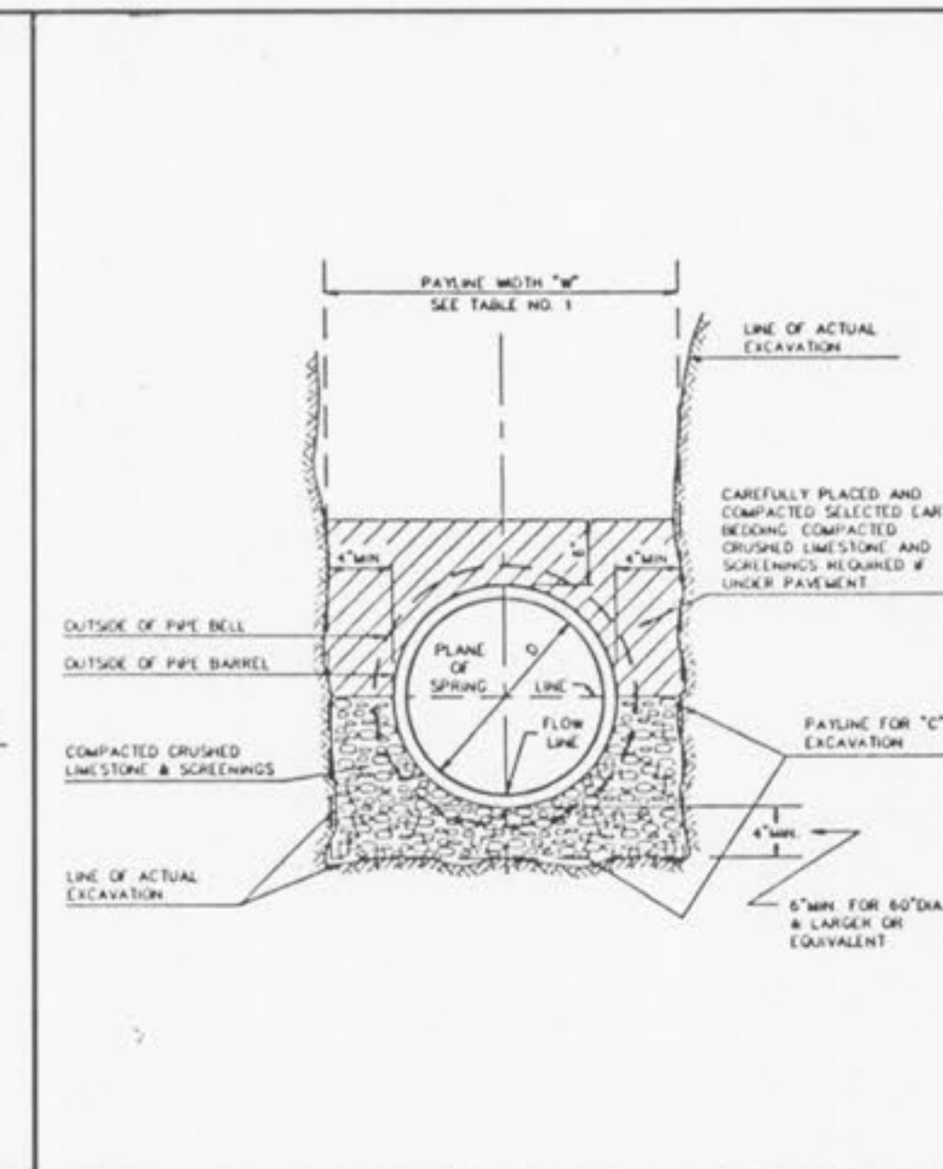
CONCRETE ENCASEMENT METROPOLITAN ST. LOUIS SEWER DISTRICT Standard Details of Sewer Construction Dr. W.S.H. Ch. J.C.K. 1992 SHEET 4
