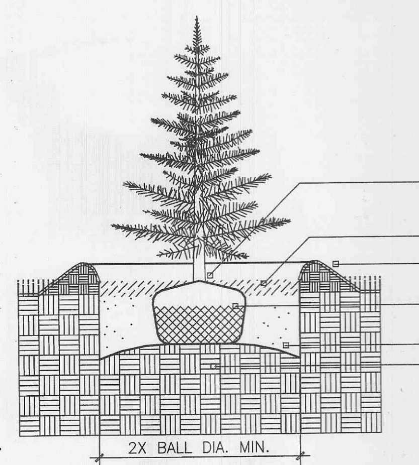
NOTE: USE SHREDDED BARK MULCH ONLY EVERGREEN TREE PLANTING N.T.S.
