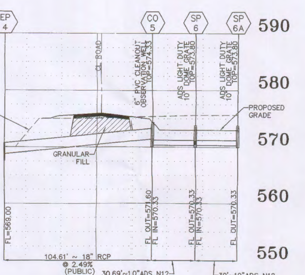
STORM SEWER PROFILE SCALES: HORIZ. 1"=40' VERT. 1"=10'
