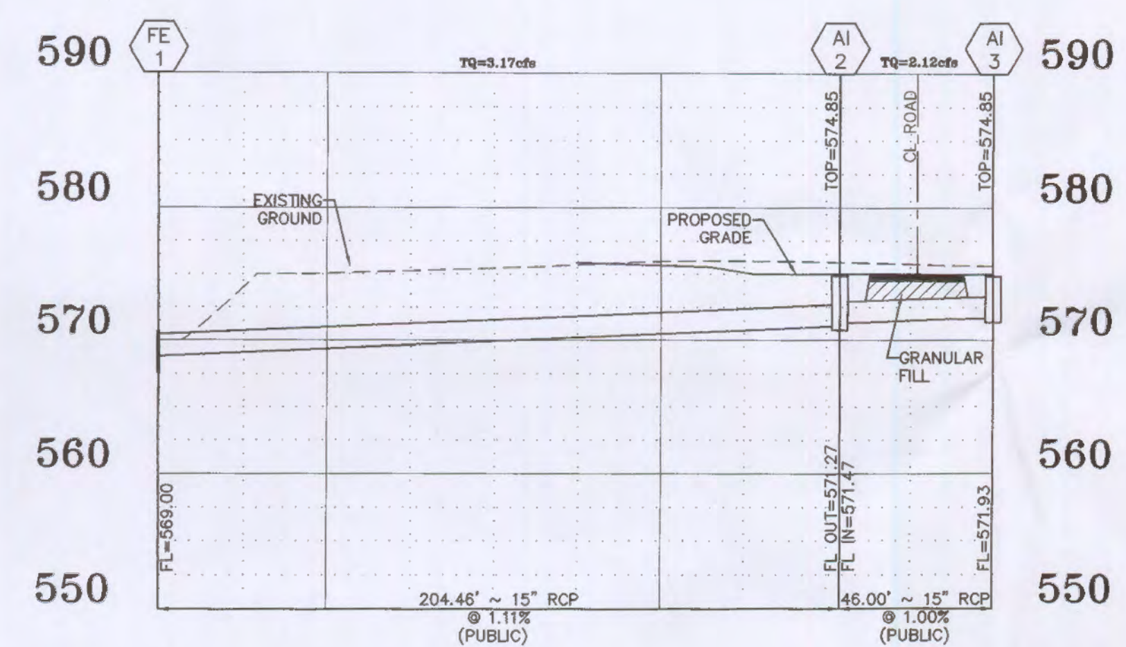
STORM SEWER PROFILE SCALES: HORIZ. 1"=40' VERT. 1"=10'
