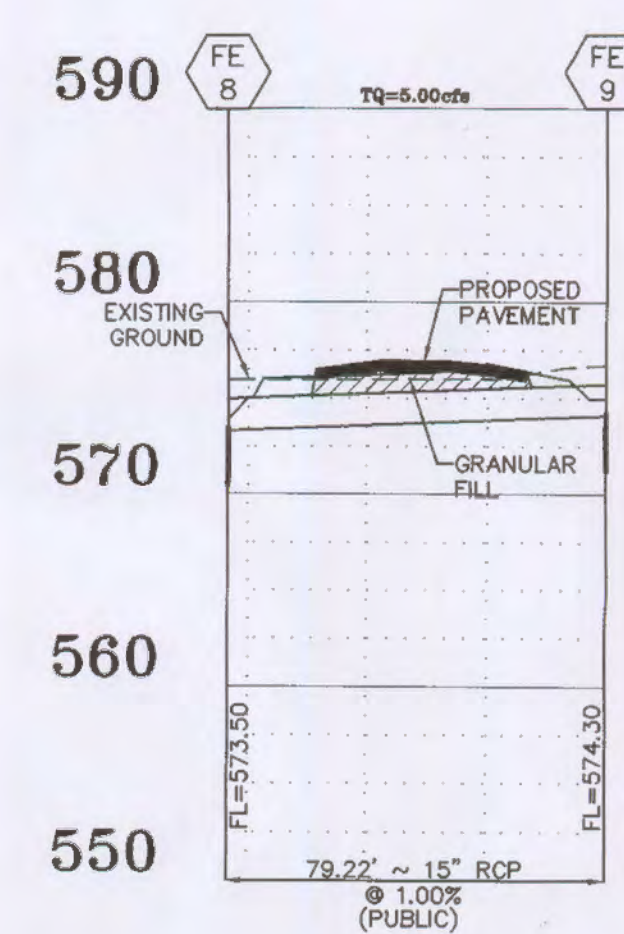
STORM SEWER PROFILE SCALES: HORIZ. 1"=40' VERT. 1"=10'
