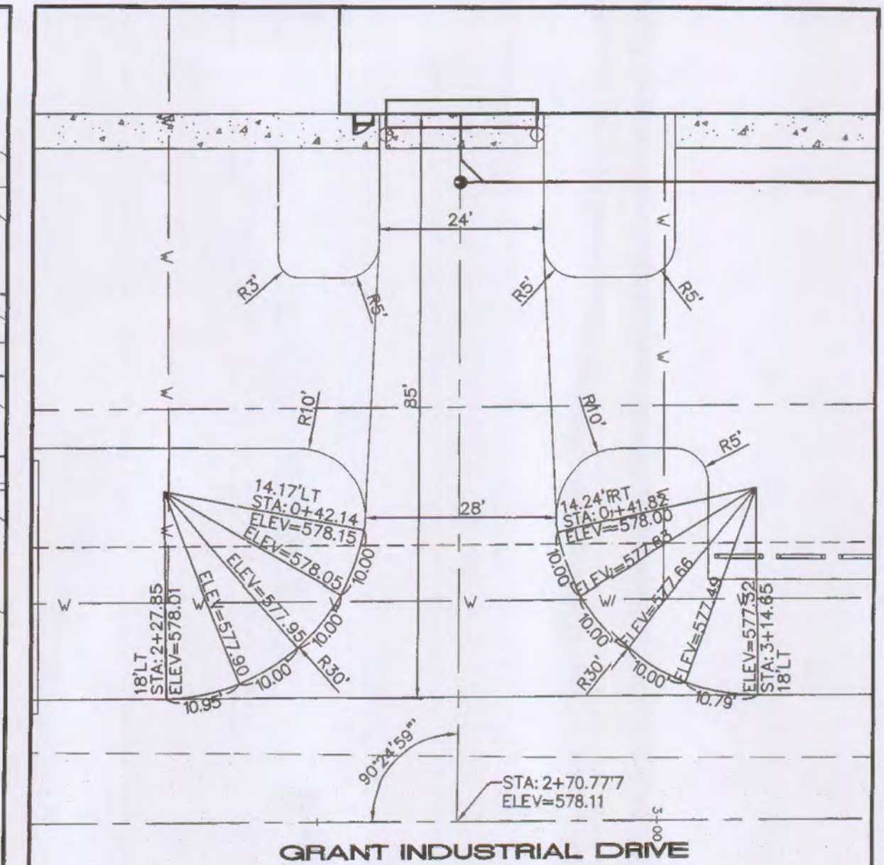
WEST ENTRANCE DETAIL SCALE: 1" = 20'
