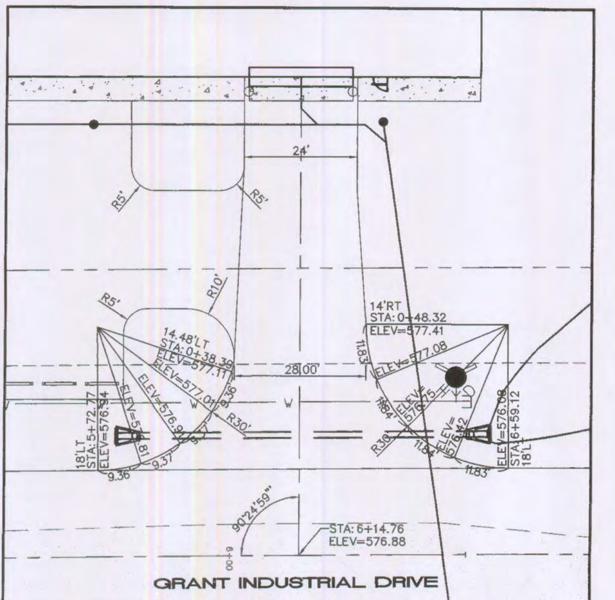
EAST ENTRANCE DETAIL SCALE: 1" = 20'
