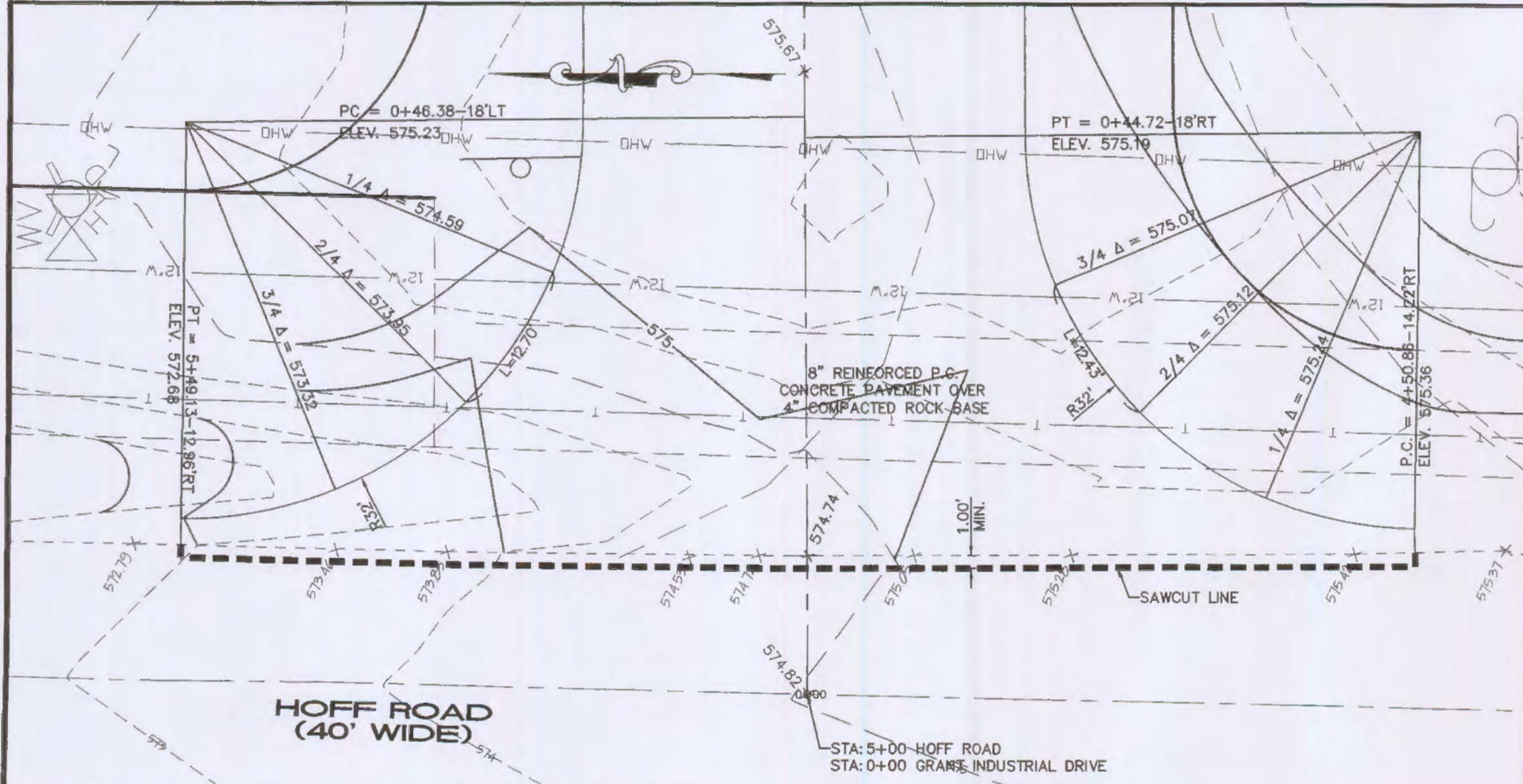
ROAD ENTRANCE DETAIL SCALE: 1" = 10'
