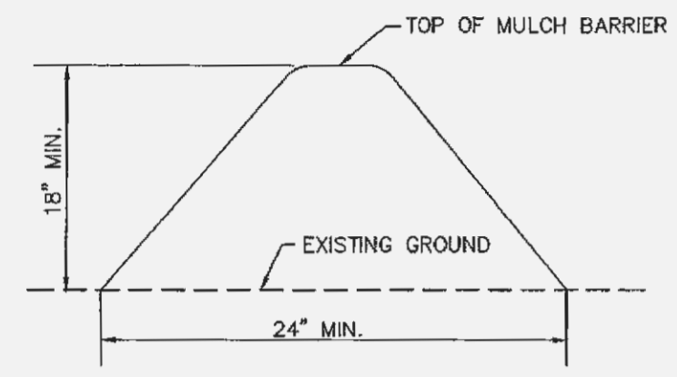
MULCH SEDIMENT BARRIER NOT TO SCALE
