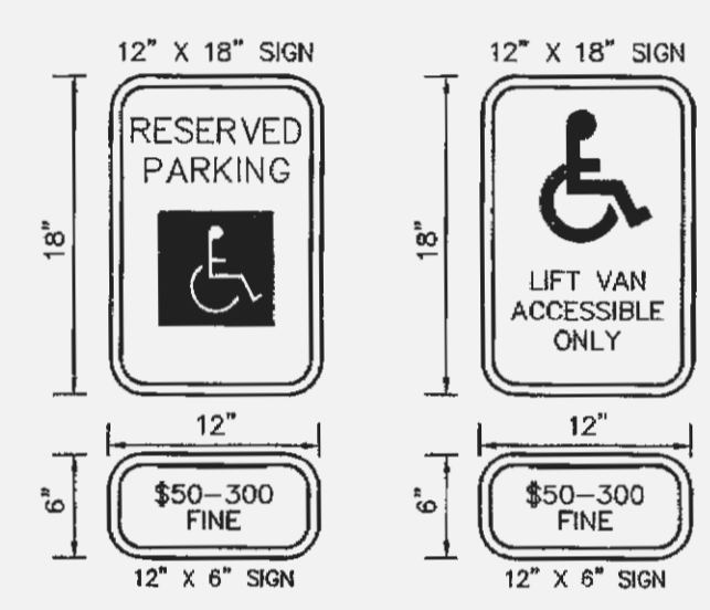
ACCESSIBLE PARKING SIGNS NOT TO SCALE
