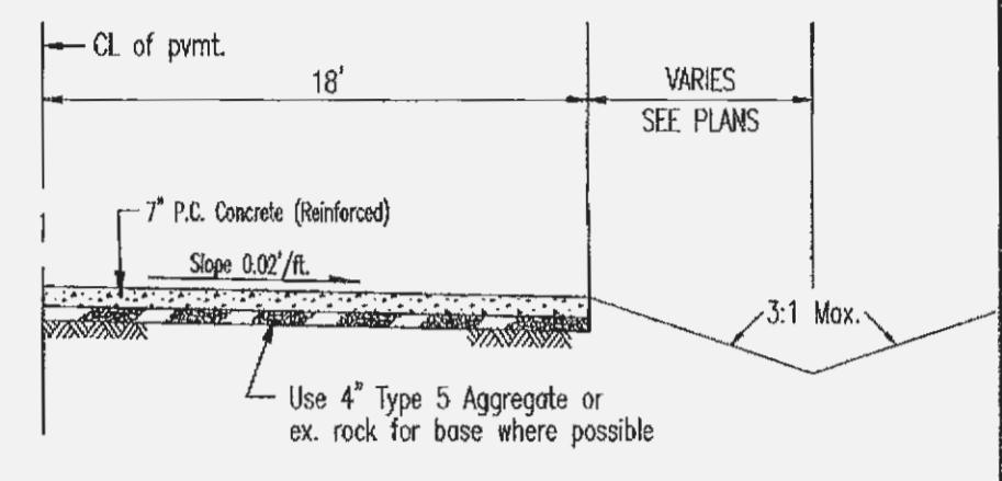
ROAD SECTION W/NO CURB
