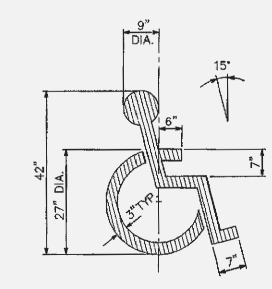
PAINTED ACCESSIBLE PARKING SYMBOL NOT TO SCALE
