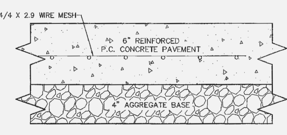
PARKING LOT PAVEMENT DETAIL NOT TO SCALE
