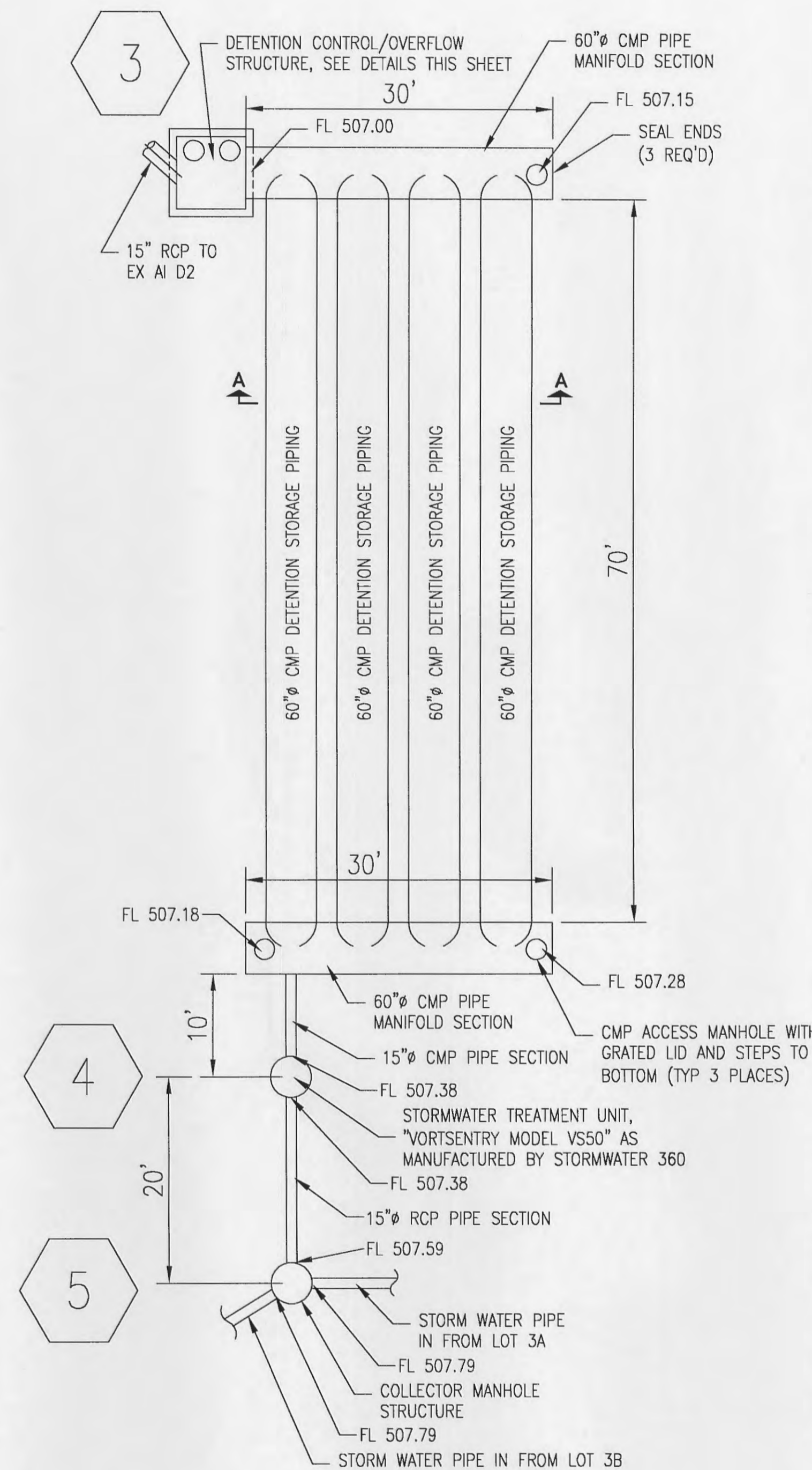
DETENTION PIPING LAYOUT DETAIL SCALE: 1"=10'
