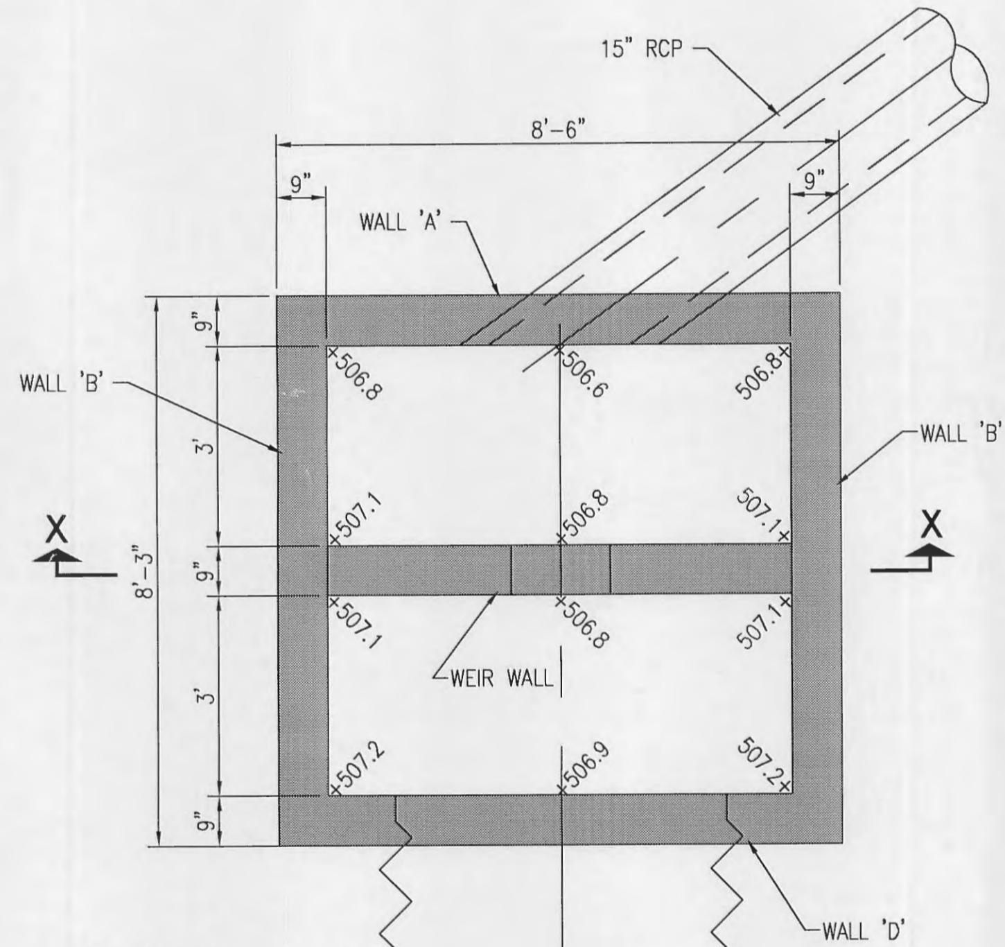
BOTTOM SLAB
