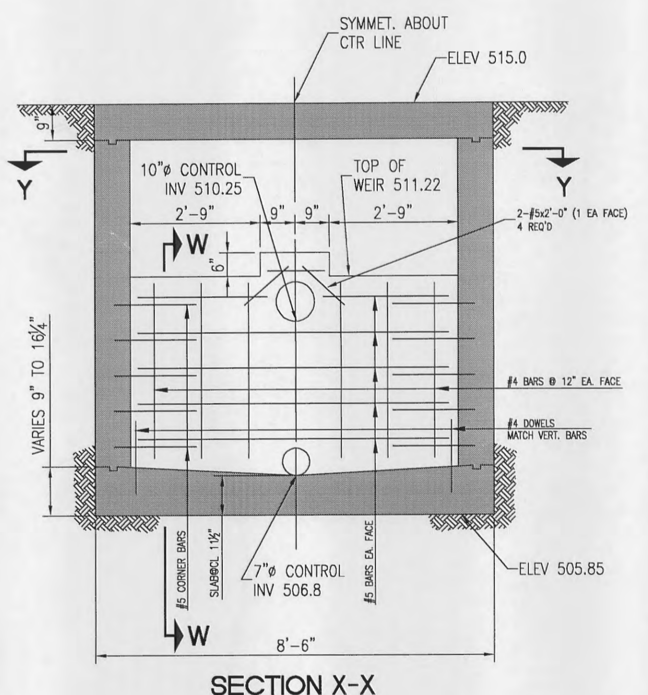
SECTION X-X
