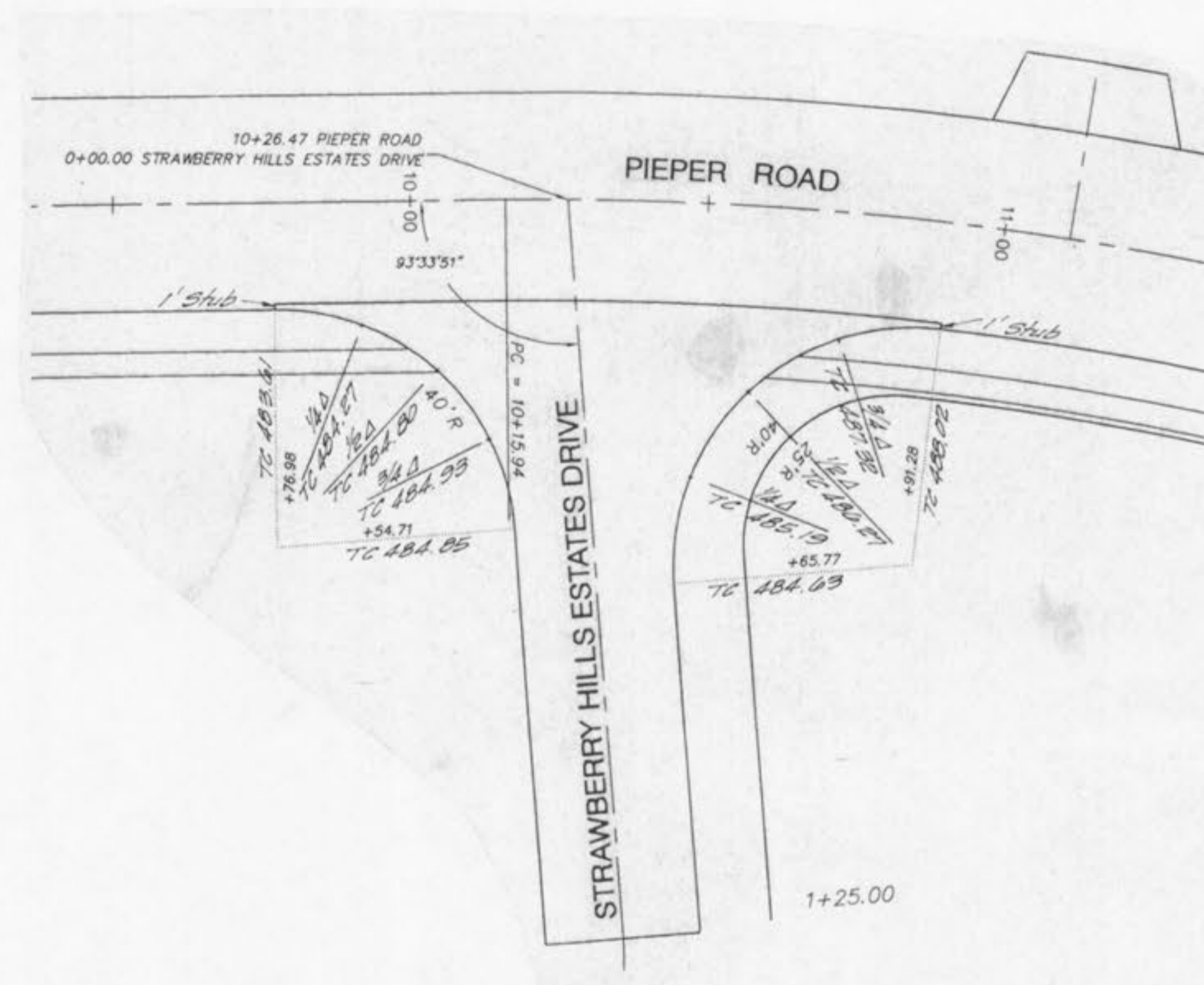
STRAWBERRY HILLS ESTATES DRIVE 1" = 20'
