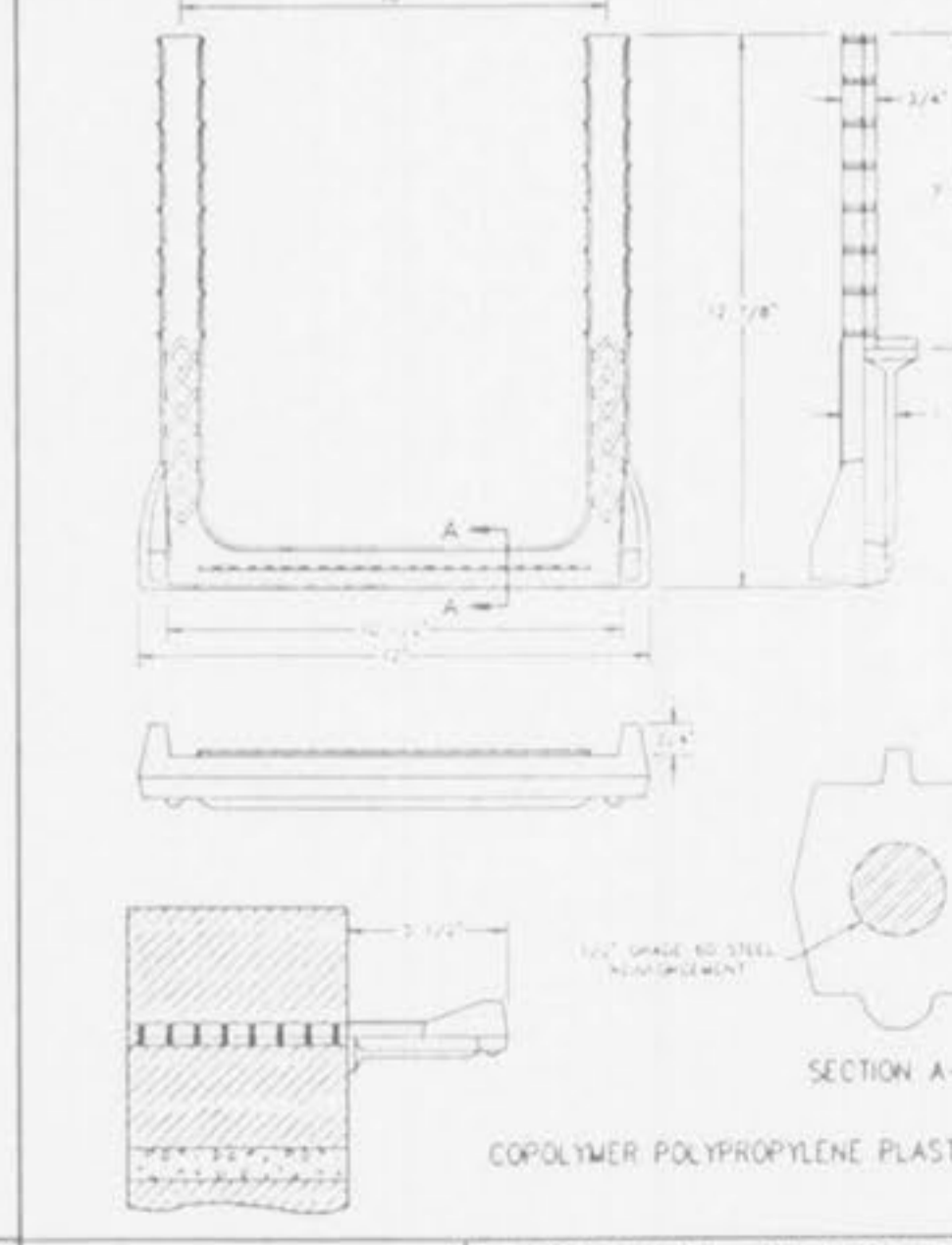
PSI-B MANHOLE STEP INTO JOINT METROPOLITAN ST. LOUIS SEWER DISTRICT Standard Details of Sewer Construction DI. H.C.W. CH. J.C.K. 1992 SHEET 53
