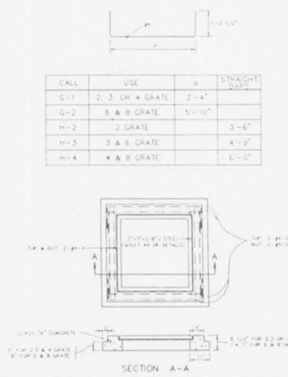
STEEL REQUIREMENTS FOR GRATE INLET SEAT METROPOLITAN ST. LOUIS SEWER DISTRICT Standard Details of Sewer Construction DI. H.C.W. CH. J.C.K. 1992 SHEET 46
