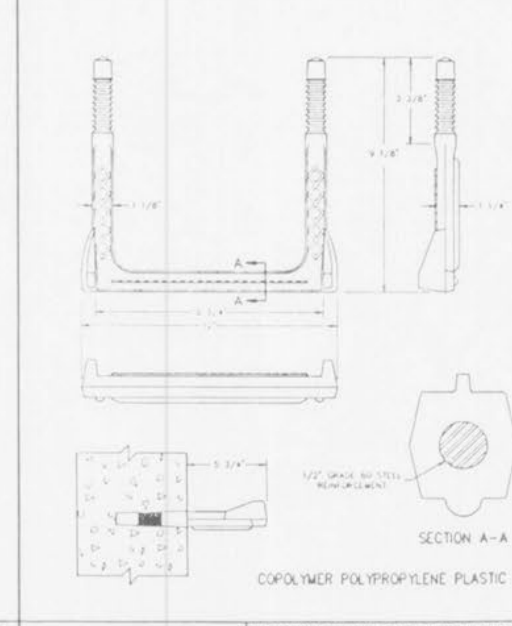
MANHOLE STEP FOR PRECAST MANHOLE METROPOLITAN ST. LOUIS SEWER DISTRICT Standard Details of Sewer Construction DI. D.A.B. CH. J.C.K. 1992 SHEET 54
