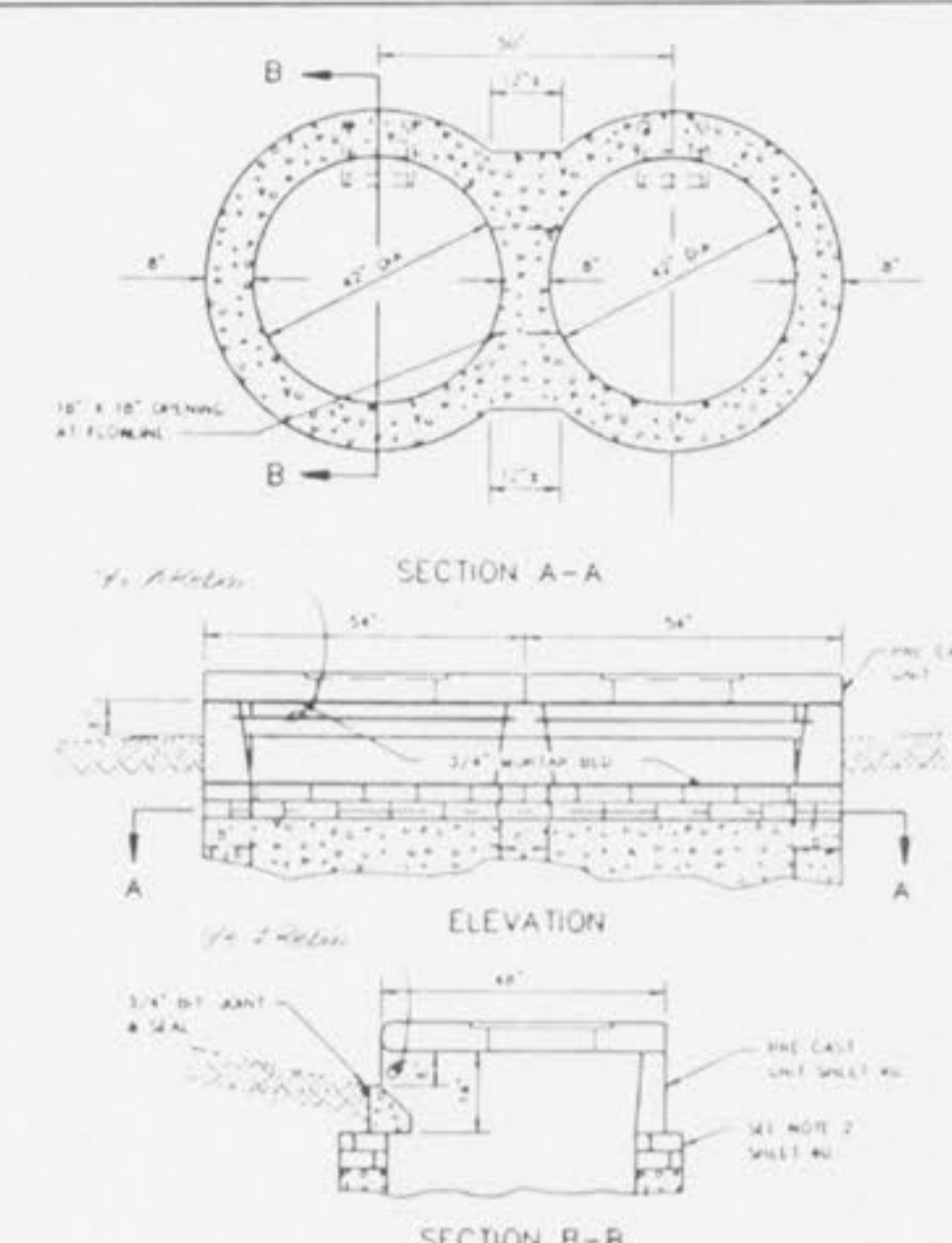
CONCRETE DOUBLE STREET INLET W/PRE CAST CONCRETE UNIT A METROPOLITAN ST. LOUIS SEWER DISTRICT Standard Details of Sewer Construction DI. H.C.W. CH. J.C.K. 1992 SHEET 39
