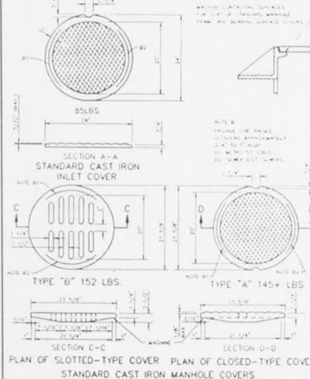
CAST IRON COVERS, MANHOLES AND INLETS METROPOLITAN ST. LOUIS SEWER DISTRICT Standard Details of Sewer Construction DI. H.C.W. CH. J.C.K. 1992 SHEET 49
