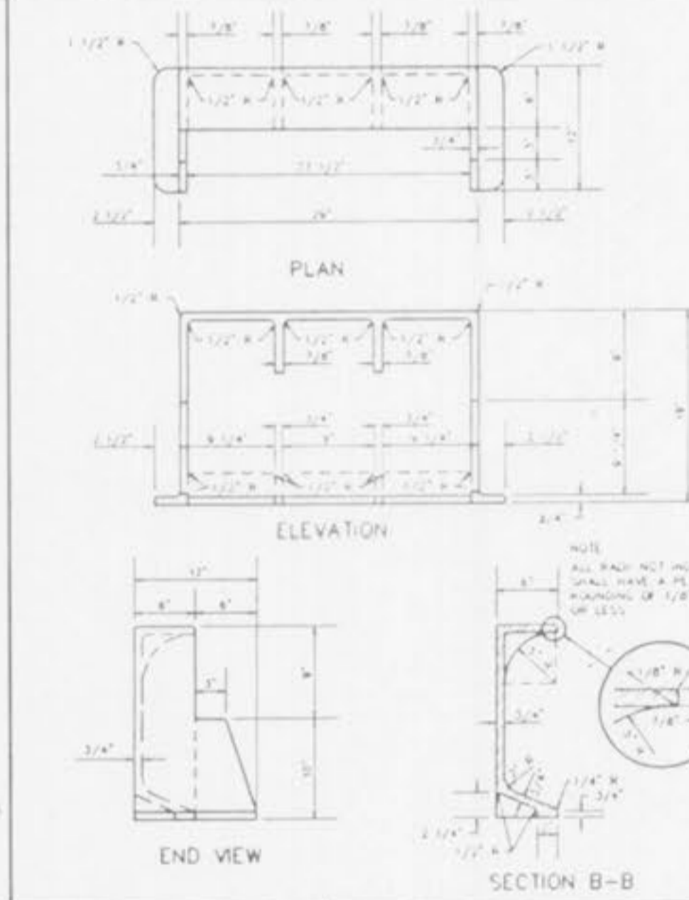
CAST IRON SIDE INTAKE UNIT FOR GRATED INLETS 249 LBS METROPOLITAN ST. LOUIS SEWER DISTRICT Standard Details of Sewer Construction DI. H.C.W. CH. J.C.K. 1992 SHEET 47
