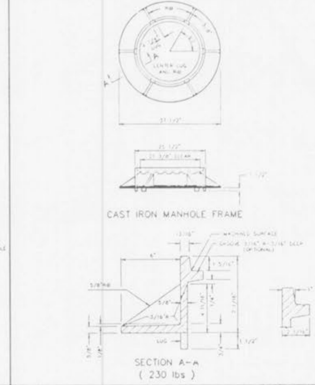
CAST IRON MANHOLE FRAME METROPOLITAN ST. LOUIS SEWER DISTRICT Standard Details of Sewer Construction DI. D.A.B. CH. J.C.K. 1992 SHEET 48
