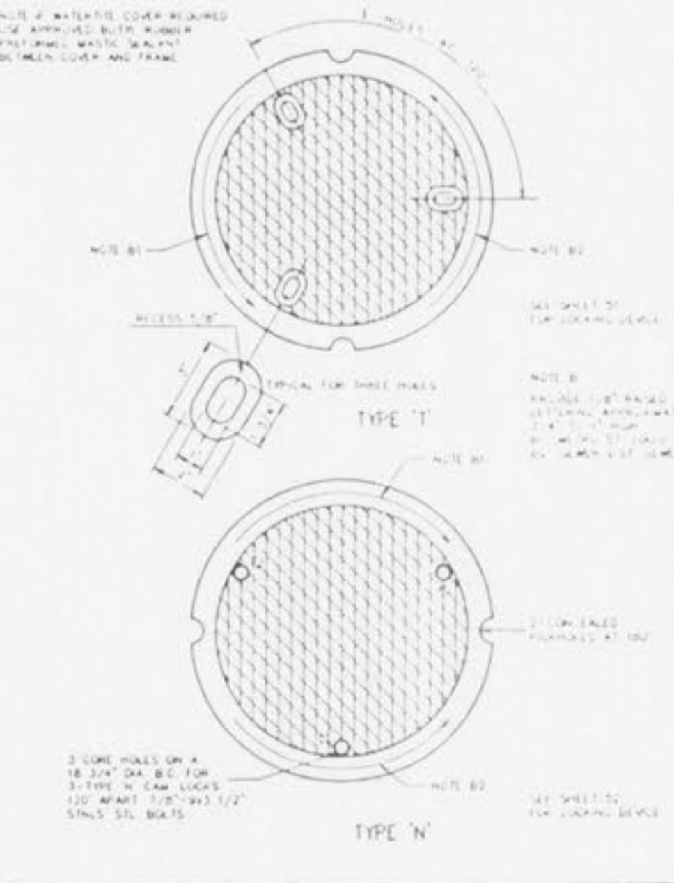
CAST IRON MANHOLE COVERS (LOCK TYPE) METROPOLITAN ST. LOUIS SEWER DISTRICT Standard Details of Sewer Construction DI. H.C.W. CH. J.C.K. 1992 SHEET 50
