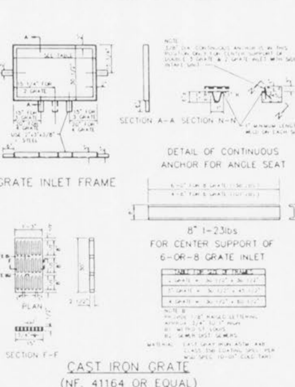
DETAILS OF INLET FRAME AND GRATES METROPOLITAN ST. LOUIS SEWER DISTRICT Standard Details of Sewer Construction DI. H.C.W. CH. J.C.K. 1992 SHEET 44
