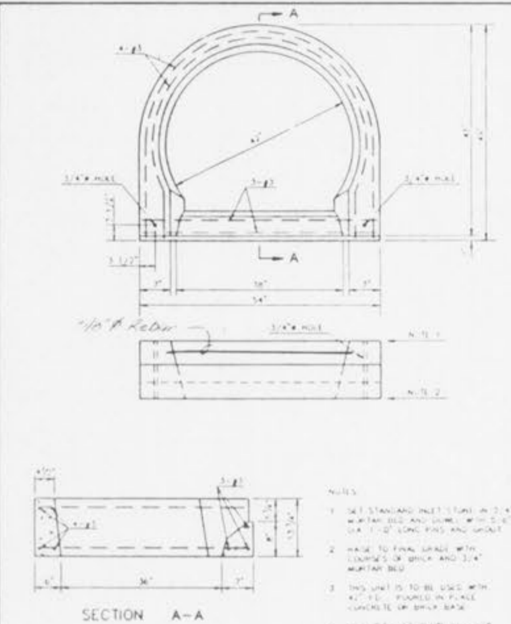
PRE-CAST CONCRETE UNIT FOR SINGLE STREET INLET METROPOLITAN ST. LOUIS SEWER DISTRICT Standard Details of Sewer Construction DI. H.C.W. CH. J.C.K. 1992 SHEET 37
