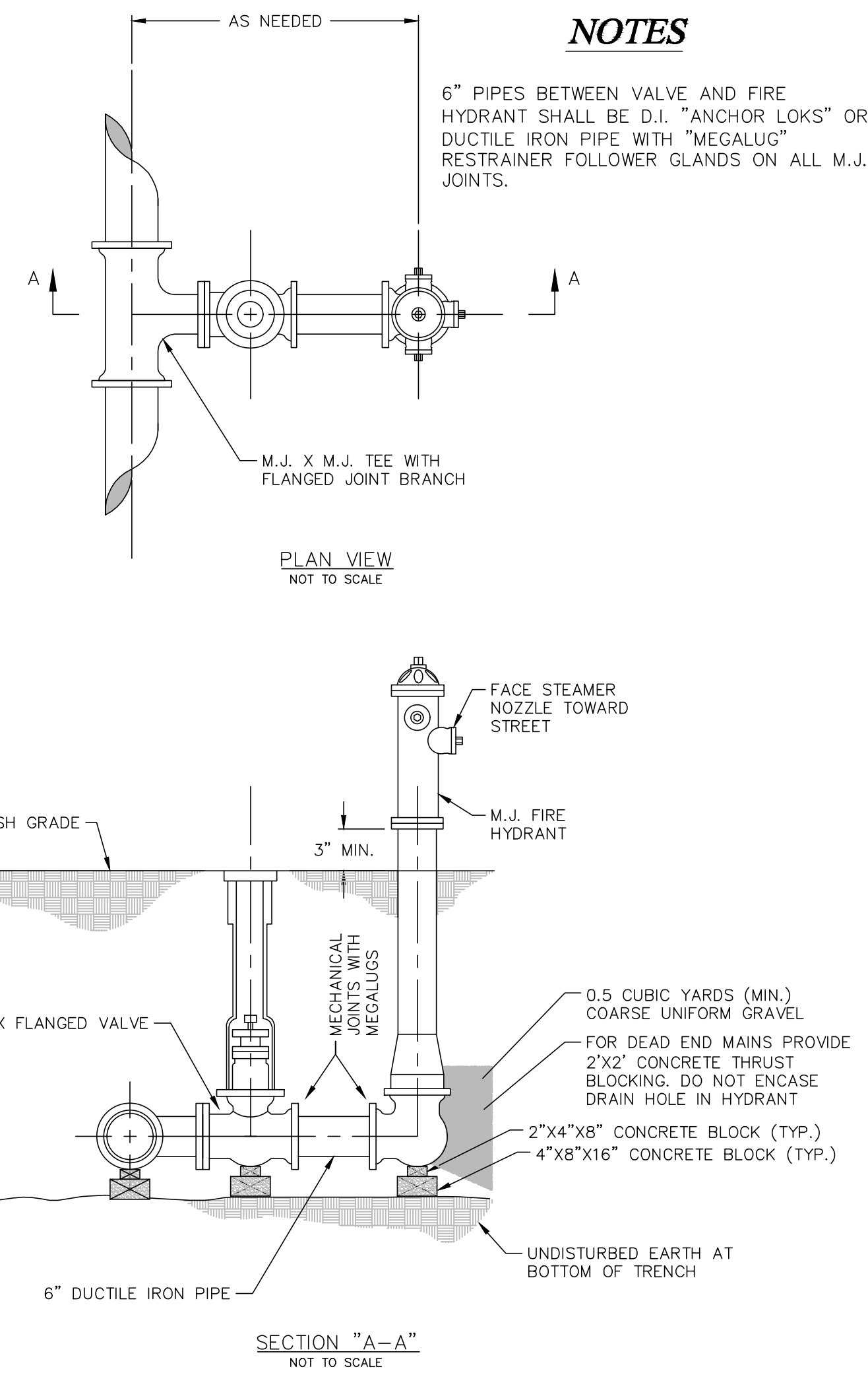
FIRE HYDRANT DETAIL DETAIL "B" PAGE 1 OF 3
