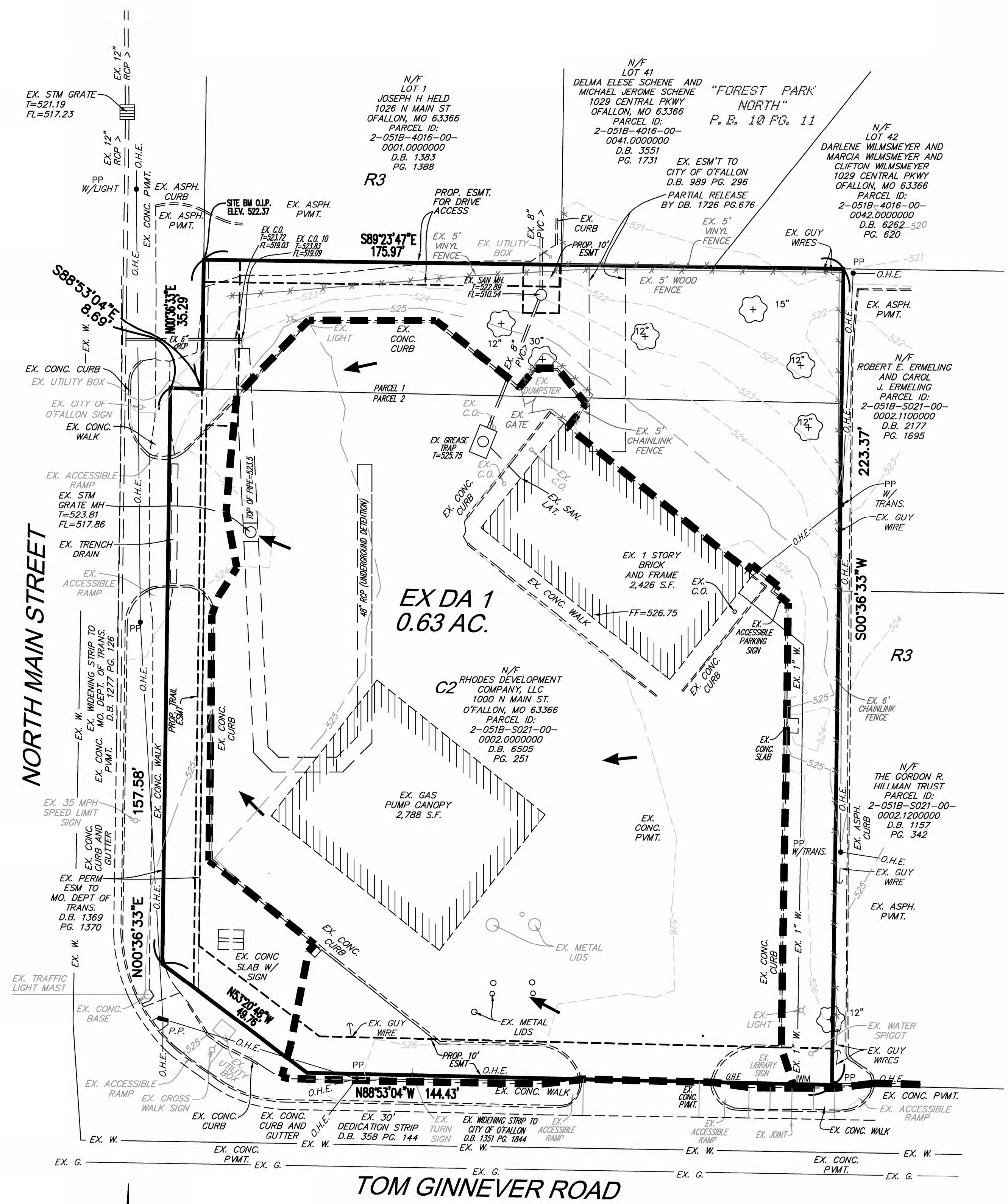
EXISTING DRAINAGE AREA MAP
