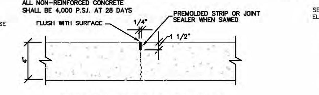
TYPICAL CONSTRUCTION JOINT TYPE C (4\"/>
