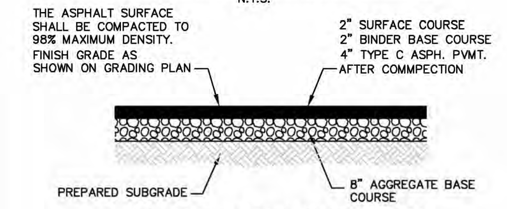
ASPHALT PAVEMENT DETAIL (FOR DRIVE ISLES ONLY) N.T.S.
