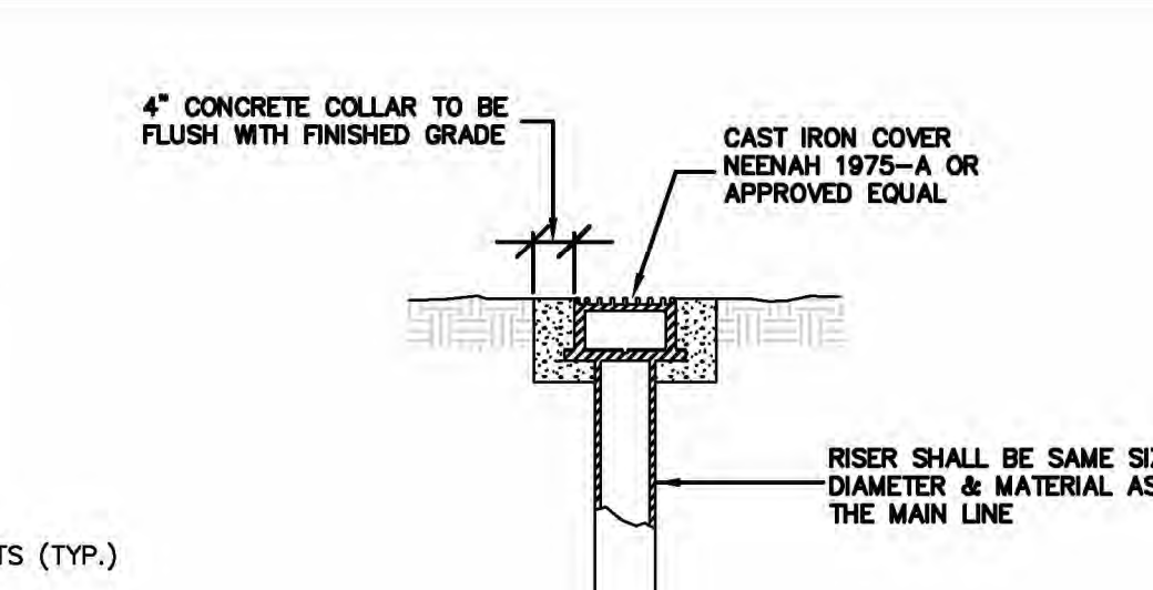
CLEAN OUT DETAIL (SANITARY SEWER ONLY) N.T.S.
