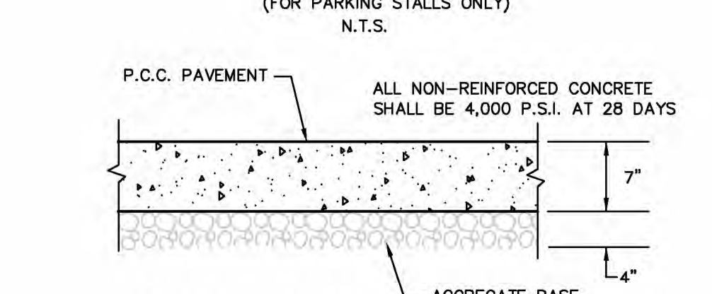
CONCRETE PAVEMENT SECTION @ TRASH ENCLOSURE AND DRIVE THRU AISLE N.T.S.
