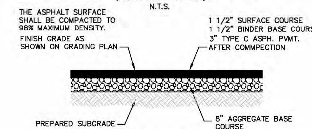
ASPHALT PAVEMENT DETAIL (FOR PARKING STALLS ONLY) N.T.S.
