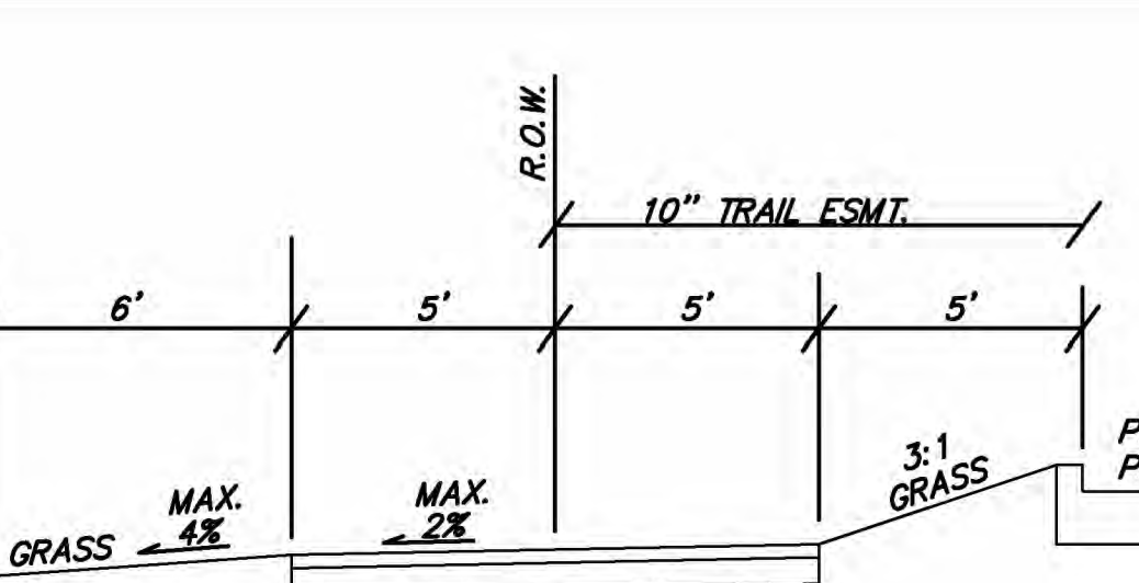
TRAIL DETAIL SCALE: 1"=4'
