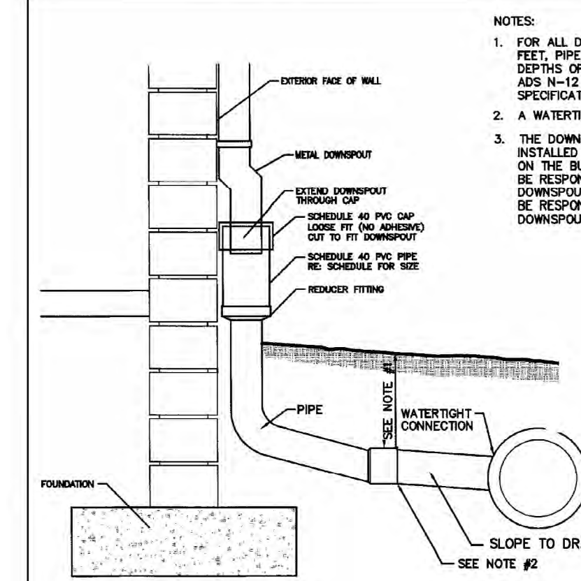
DOWNSPOUT COLLECTOR DETAIL NO SCALE
