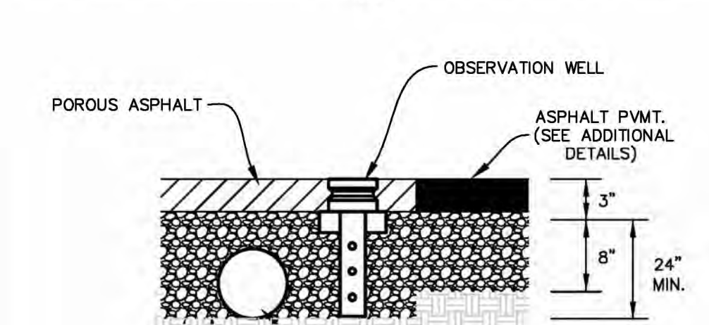
POROUS ASPHALT PAVEMENT TYPICAL SECTION N.T.S.
