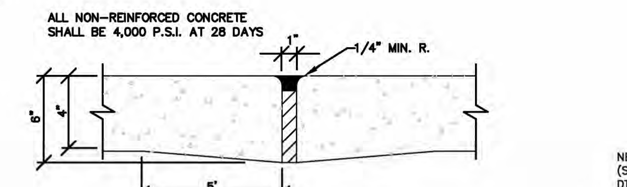
TYPICAL EXPANSION JOINT TYPE A (4\"/>
