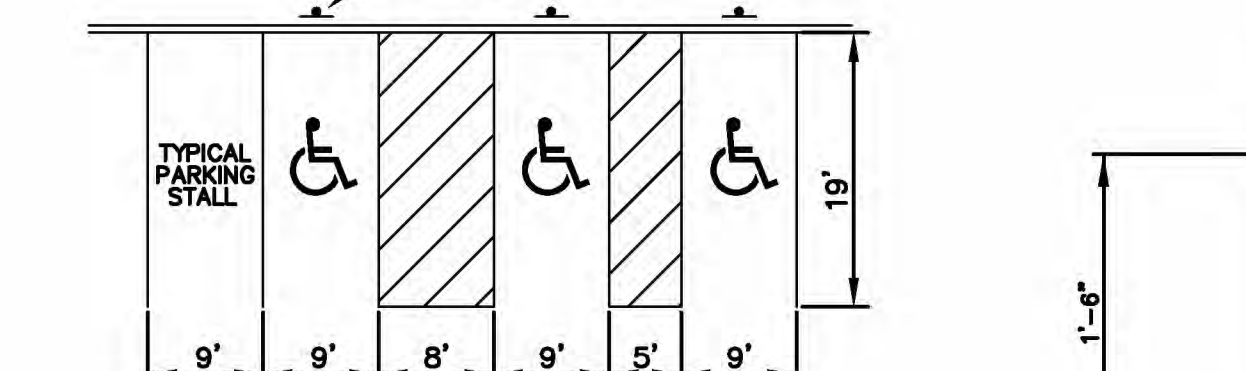
TYPICAL PARKING SPACE N.T.S.
