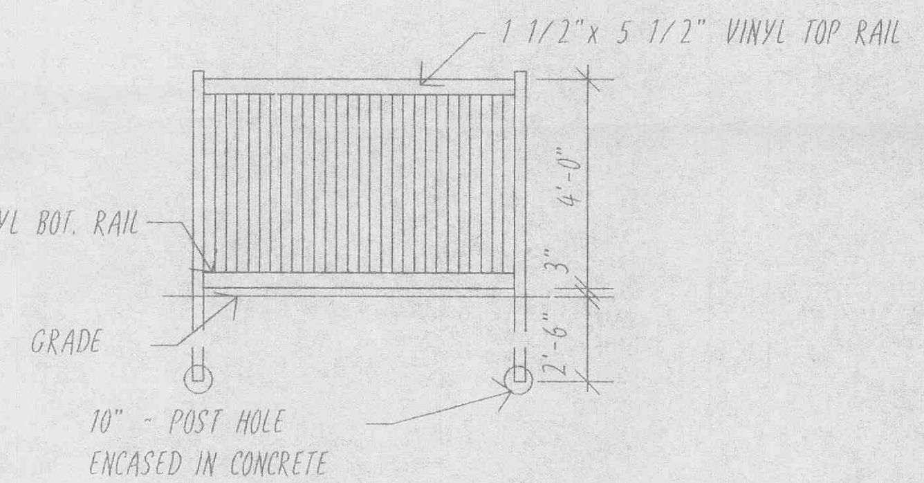
SIDE & REAR ELEVATION
