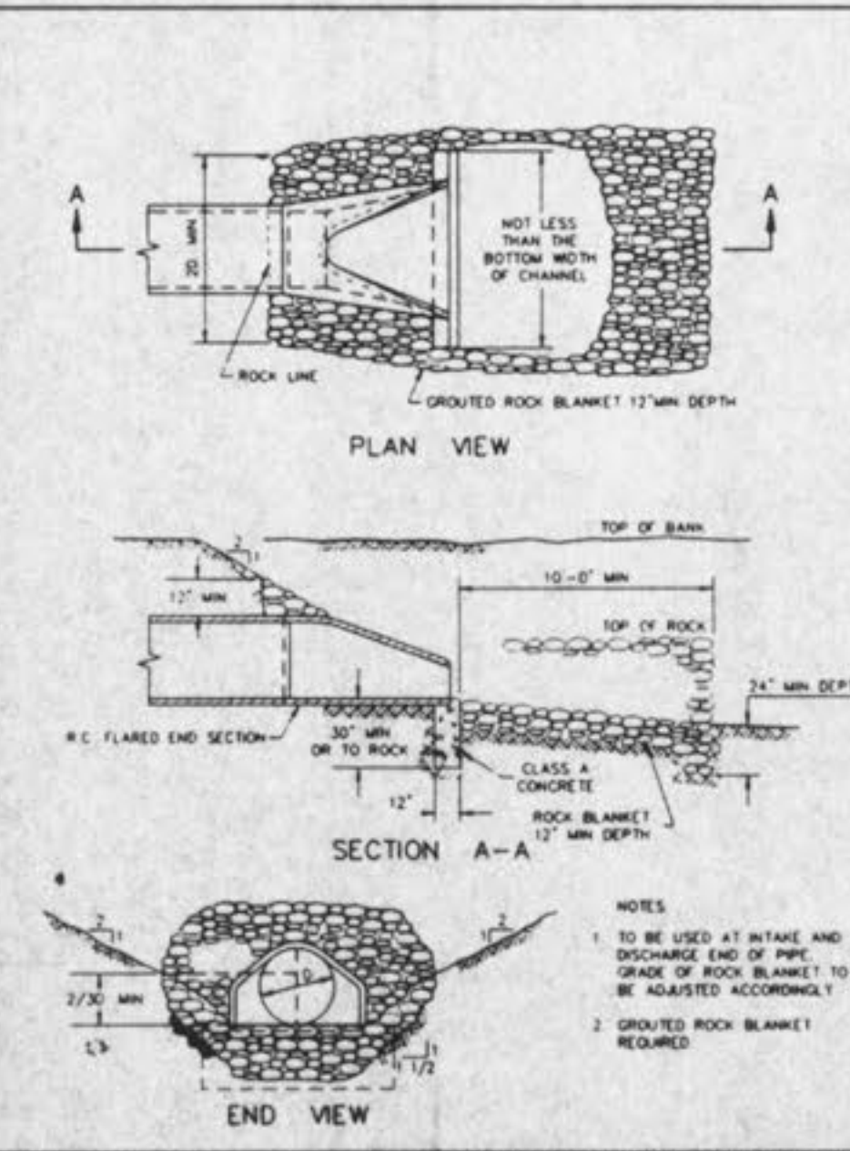
FLARED END SECTION METROPOLITAN ST. LOUIS SEWER DISTRICT Standard Details of Sewer Construction Dr. W.S.H. 1992 SHEET 57
