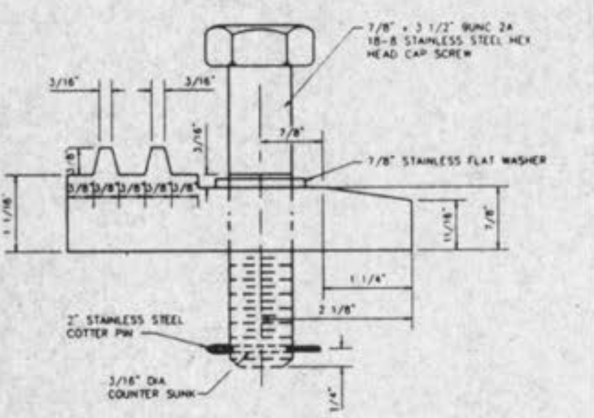
LOCKING DEVICE FOR TYPE 'I' LOCK TYPE MANHOLE COVER METROPOLITAN ST. LOUIS SEWER DISTRICT Standard Details of Sewer Construction Dr. R.G.W. 1992 SHEET 51
