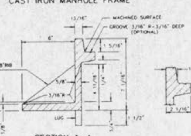
CAST IRON MANHOLE FRAME METROPOLITAN ST. LOUIS SEWER DISTRICT Standard Details of Sewer Construction Dr. D.A.B. 1992 SHEET 48
