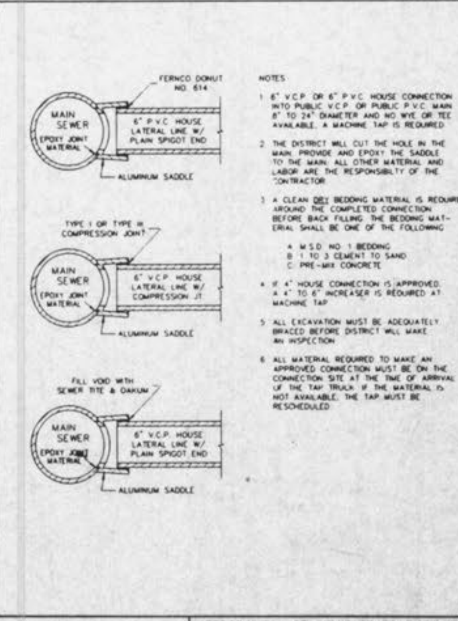
MACHINE TAP METROPOLITAN ST. LOUIS SEWER DISTRICT Standard Details of Sewer Construction Dr. W.S.H. 1992 SHEET 60
