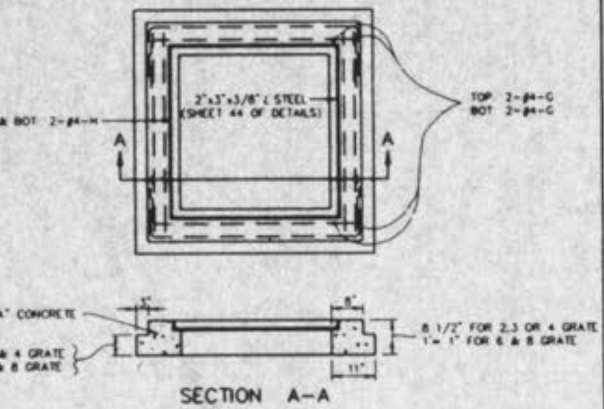
STEEL REQUIREMENTS FOR GRATE INLET SEAT METROPOLITAN ST. LOUIS SEWER DISTRICT Standard Details of Sewer Construction Dr. W.S.H. 1992 SHEET 46
