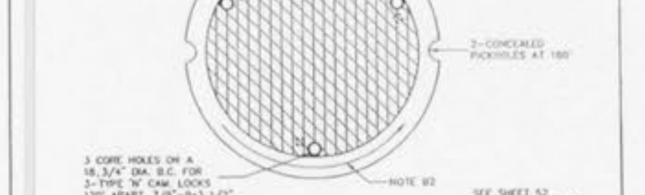
CAST IRON MANHOLE COVER (LOCK TYPE) METROPOLITAN ST. LOUIS SEWER DISTRICT Standard Details of Sewer Construction Dr. R.G.W. 1992 SHEET 50
