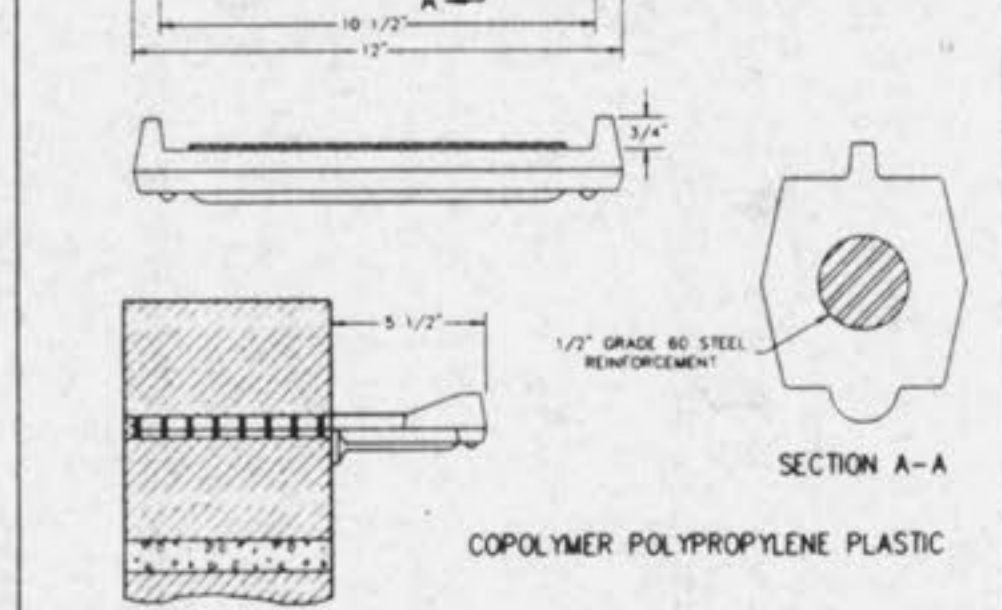
PSI-B MANHOLE STEP INTO JOINT METROPOLITAN ST. LOUIS SEWER DISTRICT Standard Details of Sewer Construction Dr. W.S.H. 1992 SHEET 53
