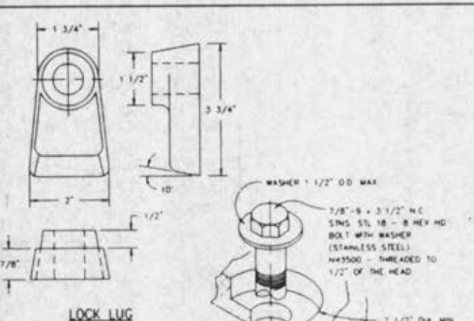
CAST IRON SIDE INTAKE UNIT FOR GRATED INLETS 249 LBS. METROPOLITAN ST. LOUIS SEWER DISTRICT Standard Details of Sewer Construction Dr. R.G.W. 1992 SHEET 47
