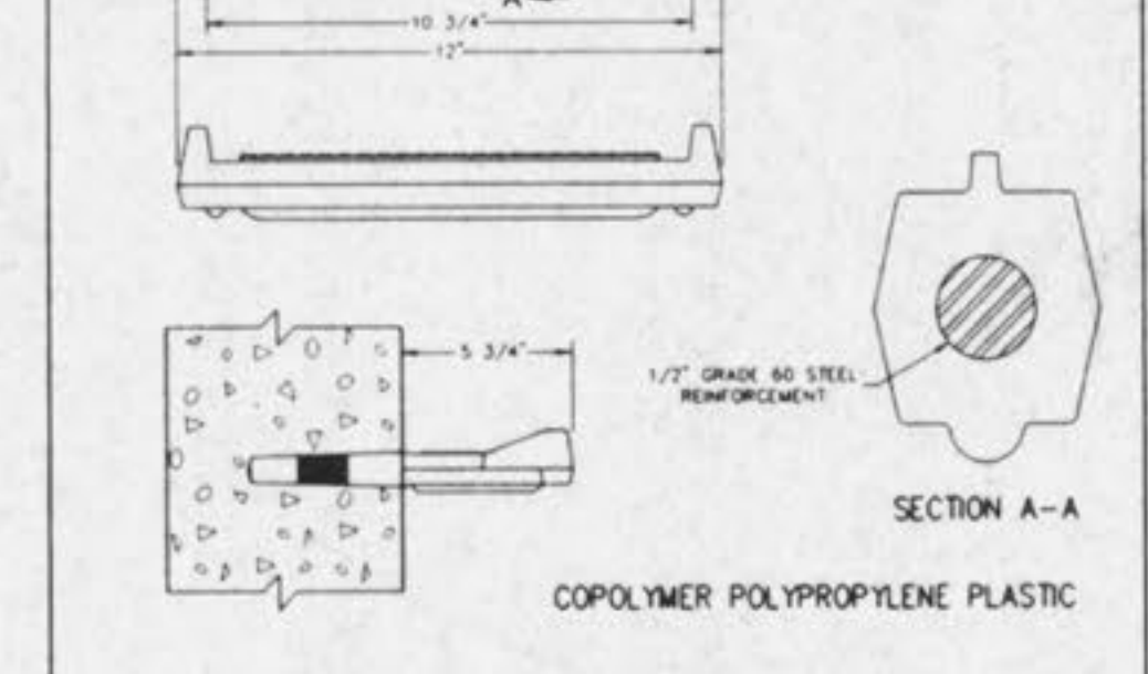
MANHOLE STEP FOR PRECAST MANHOLE METROPOLITAN ST. LOUIS SEWER DISTRICT Standard Details of Sewer Construction Dr. D.A.B. 1992 SHEET 54
