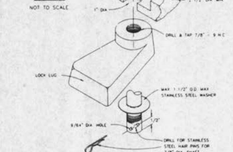
LOCKING DEVICE FOR TYPE 'N' LOCK TYPE MANHOLE COVER METROPOLITAN ST. LOUIS SEWER DISTRICT Standard Details of Sewer Construction Dr. J.L.G. 1992 SHEET 52
