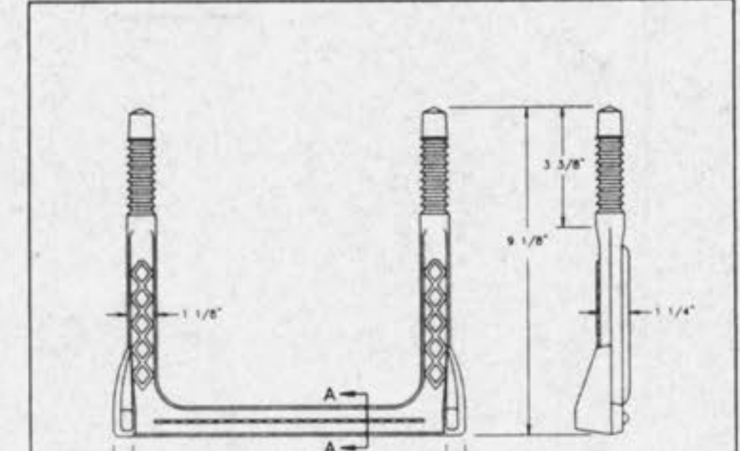
CAST IRON COVERS MANHOLES AND INLETS METROPOLITAN ST. LOUIS SEWER DISTRICT Standard Details of Sewer Construction Dr. R.G.W. 1992 SHEET 49
