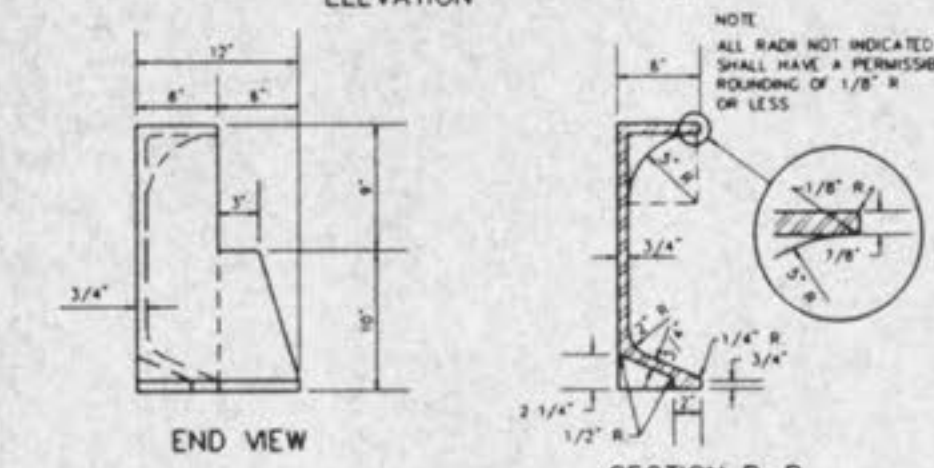
CAST IRON SIDE INTAKE UNIT FOR GRATED INLETS 249 LBS. METROPOLITAN ST. LOUIS SEWER DISTRICT Standard Details of Sewer Construction Dr. R.G.W. 1992 SHEET 47
