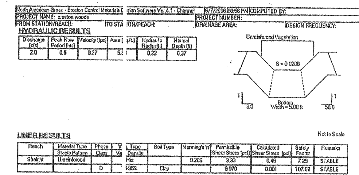
SECTION "10-10"
