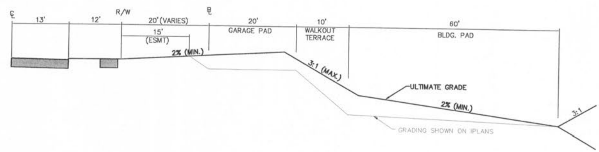
TYPICAL SINGLE FAMILY WALKOUT LOT TEMPLATE
