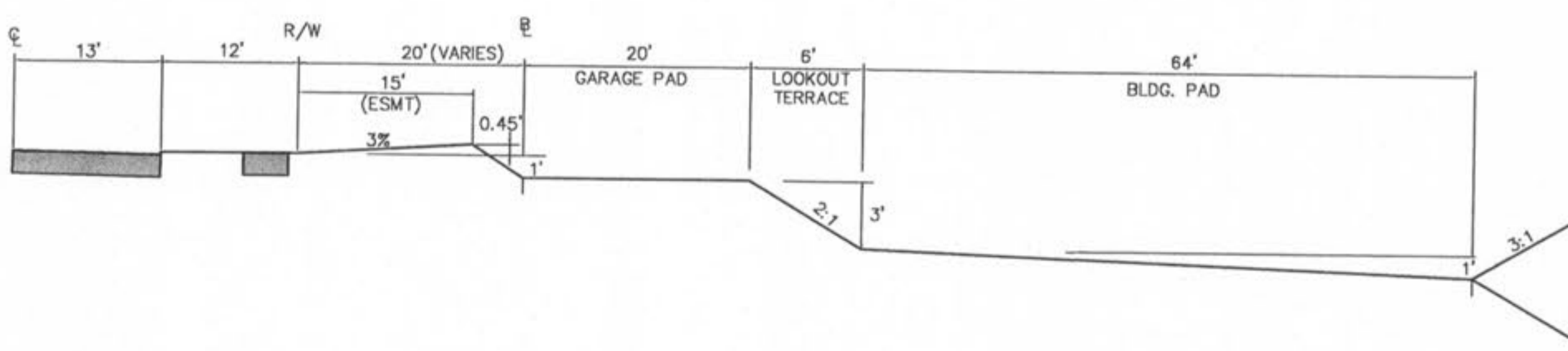
TYPICAL SINGLE FAMILY LOOKOUT LOT TEMPLATE
