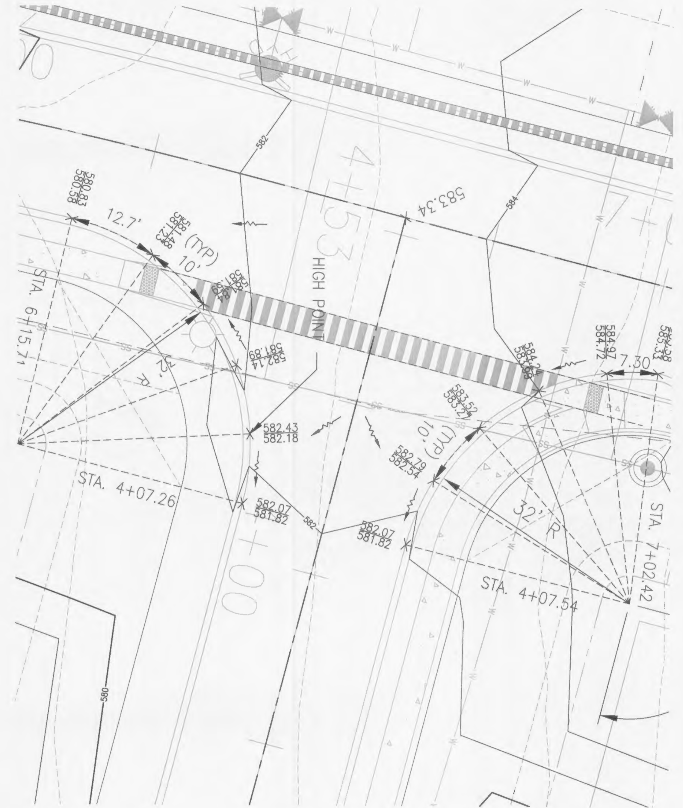
2 LYNWOOD RIDGE AND SOUTHERN MAGNOLIA SCALE: - REF. DWG.
