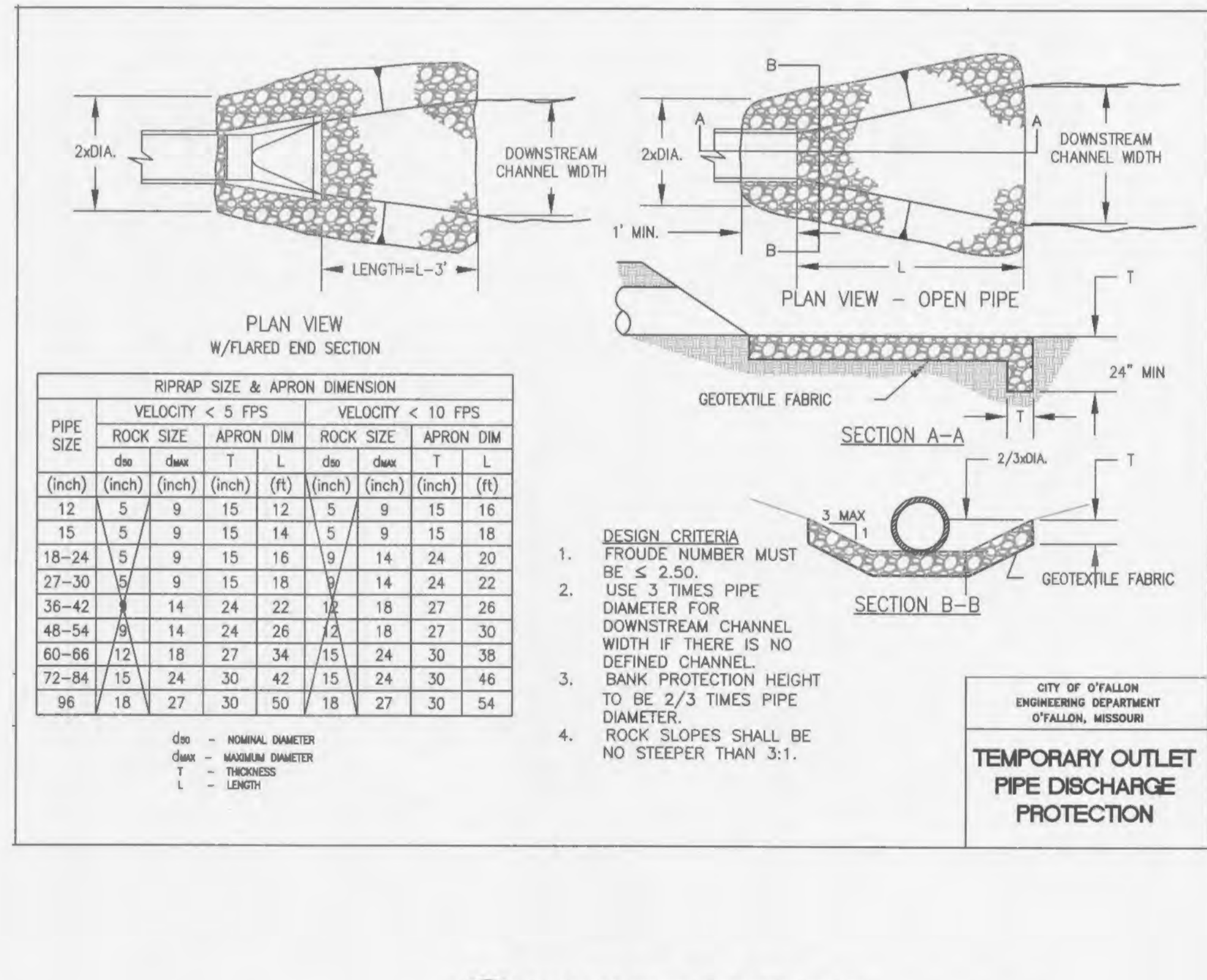
1 STORM PIPE DISCHARGE SCALE: NTS REF. DWG.
