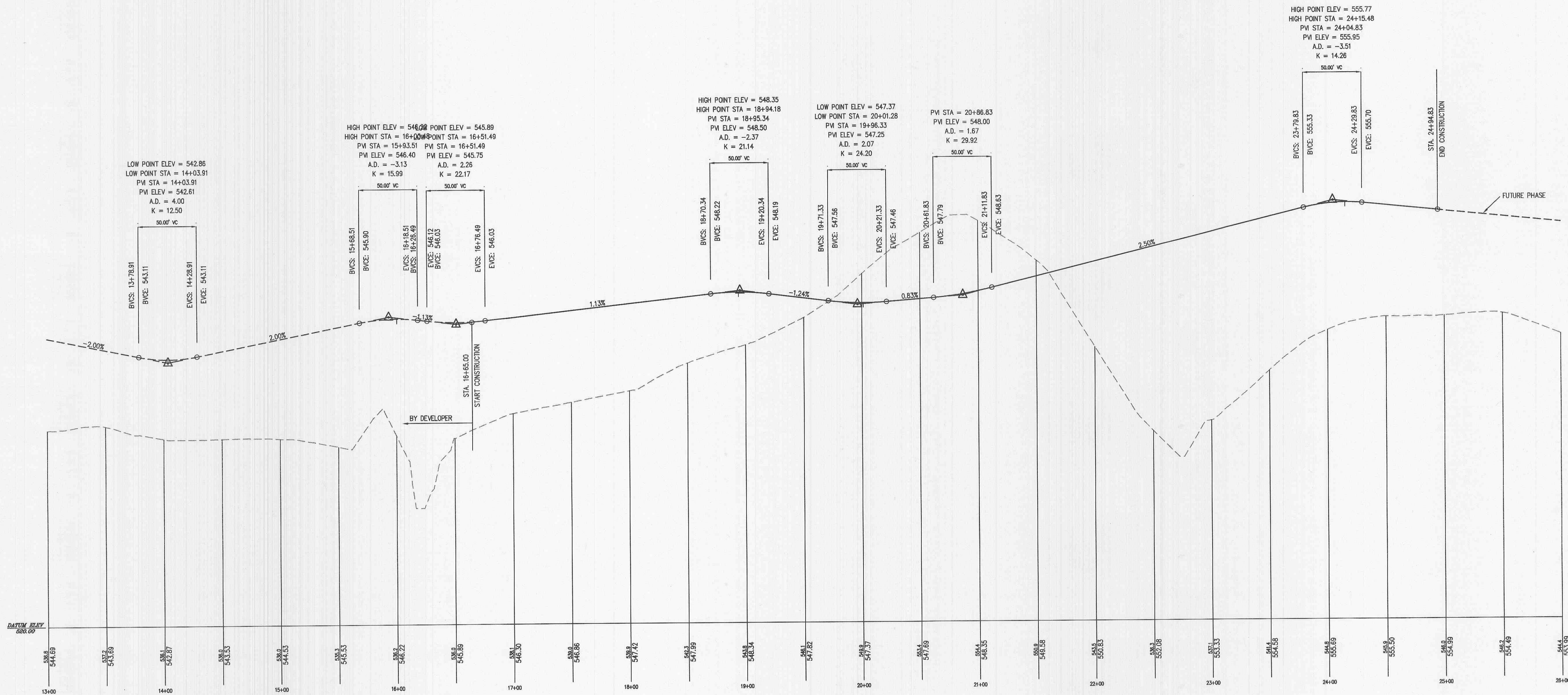
REAR ENTRY ROAD PROFILE
