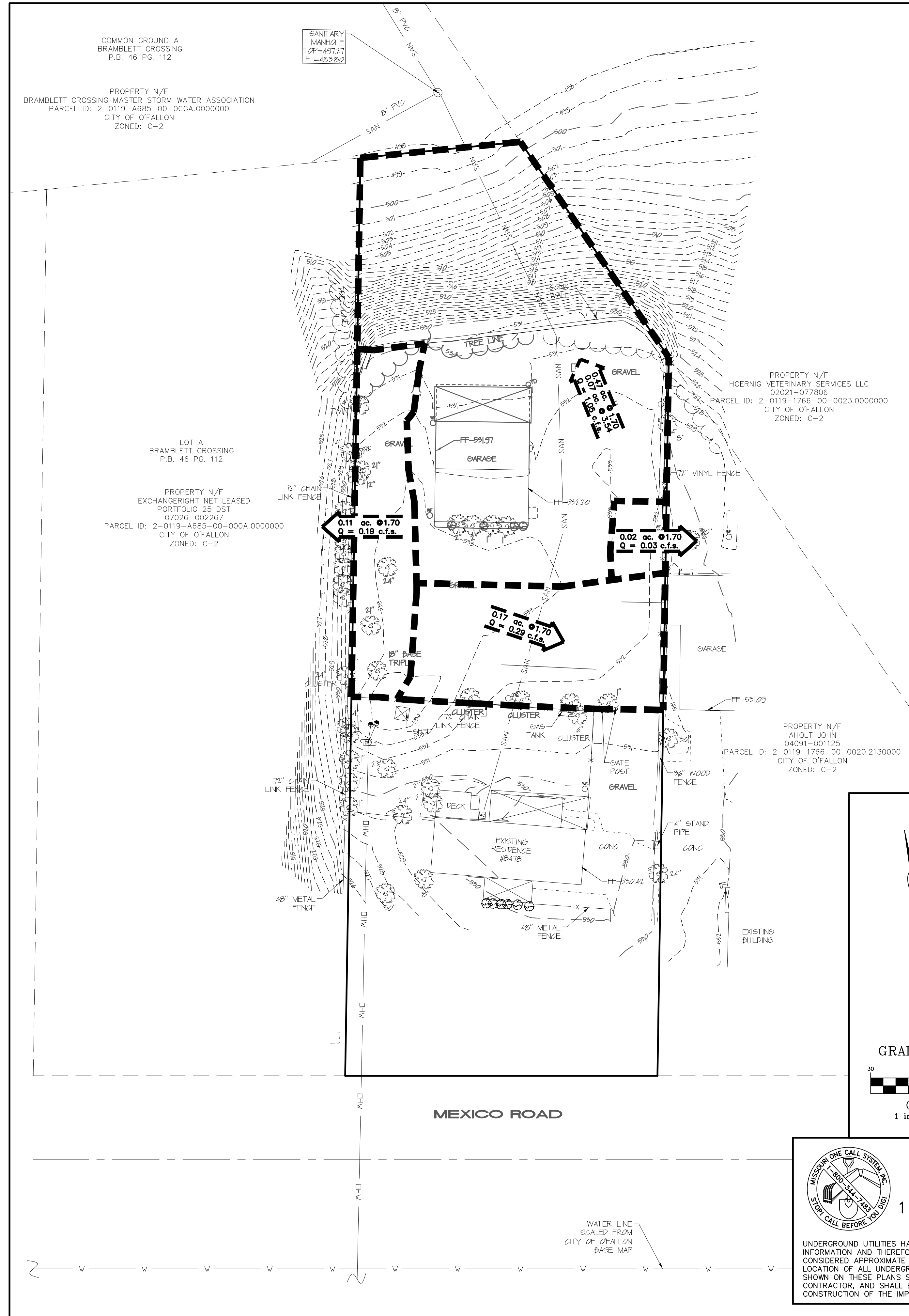
EXISTING DRAINAGE AREA MAP
