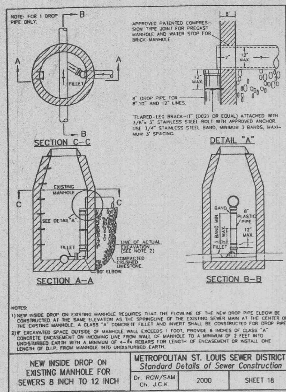
NEW INSIDE DROP ON EXISTING MANHOLE FOR 8 INCH TO 12 INCH METROPOLITAN ST. LOUIS SEWER DISTRICT Standard Details of Sewer Construction Dr. ROW/SAM Ch. J.C.K. 2000 SHEET 18
