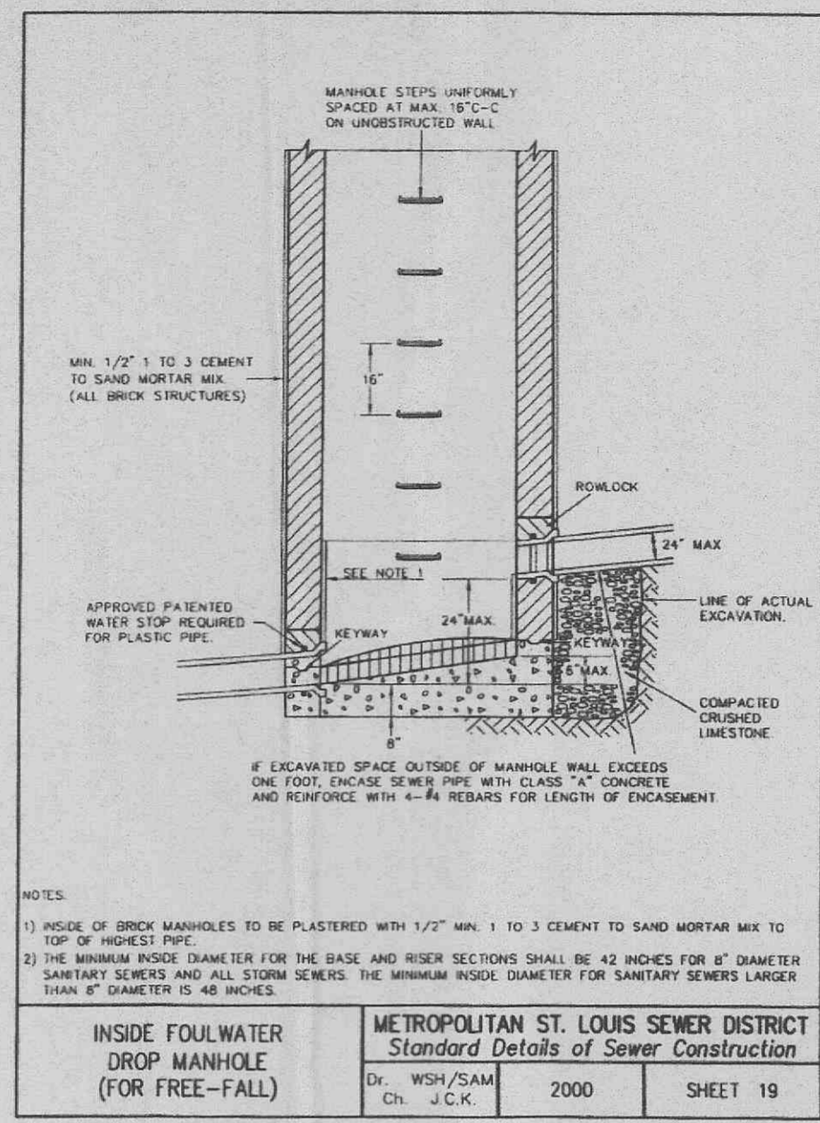
INSIDE FOULWATER DROP MANHOLE (FOR FREE-FALL) METROPOLITAN ST. LOUIS SEWER DISTRICT Standard Details of Sewer Construction Dr. WSH/SAM Ch. J.C.K. 2000 SHEET 19
