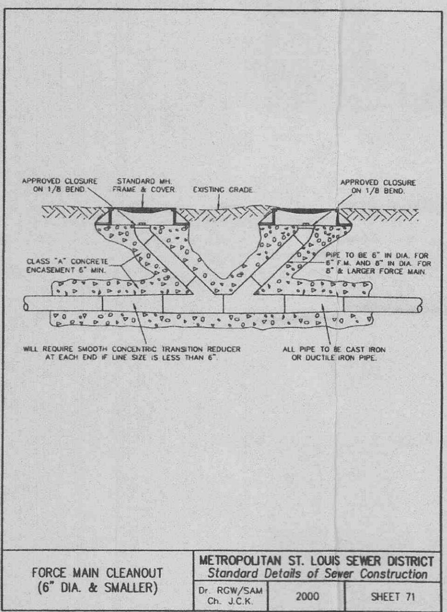
FORCE MAIN CLEANOUT (6" DIA. & SMALLER) METROPOLITAN ST. LOUIS SEWER DISTRICT Standard Details of Sewer Construction Dr. ROW/SAM Ch. J.C.K. 2000 SHEET 71
