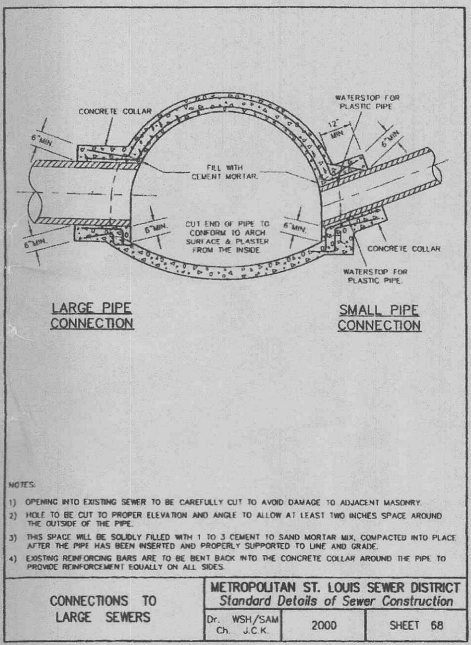
CONNECTIONS TO LARGE SEWERS METROPOLITAN ST. LOUIS SEWER DISTRICT Standard Details of Sewer Construction Dr. WSH/SAM Ch. J.C.K. 2000 SHEET 68
