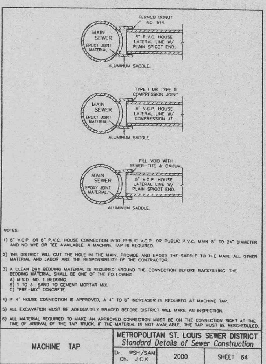
MACHINE TAP METROPOLITAN ST. LOUIS SEWER DISTRICT Standard Details of Sewer Construction Dr. WSH/SAM Ch. J.C.K. 2000 SHEET 64
