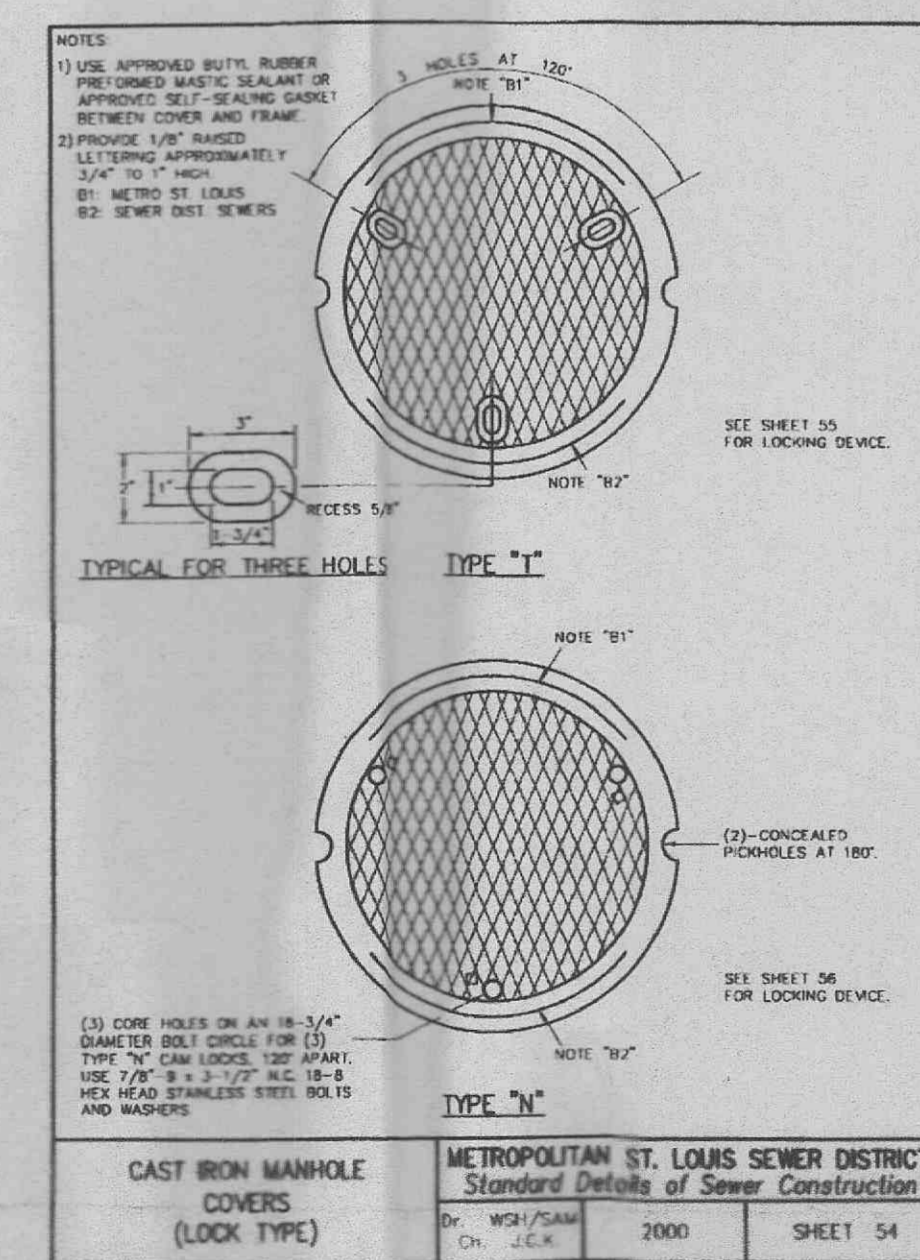
CAST IRON MANHOLE COVERS (LOCK TYPE) METROPOLITAN ST. LOUIS SEWER DISTRICT Standard Details of Sewer Construction Dr. WSH/SAM Ch. J.C.K. 2000 SHEET 54
