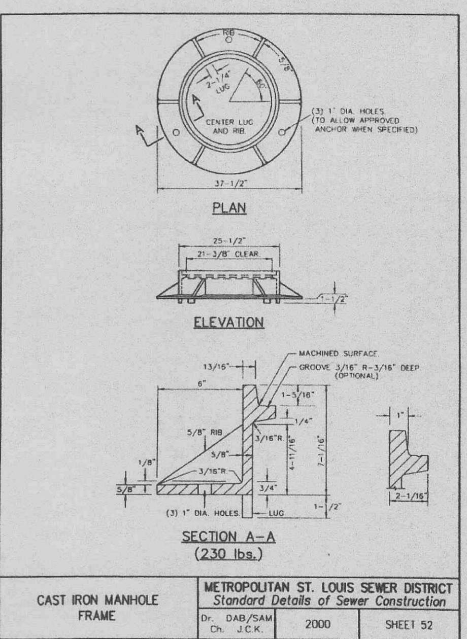
CAST IRON MANHOLE FRAME METROPOLITAN ST. LOUIS SEWER DISTRICT Standard Details of Sewer Construction Dr. DAB/SAM Ch. J.C.K. 2000 SHEET 52
