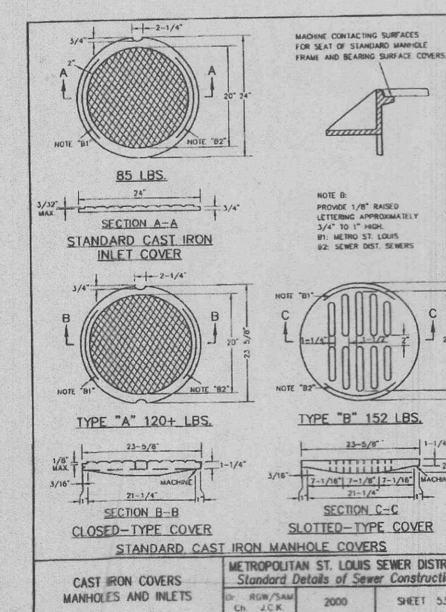
CAST IRON COVERS MANHOLES AND INLETS METROPOLITAN ST. LOUIS SEWER DISTRICT Standard Details of Sewer Construction Dr. ROW/SAM Ch. J.C.K. 2000 SHEET 53
