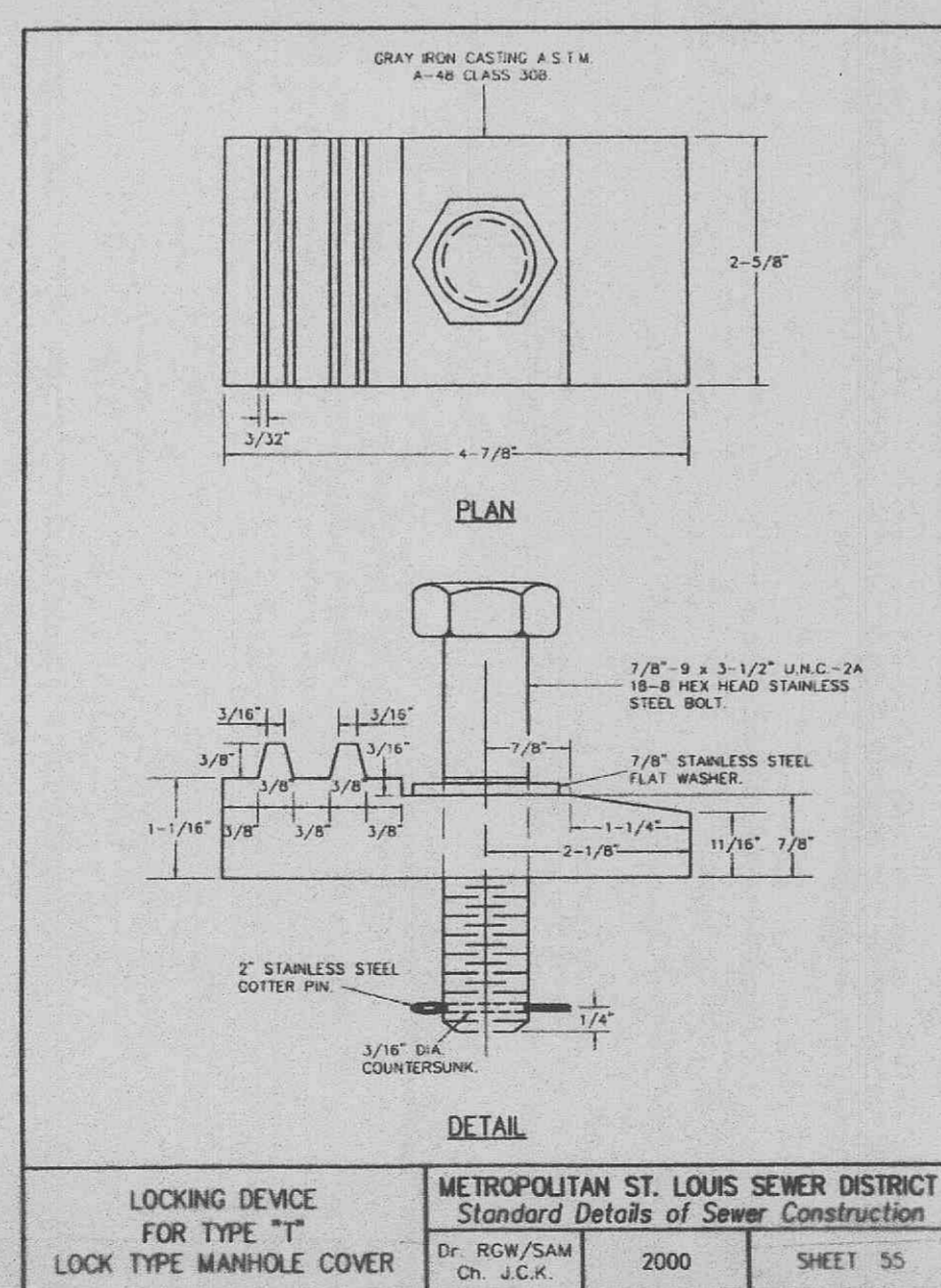
LOCKING DEVICE FOR TYPE "T" LOCK TYPE MANHOLE COVER METROPOLITAN ST. LOUIS SEWER DISTRICT Standard Details of Sewer Construction Dr. ROW/SAM Ch. J.C.K. 2000 SHEET 55
