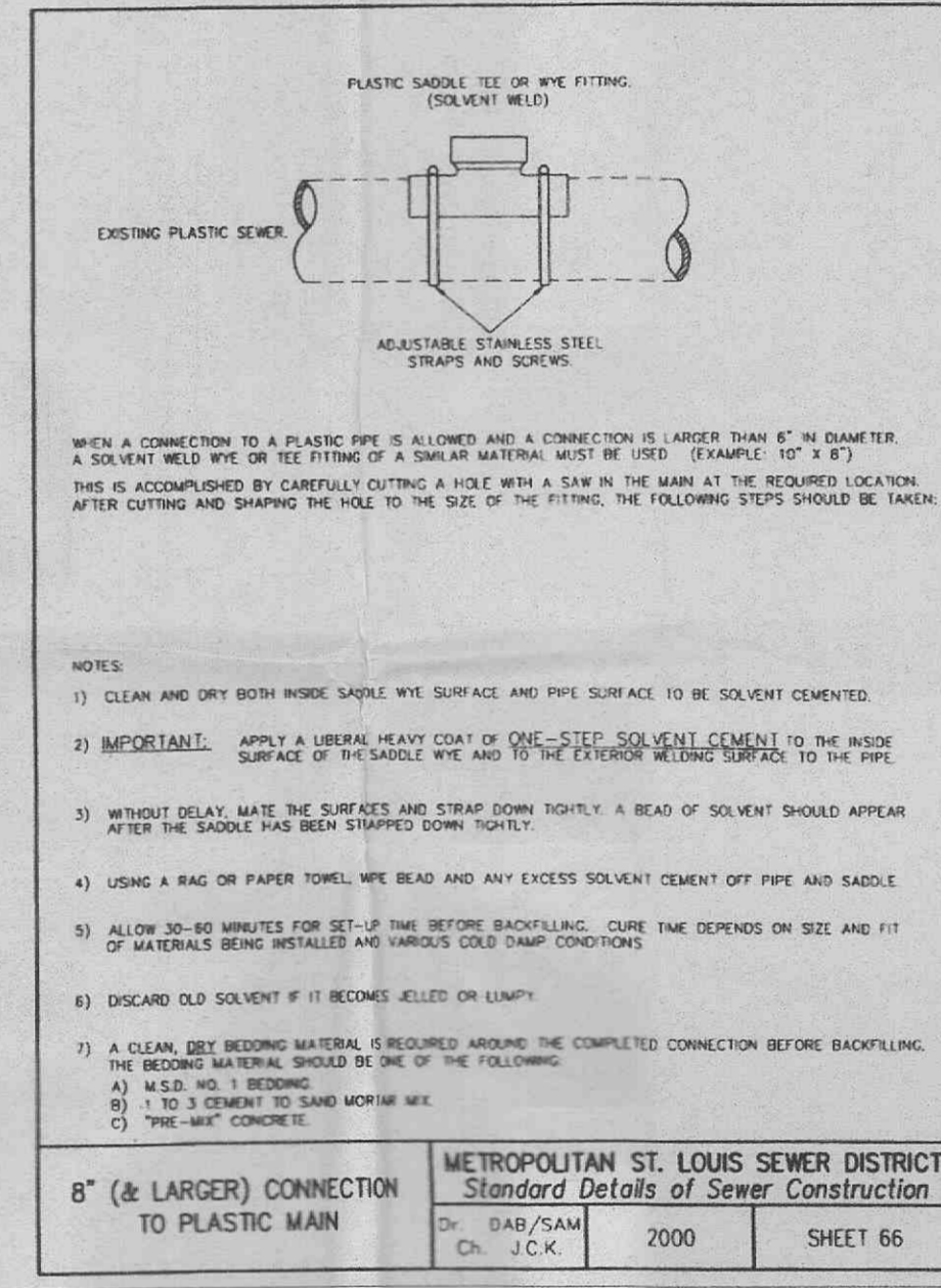
8" (& LARGER) CONNECTION TO PLASTIC MAIN METROPOLITAN ST. LOUIS SEWER DISTRICT Standard Details of Sewer Construction Dr. DAB/SAM Ch. J.C.K. 2000 SHEET 66
