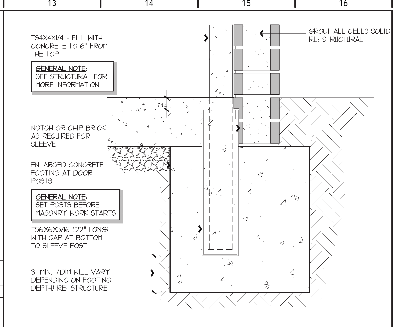
L13 DOOR POST DETAIL
