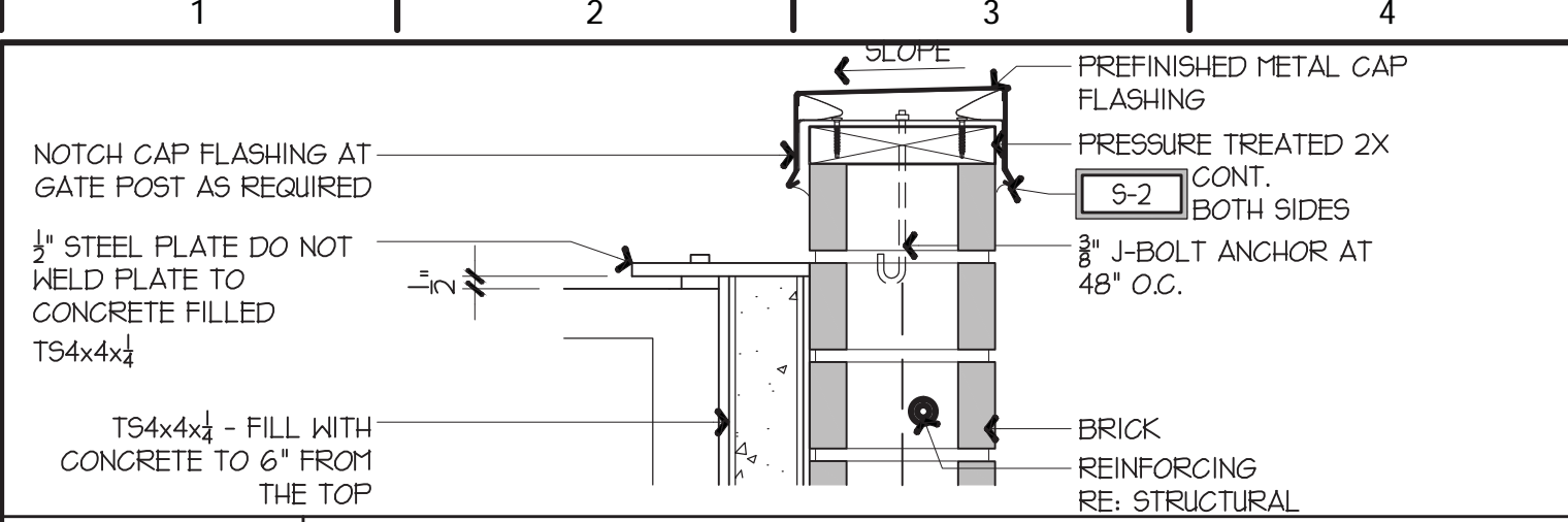
01 FLASHING DETAIL
