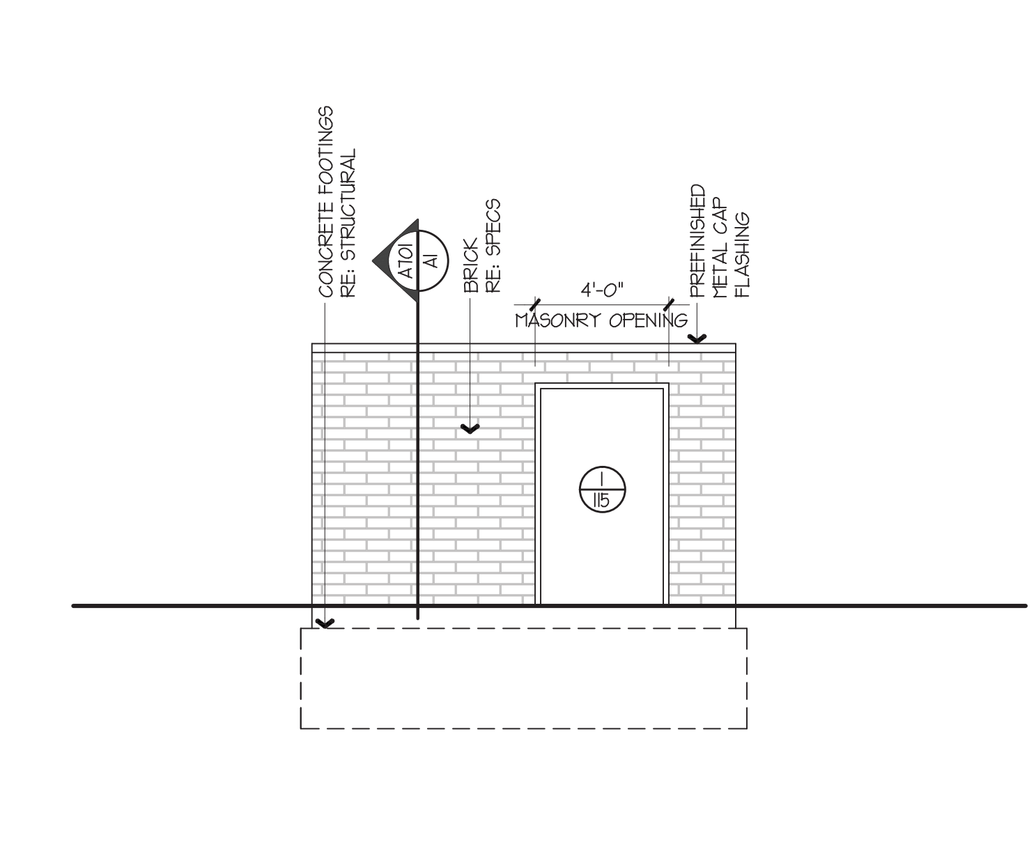
G9 TRASH ENCLOSURE SIDE ELEVATION
