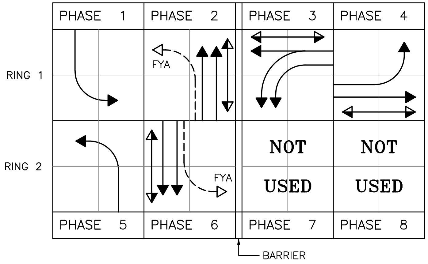
RING STRUCTURE
