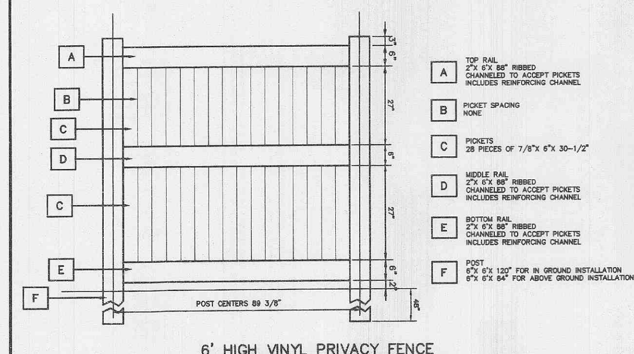
6' HIGH VINYL PRIVACY FENCE NOT TO SCALE
