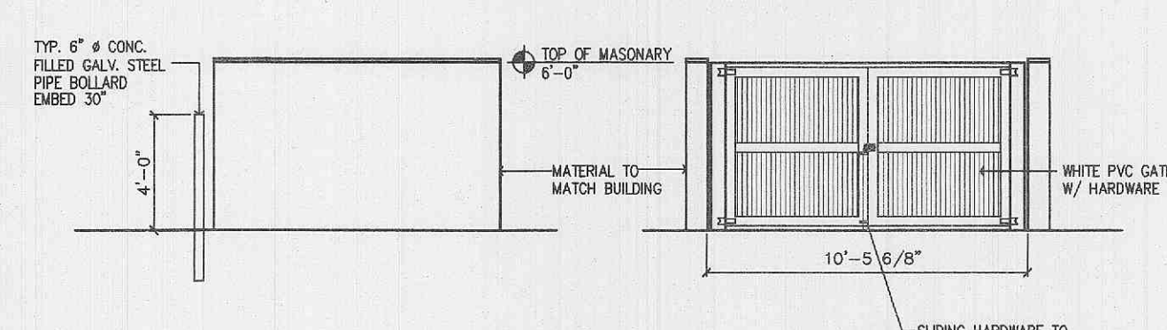
2. ELEVATION NOT TO SCALE
