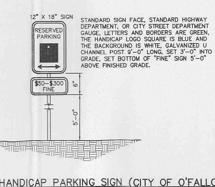
HANDICAP PARKING SIGN (CITY OF O'FALLON) NOT TO SCALE
