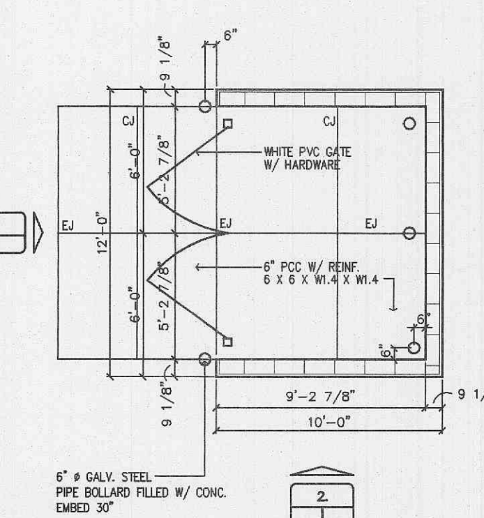
1. TRASH ENCLOSURE PLAN NOT TO SCALE
