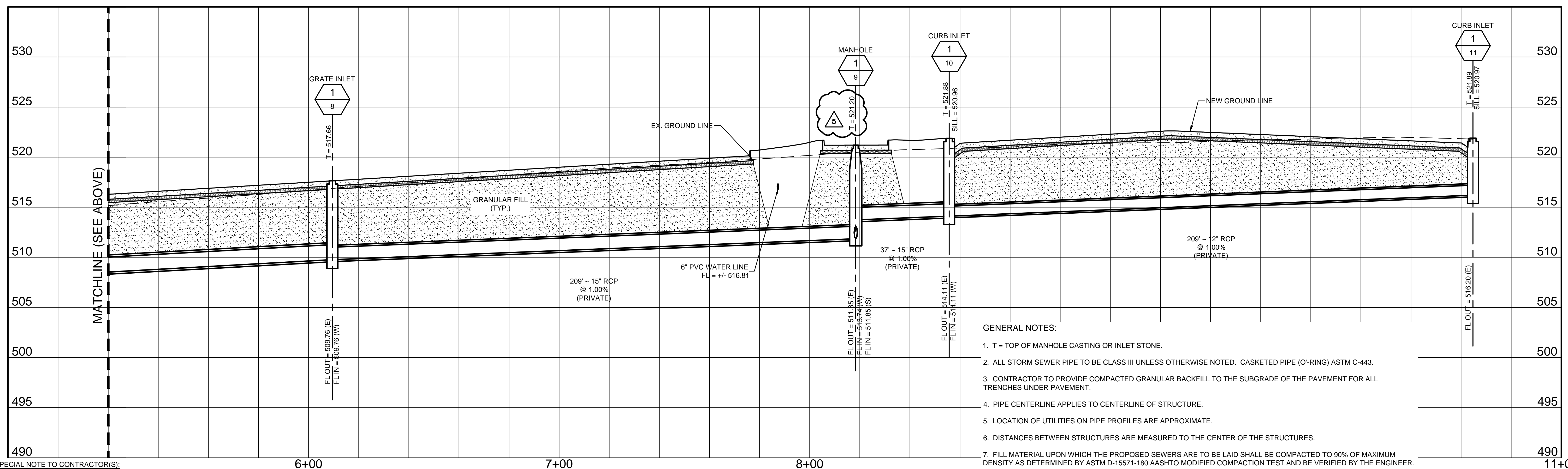
STORM SEWER PROFILES SCALES: 1" = 20' HORIZONTAL 1" = 5' VERTICAL
